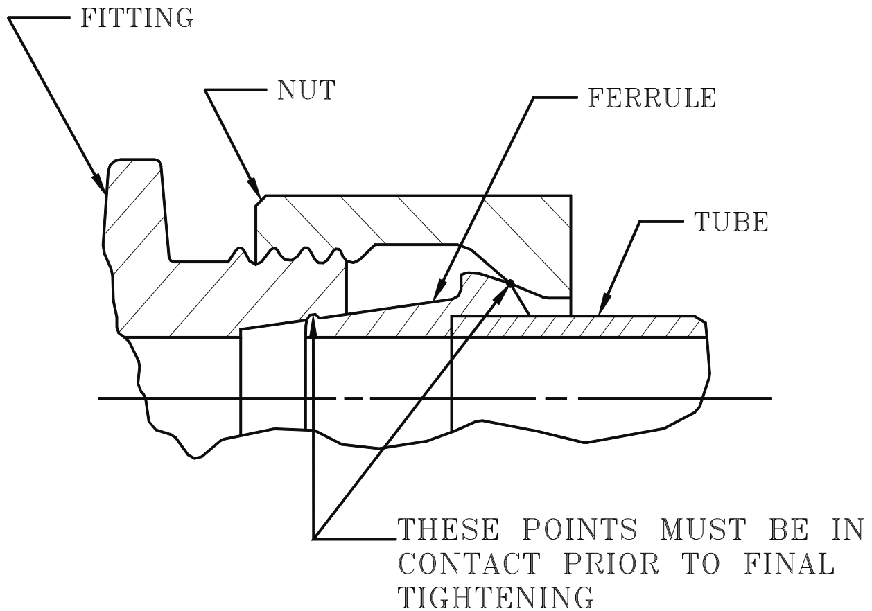
FIGURE 1. Assembly tightening.
