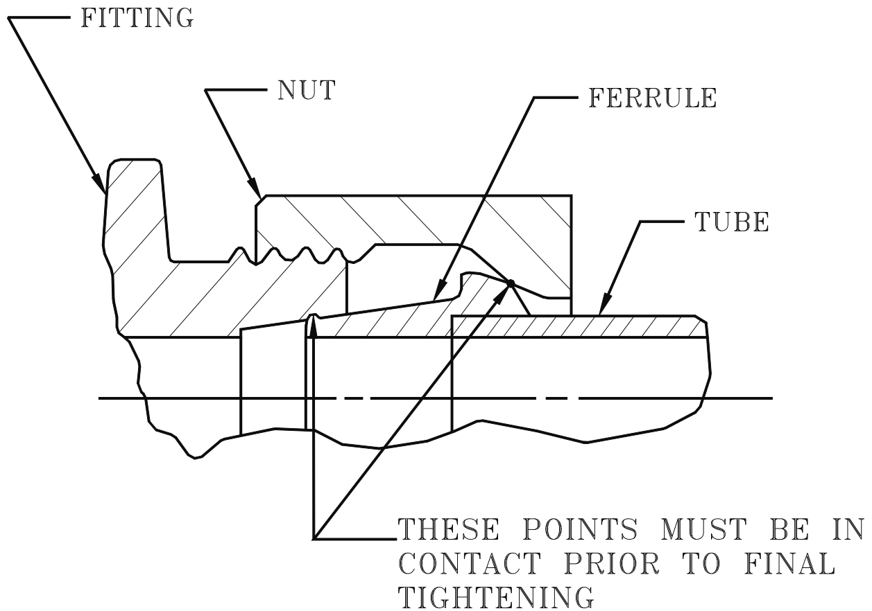
FIGURE 1. Assembly tightening.
