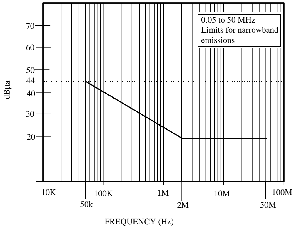
FIGURE 7. Upper limits for conducted narrowband emissions from 0.05 to 50 MHz.
