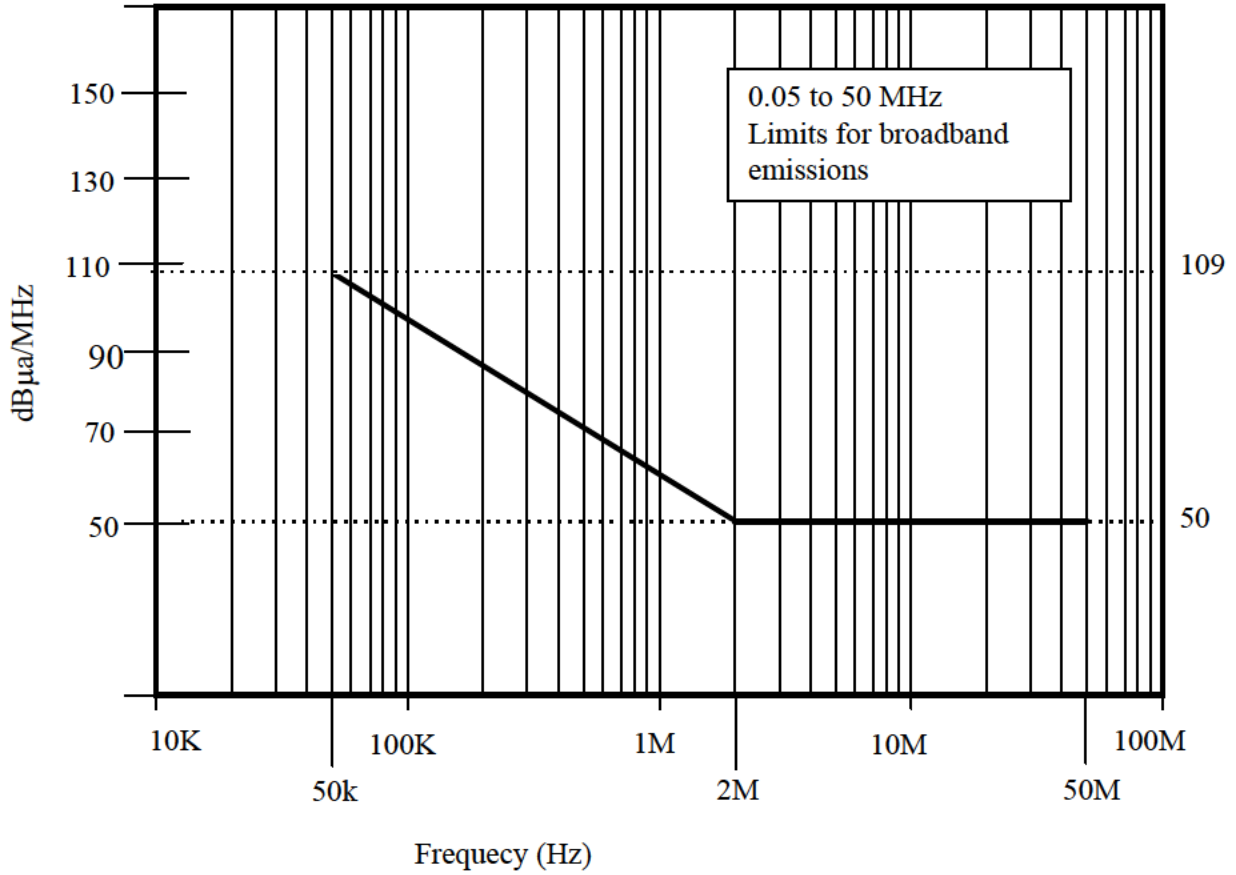
FIGURE 8. Upper limits for conducted broadband emissions from 0.05 MHz to 50 MHz.
