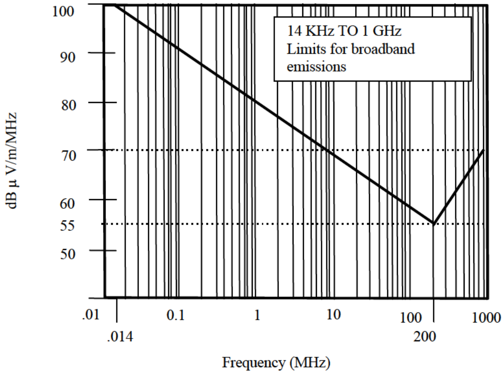
FIGURE 4. Upper limits for radiated broadband emissions.
