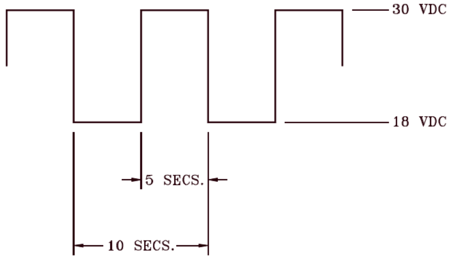
FIGURE 10. Supply voltage characteristics.
