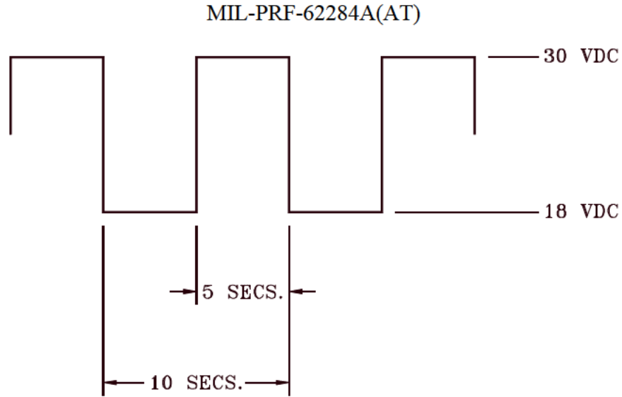
FIGURE 10. Supply voltage characteristics.
