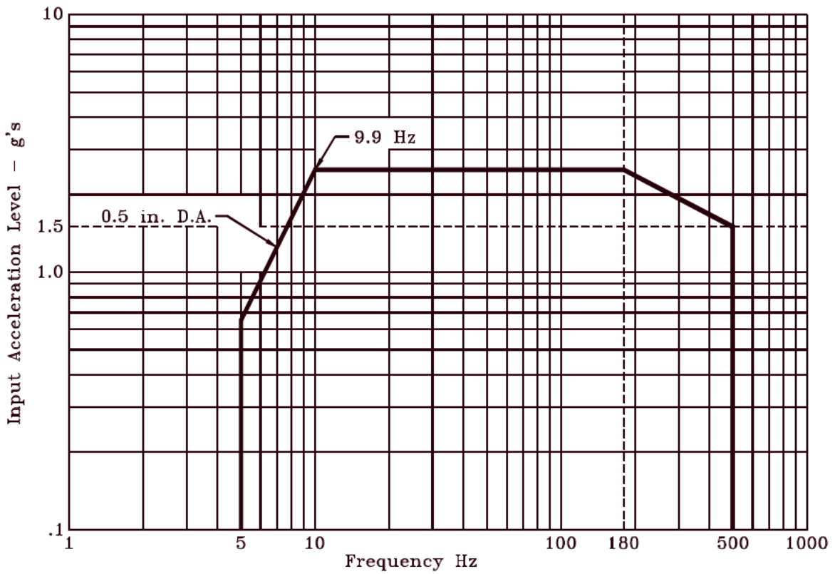
FIGURE 11. Vibration profile.
