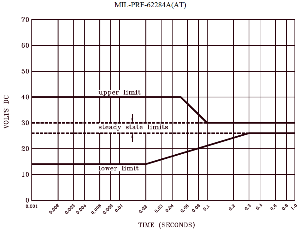
FIGURE 2. Voltage limits loci of surges for fault free operation.
