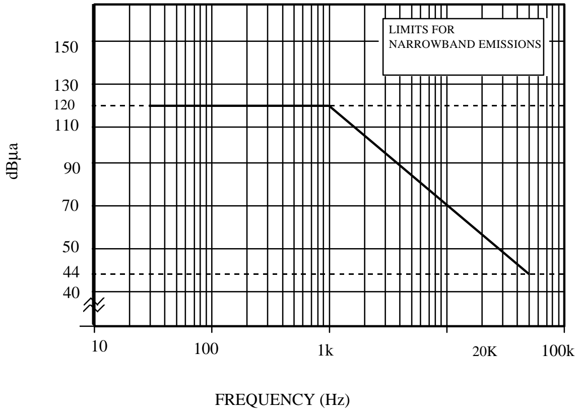
FIGURE 6. Upper limits for conducted narrowband emissions from 30 Hz to 50 KHz.
