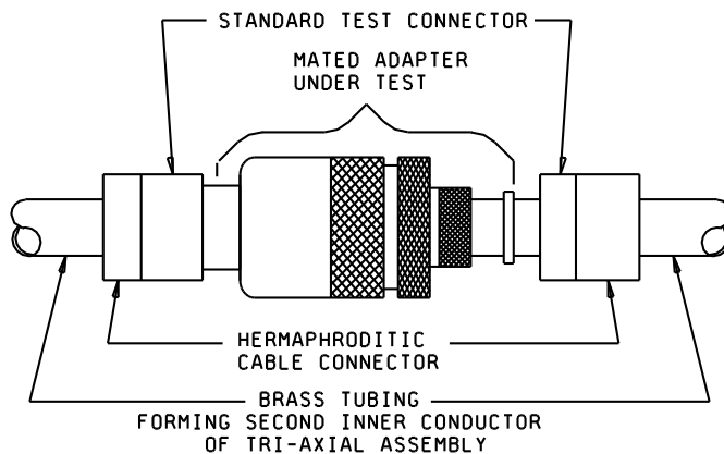
FIGURE 2A. Typical test assembly for RF leakage.
