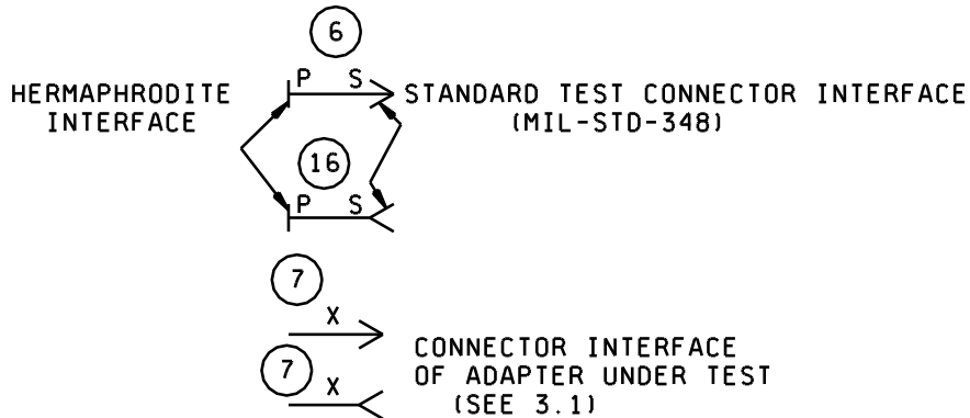
FIGURE 1. Swept frequency VSWR test - Continued.
