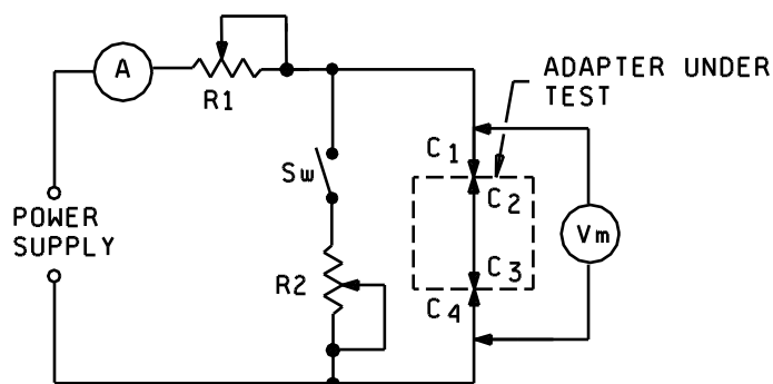
FIGURE 4. Diagram for contact resistance.
