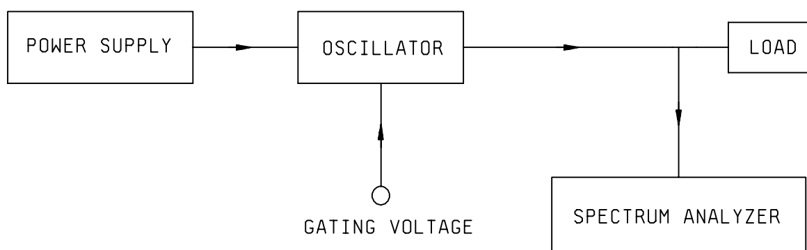
FIGURE 12. Test configuration for determining suppression of gated oscillators.
