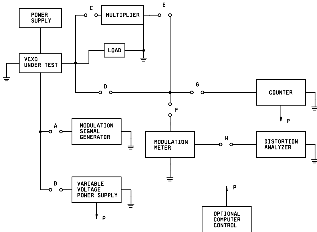
FIGURE 14. VCXO test configurations.
