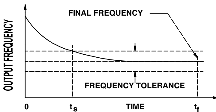
FIGURE 2. Typical oscillator warm-up characteristic.
