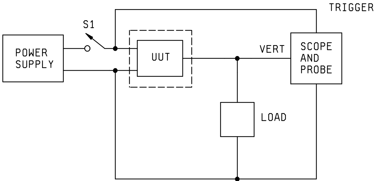
FIGURE 13. Test configuration for startup time measurement.
