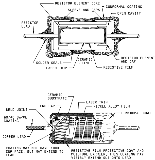
FIGURE 8. Typical hermetically sealed film resistor, RNC style.
