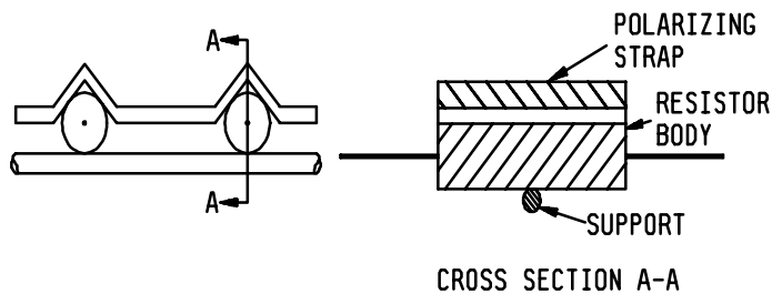
FIGURE 3. Mounting straps for moisture-resistance test.
