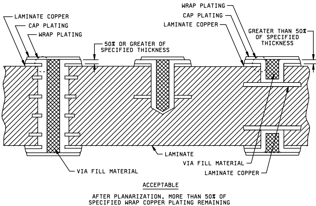
FIGURE G-17. Acceptable planarized plated hole structure wrap copper plating.
