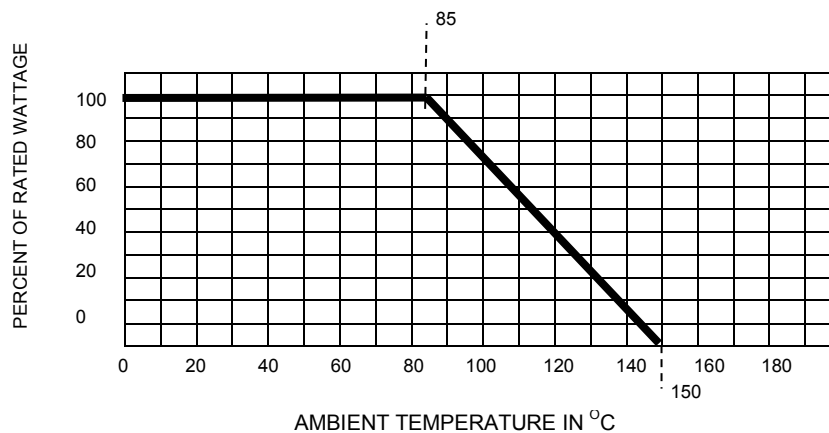
FIGURE 2. Derating curve for high-ambient temperatures .
