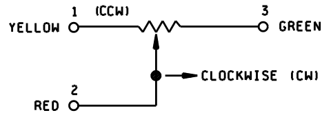
FIGURE 1. Circuit diagram
