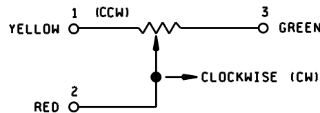
FIGURE 1. Circuit diagram
