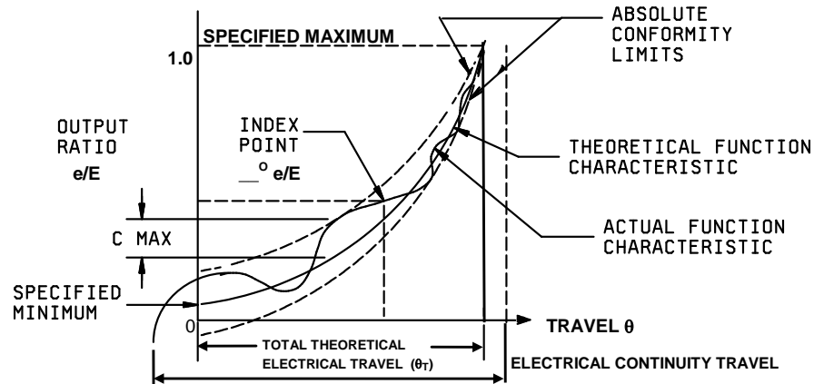
FIGURE 17. Absolute conformity.
