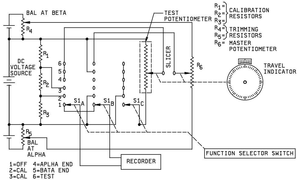
FIGURE B-I. Conformity tester.
