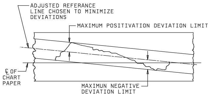
FIGURE B-II. Determination of independent linearity.
