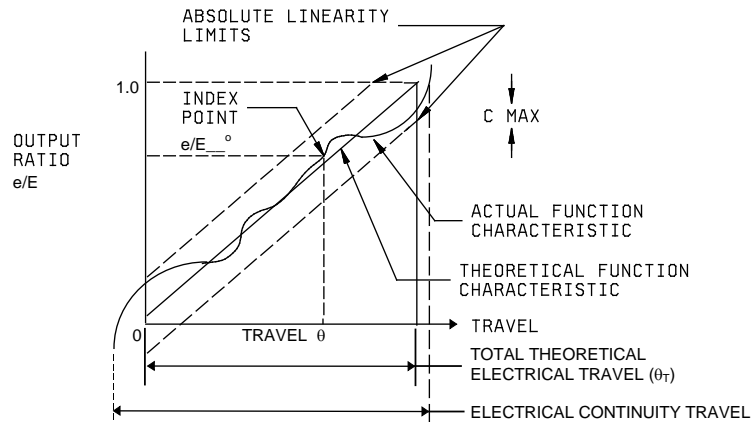
FIGURE 18. Absolute linearity.
