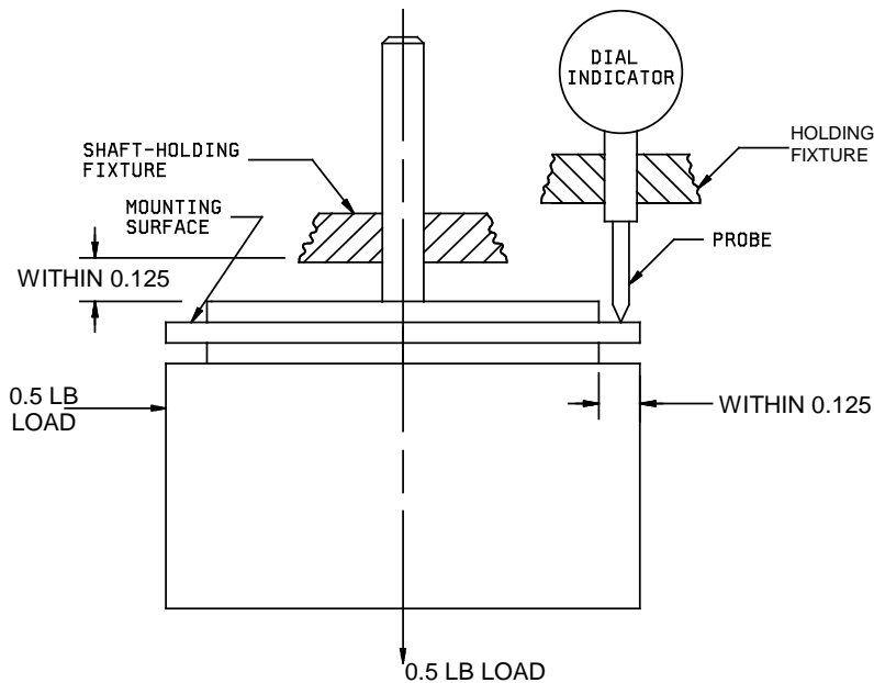
FIGURE 1. Measurement of lateral runout
