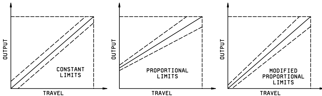
FIGURE 20. Tolerance limits.
