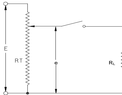
FIGURE 13. Loading error.
