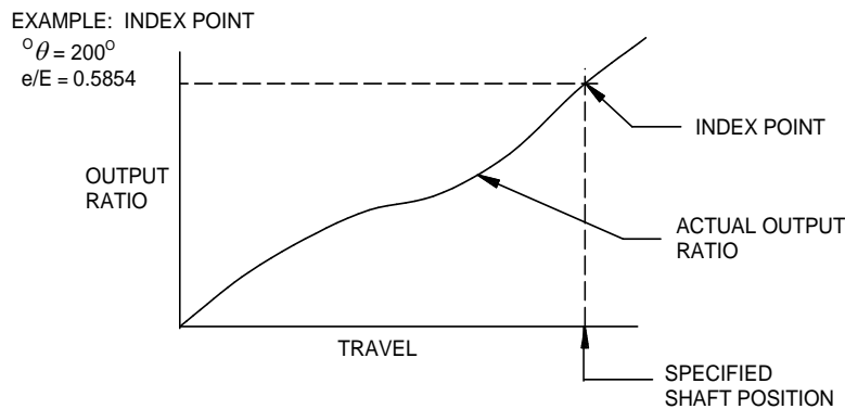
FIGURE 16. Index point.
