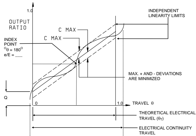
FIGURE 19. Independent linearity.
