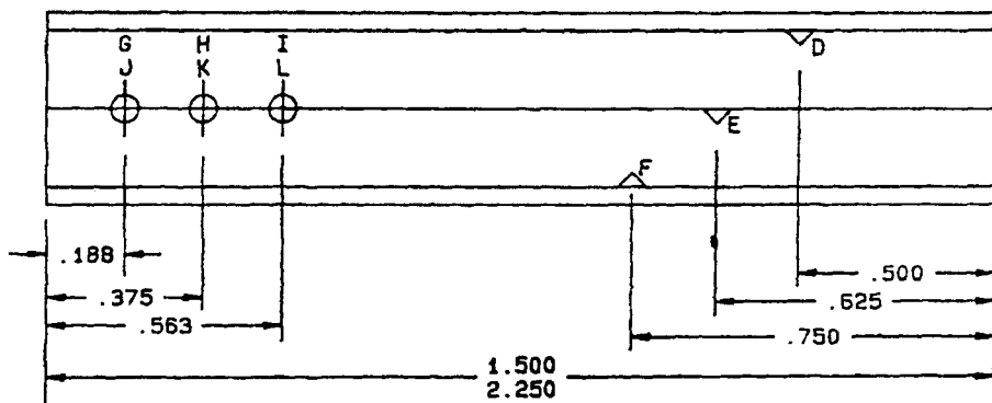
VIEW B
