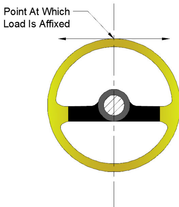
Figure 6, Torsion durability.
