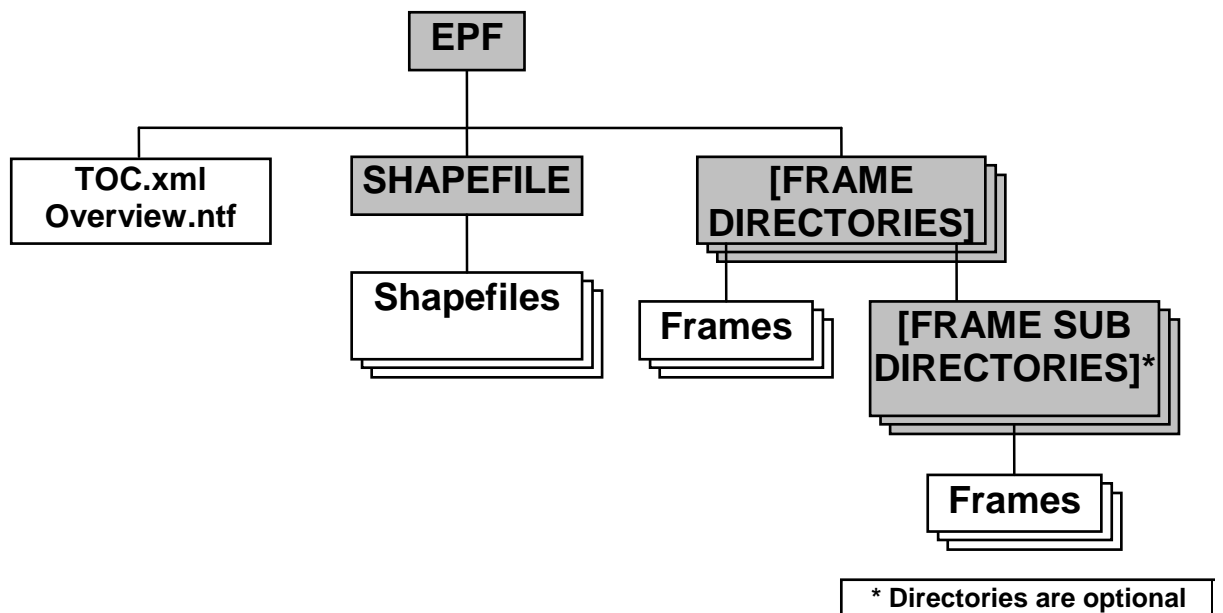
FIGURE 2. Pictorial representation of ECIB directory and file structure
