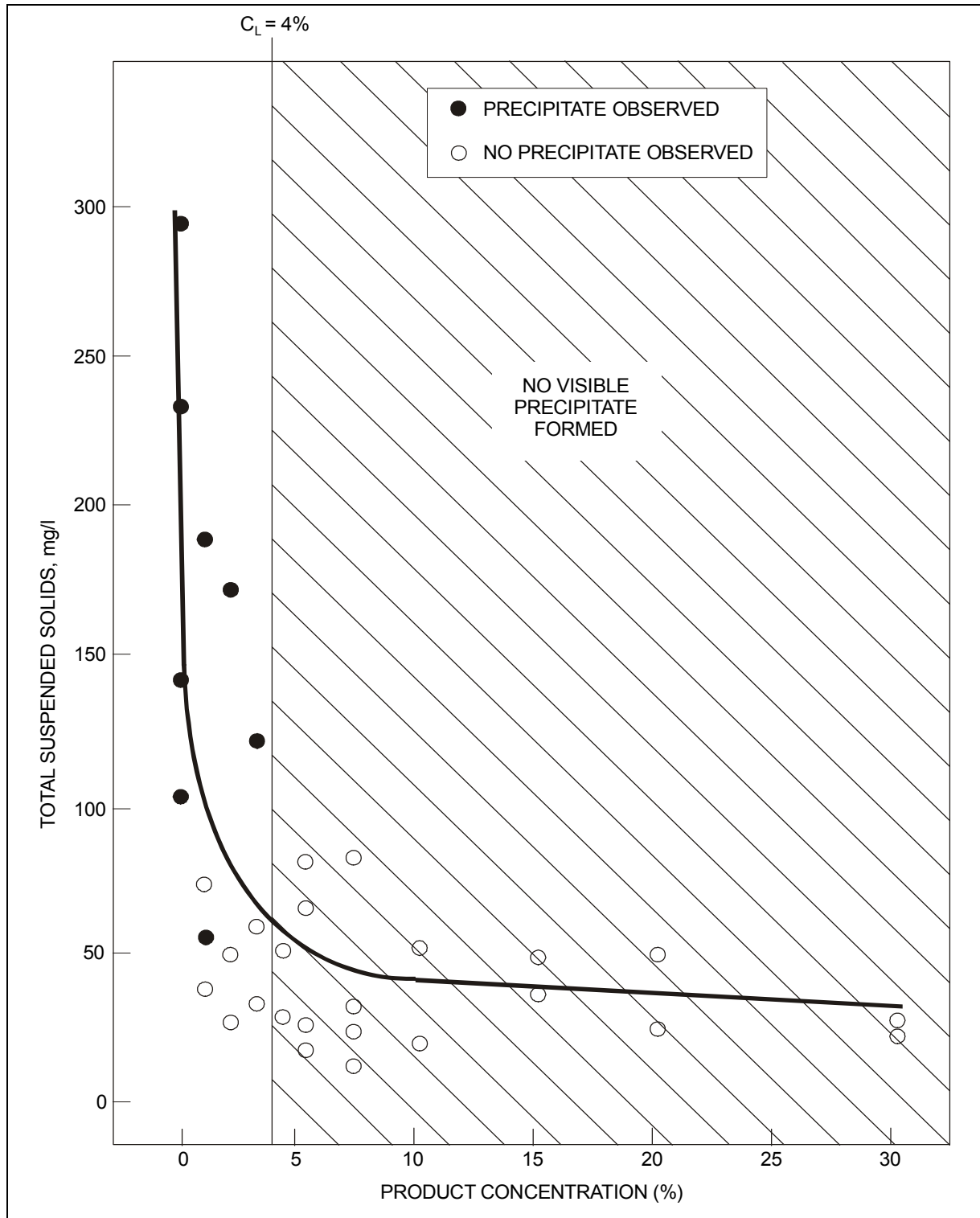
FIGURE 2. Sample static scale precipitation test curve.
