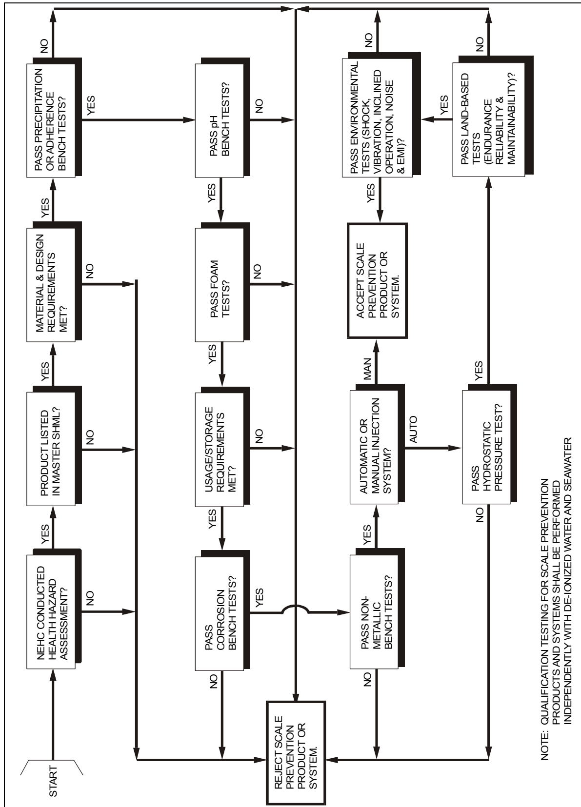
FIGURE 1. Sequence of scale prevention products and systems qualification.
