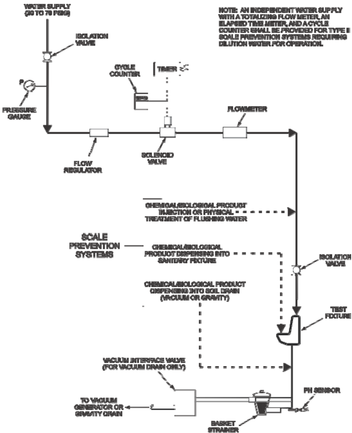
FIGURE 3. Endurance test apparatus set-up.
