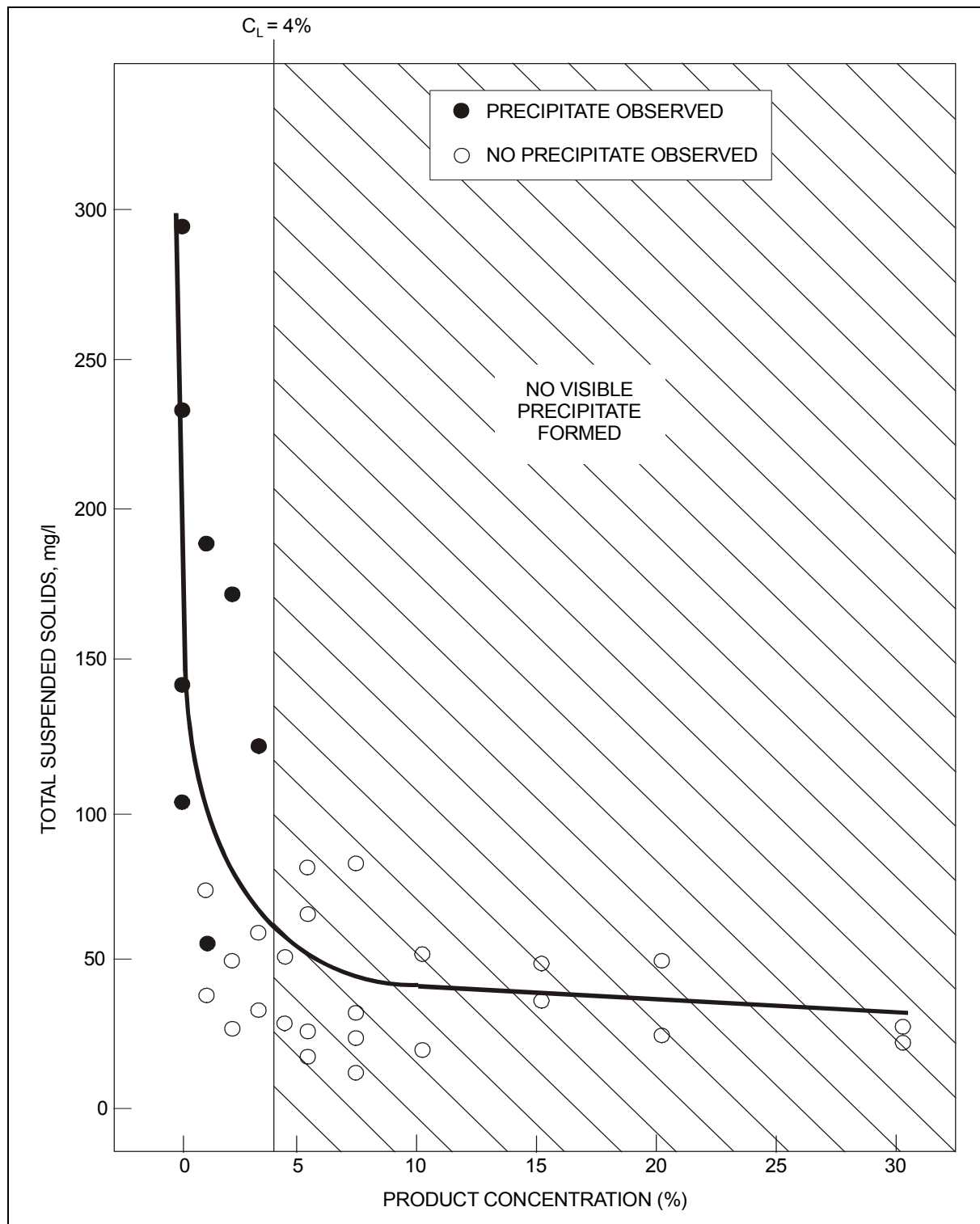
FIGURE 2. Sample static scale precipitation test curve.
