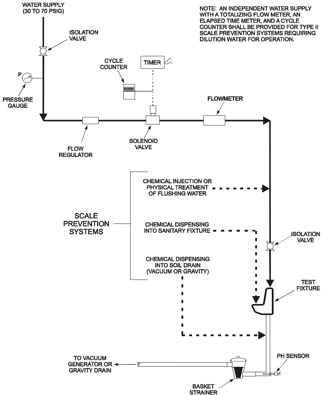
FIGURE 3. Endurance test apparatus set-up.
