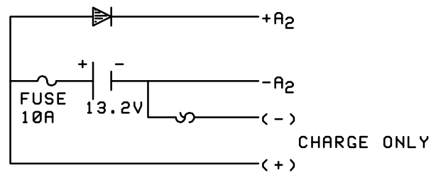
FIGURE 3. WIRING SCHEMATIC.
