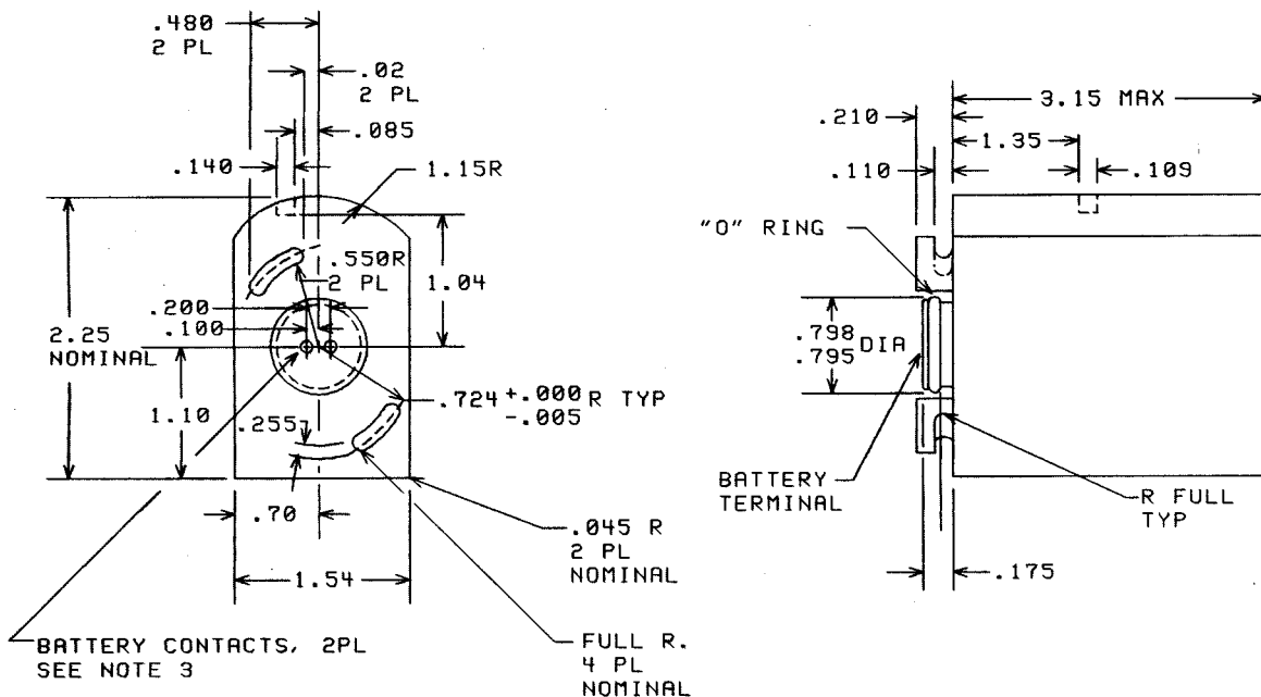
Figure 1. Battery dimensions.
