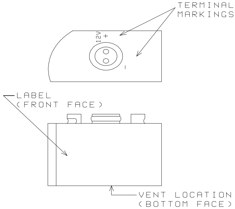
Figure 2. Terminal markings.
