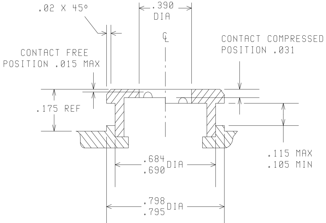
Figure 3. Contact Configuration.
