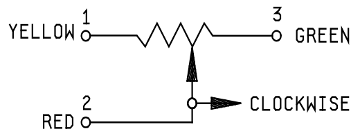
FIGURE 1. Circuit diagram .
