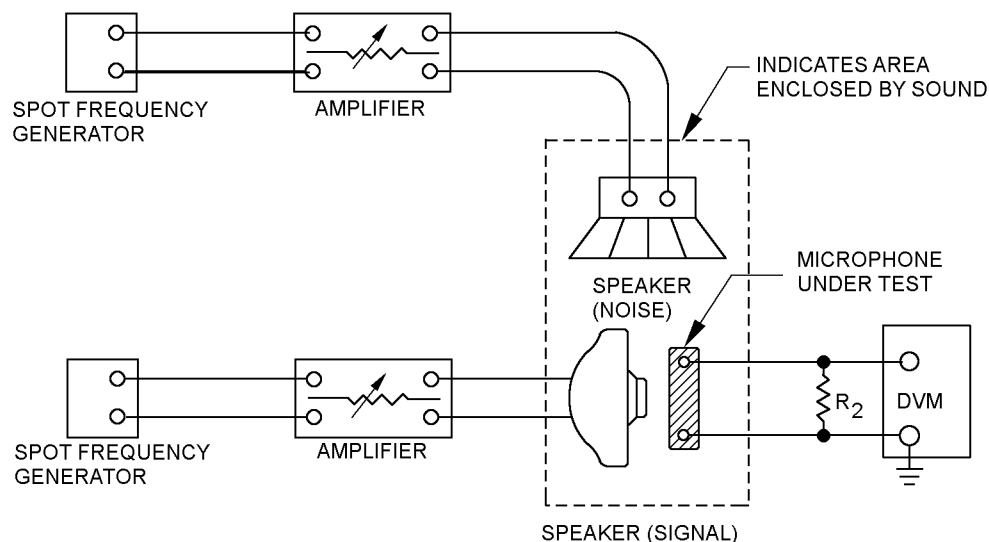
FIGURE 2. Signal-to-noise apparatus setup.
