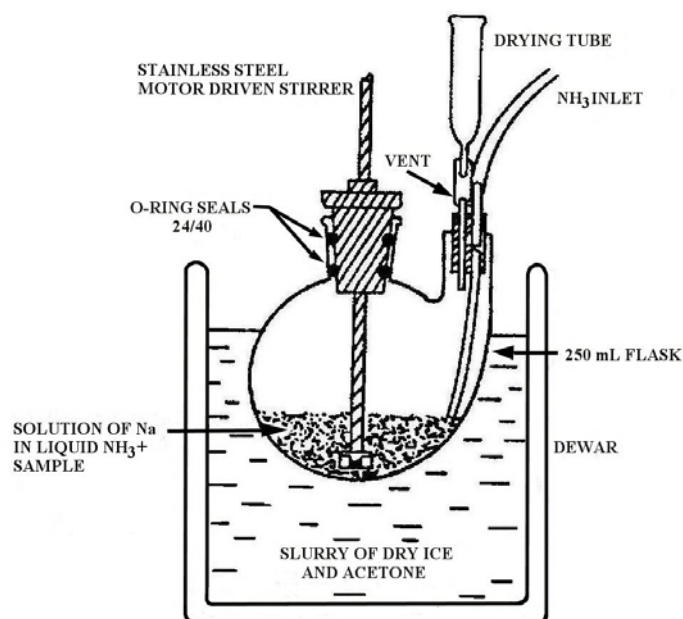
FIGURE 1. Apparatus for the decomposition of organic halides.
