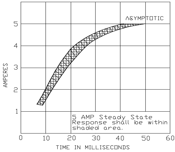
FIGURE 6. Response (current versus time) type I inductors only.
