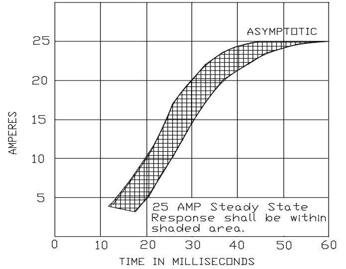
FIGURE 6. Response (current versus time) type I inductors only.
