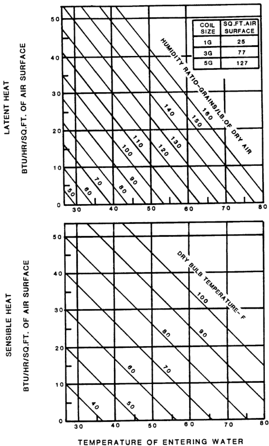
FIGURE 6. Gravity coil performance range.
