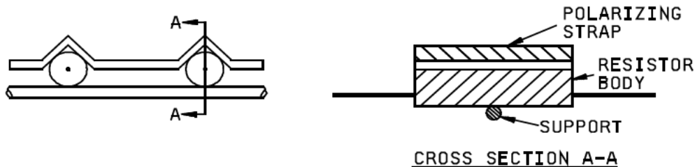
FIGURE 2. Mounting straps for moisture-resistance test.
