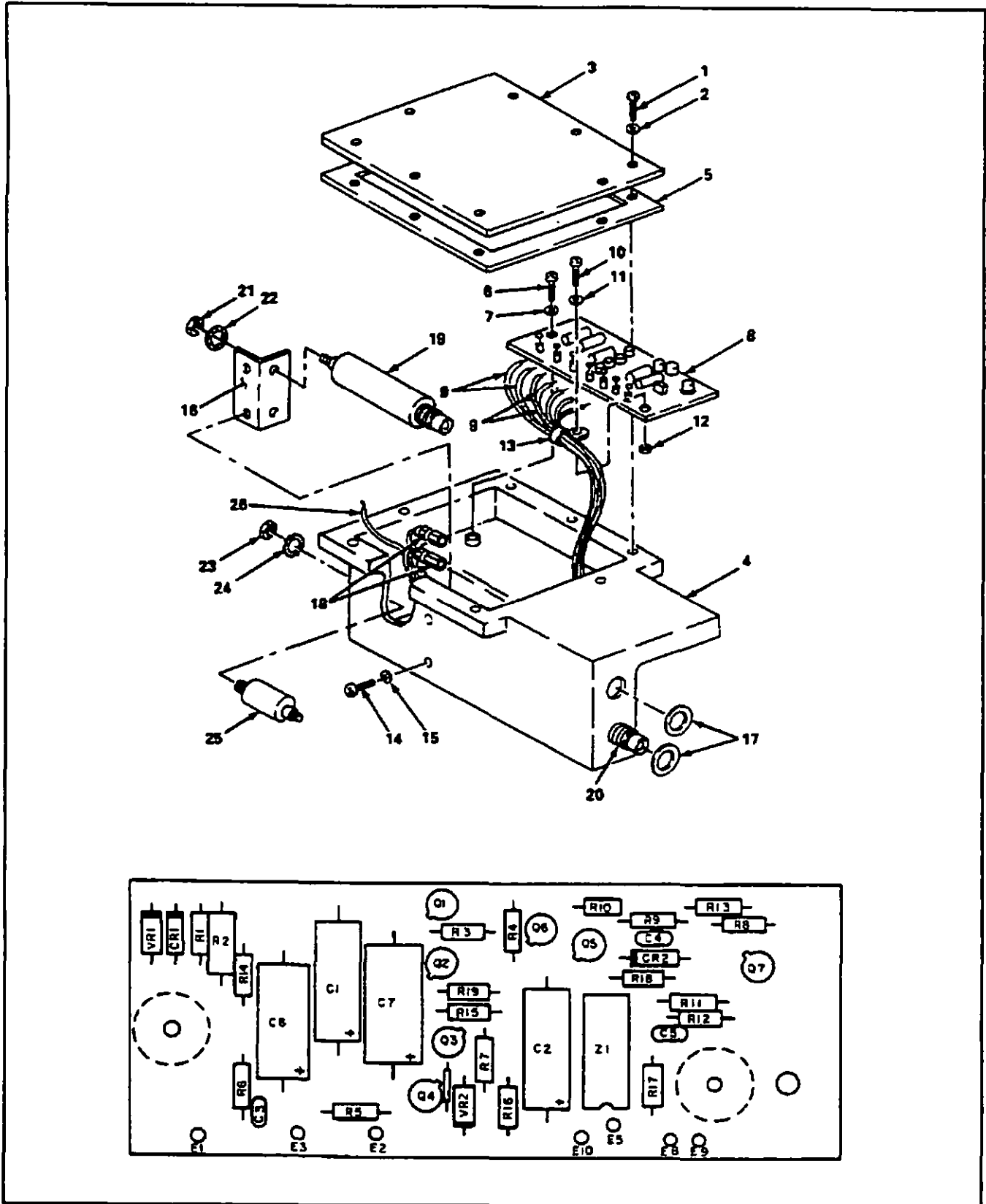
FIGURE 49. Example of an electronic component card illustration.
