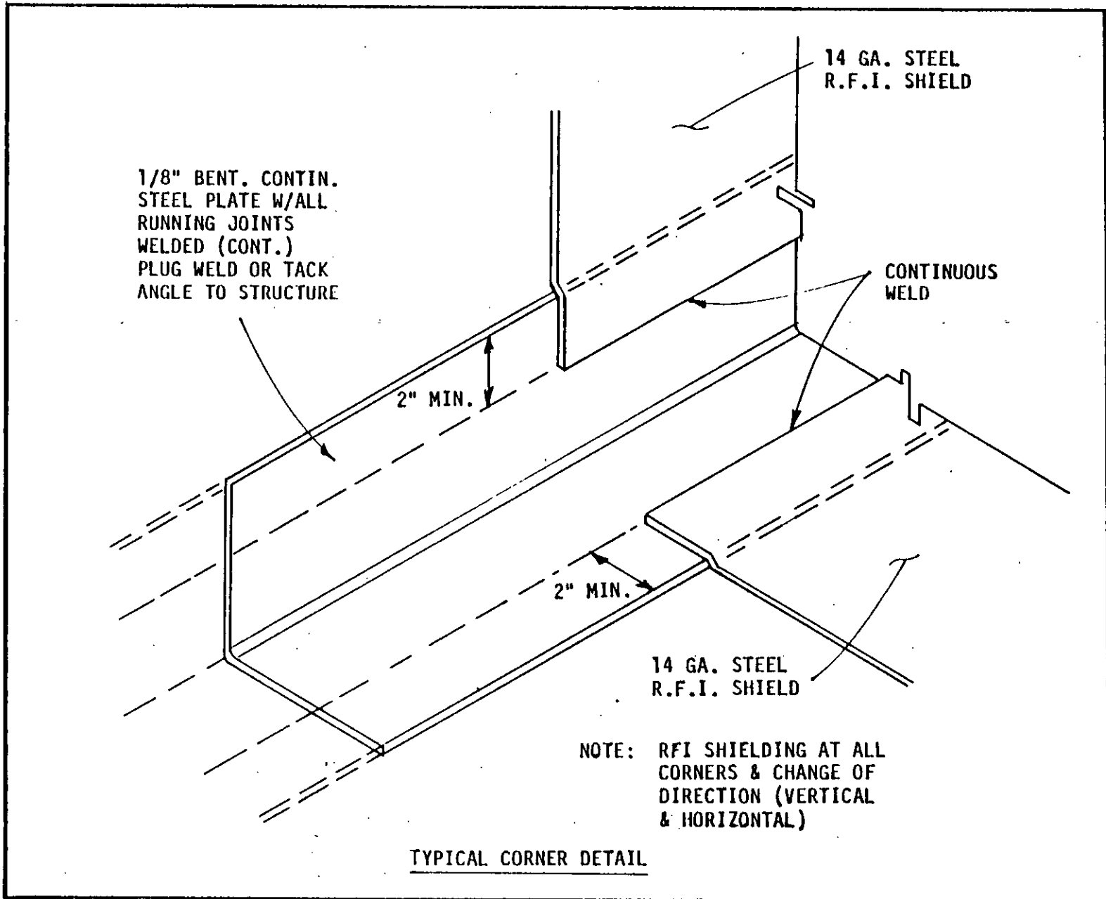
RF Shielding of Floor-wall Intersection with Overlap Seams Figure 23
