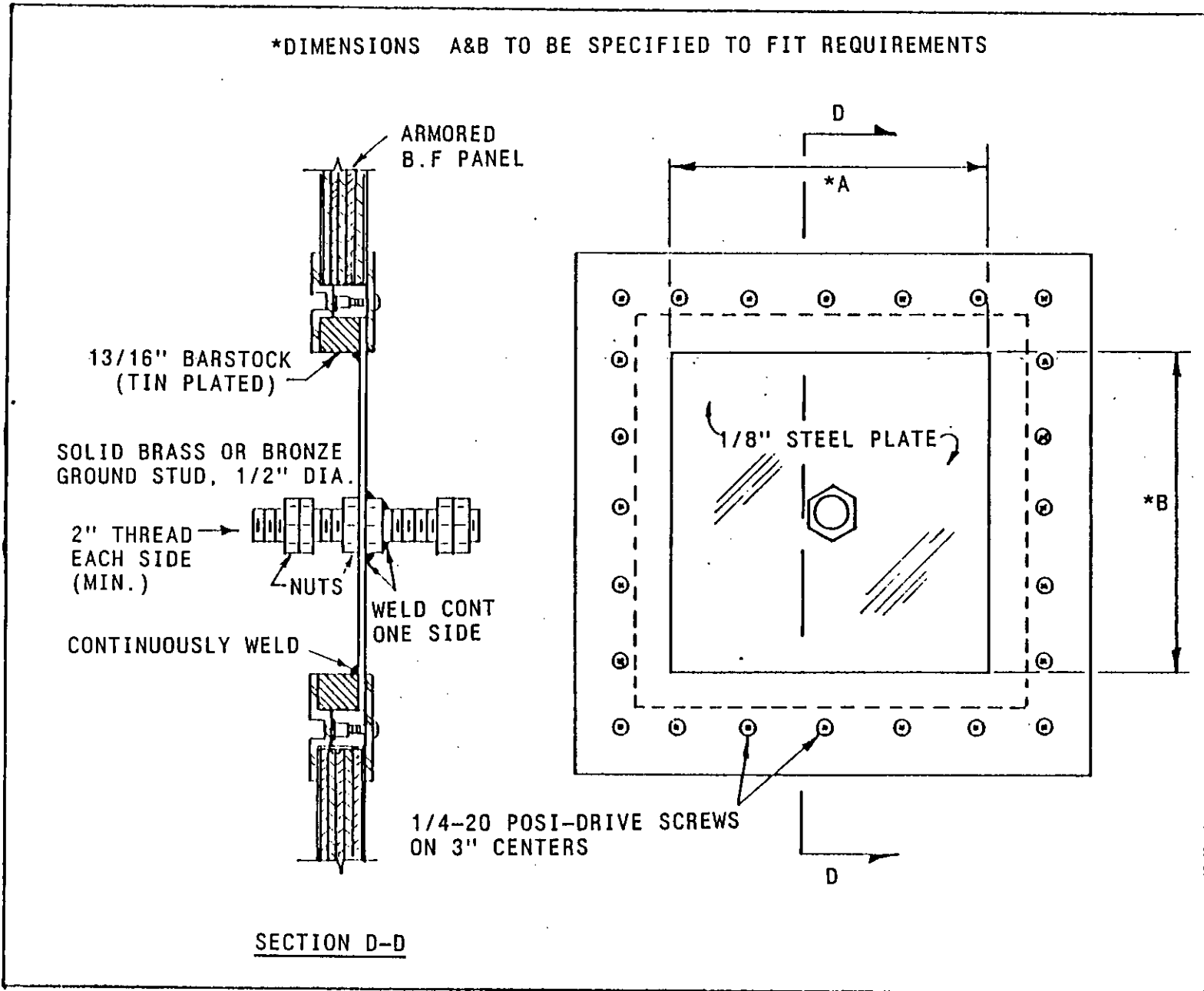
Single Entry Ground Stud Penetration in a Bolted Plate Assembly Figure 14
