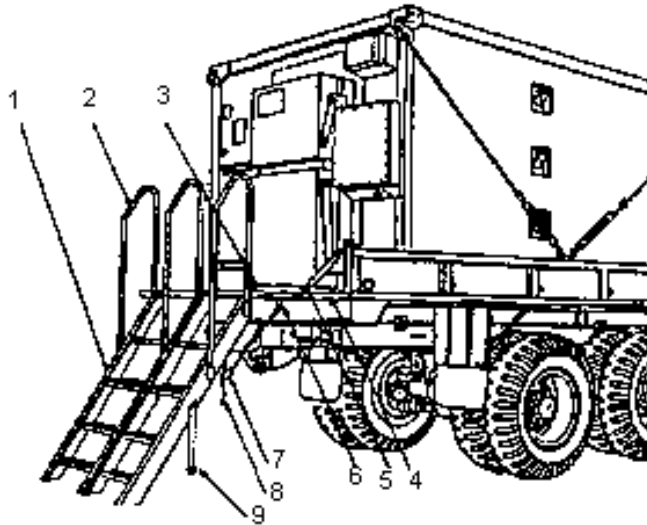
Figure 1. Ladder Installation
