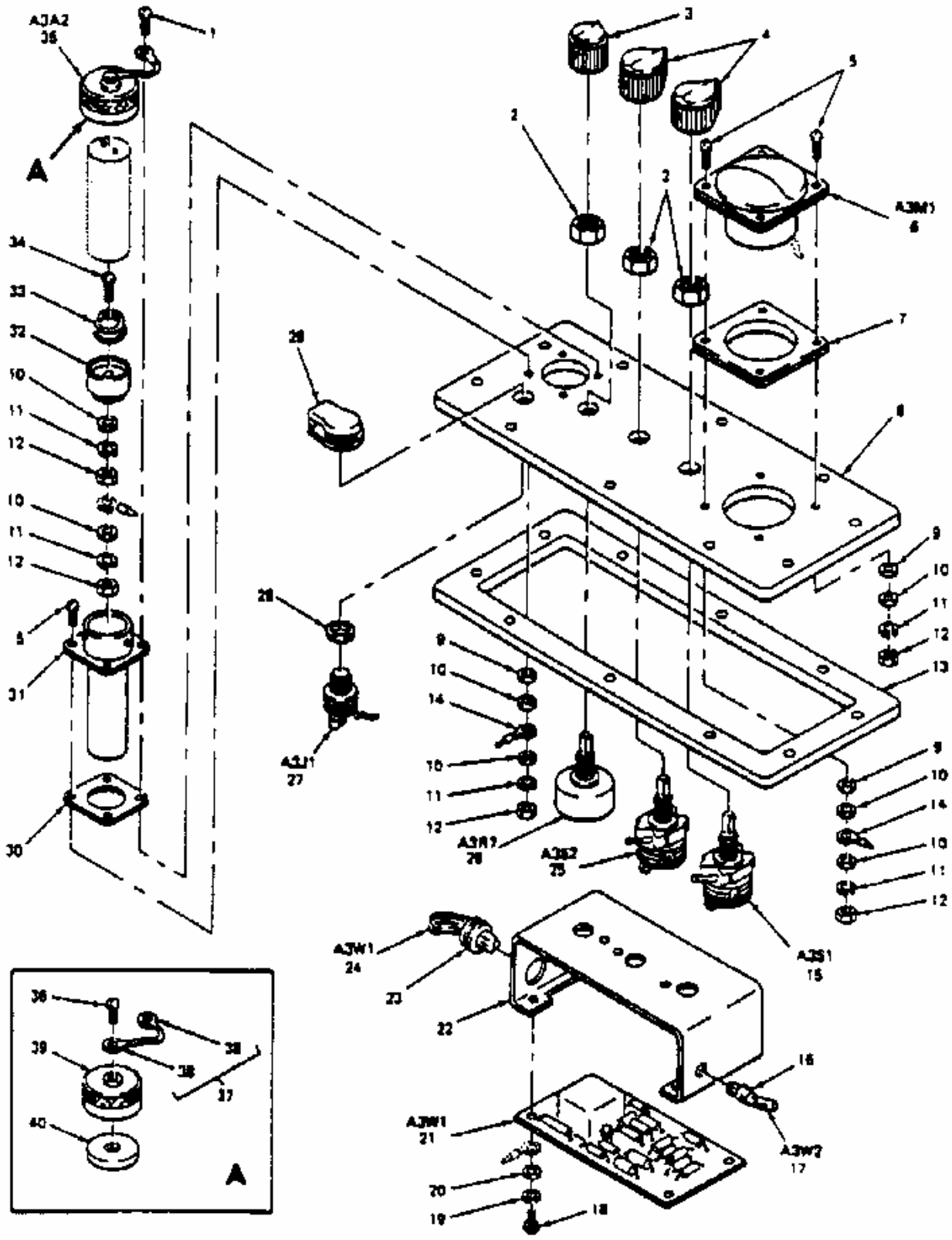
Figure 41. Example of an electronic equipment RPSTL illustration.
