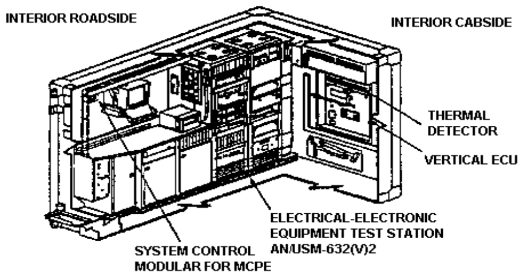
Figure 2. Interior Components
