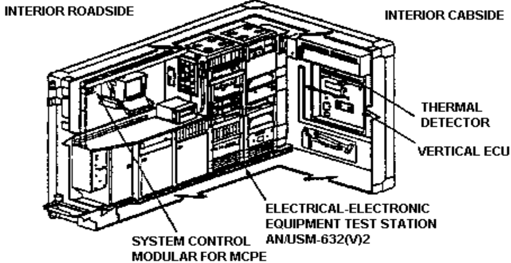
Figure 2. Interior Components
