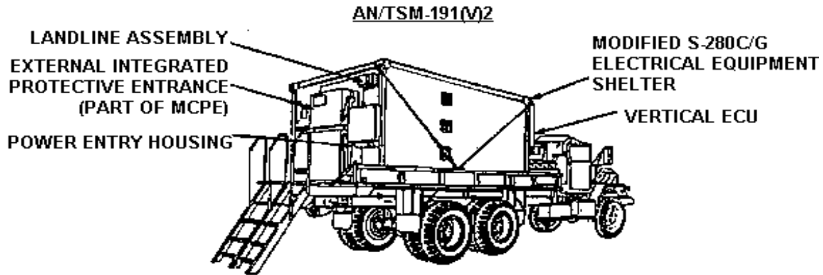
Figure 1. Exterior Components
