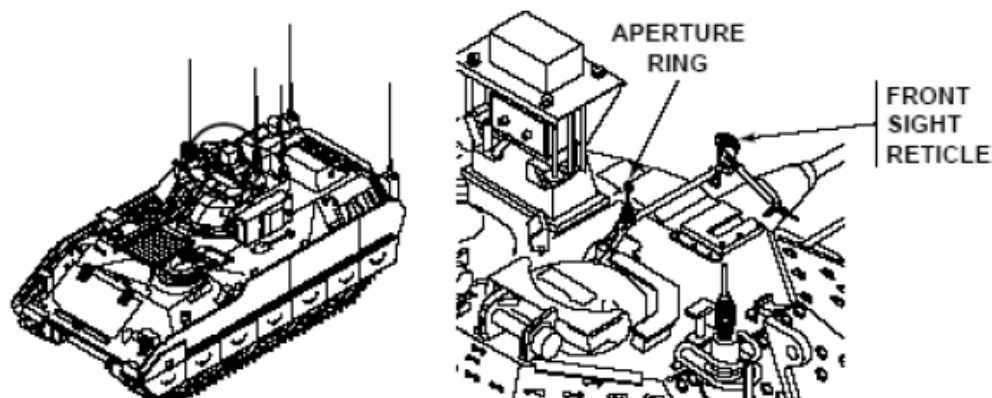
Figure 1. Aperture Ring
