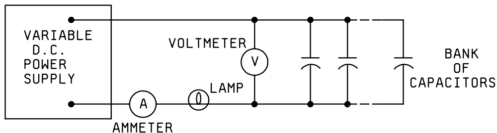
FIGURE 1. Schematic diagram.
