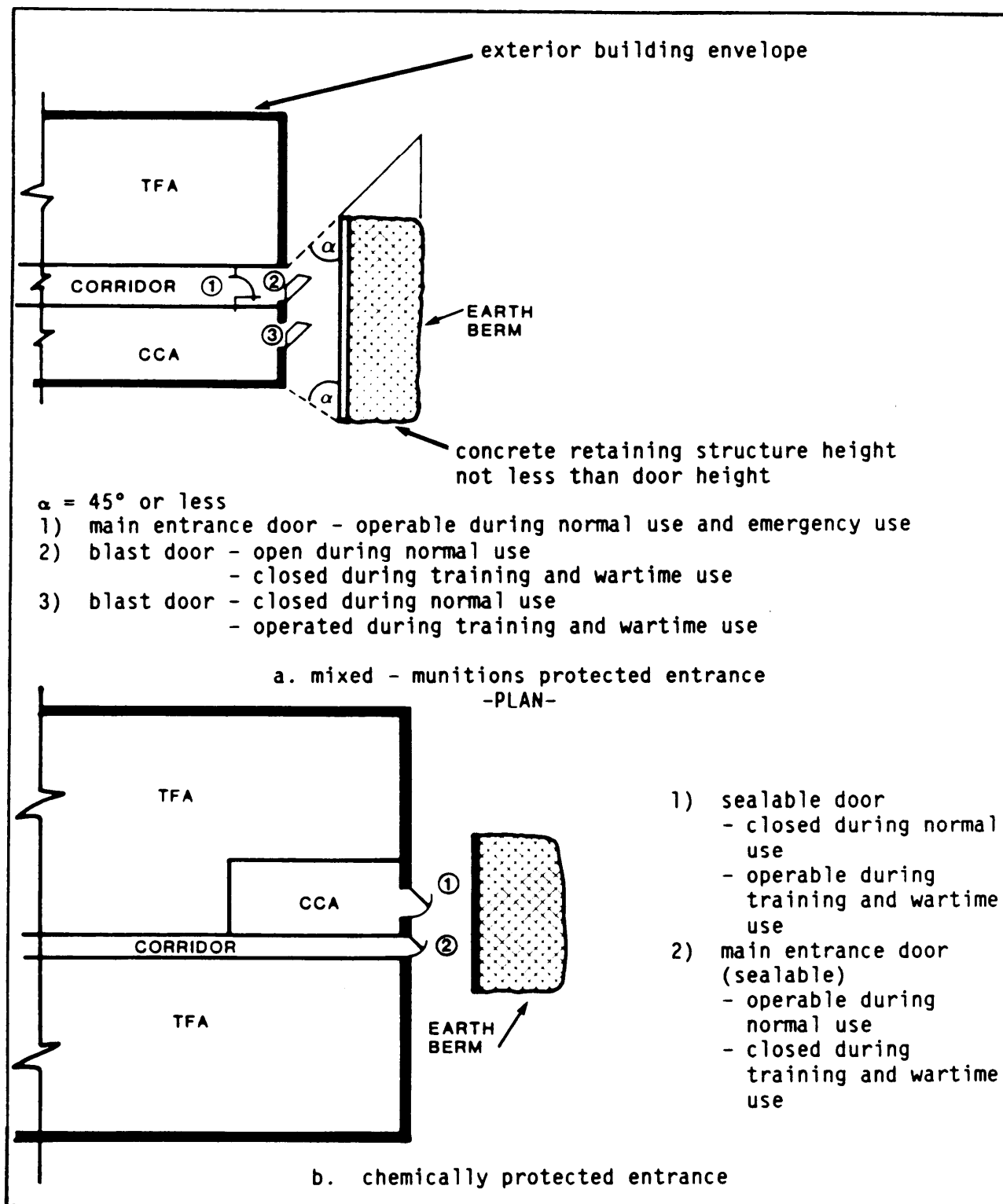
Figure 2 Entrance Arrangements
