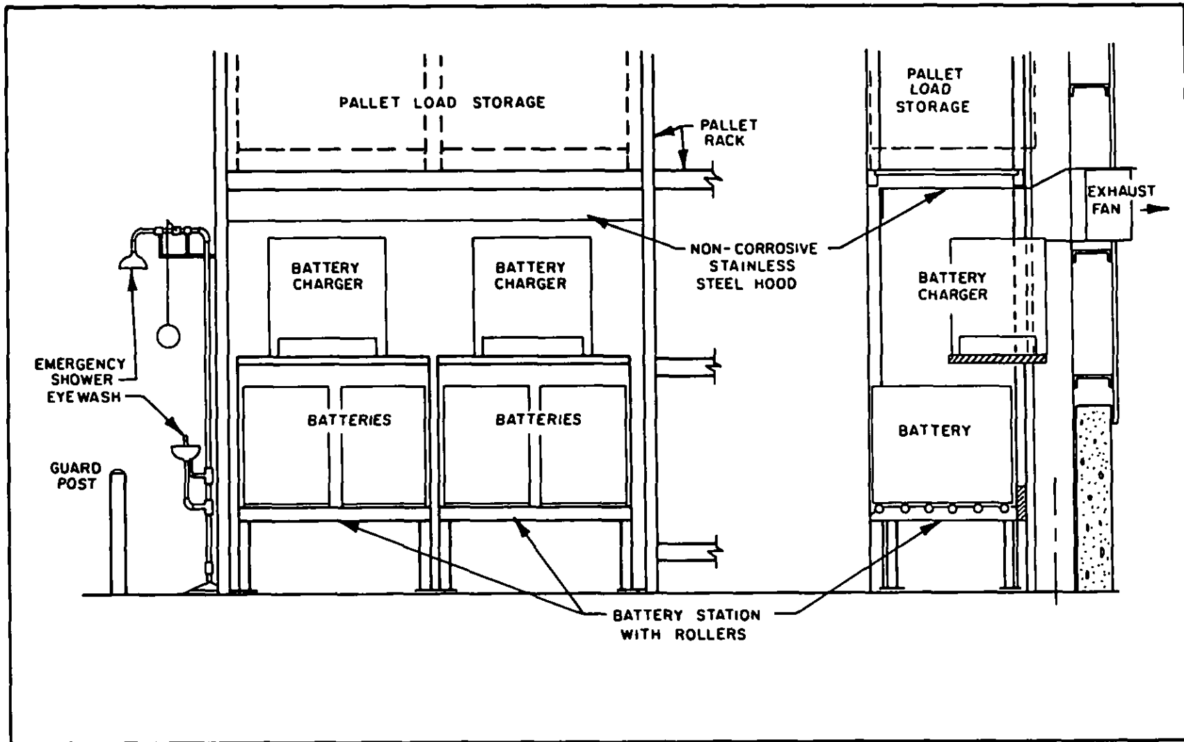
Figure 24 Typical Battery Charger Installation (With Eye Wash/Shower)
