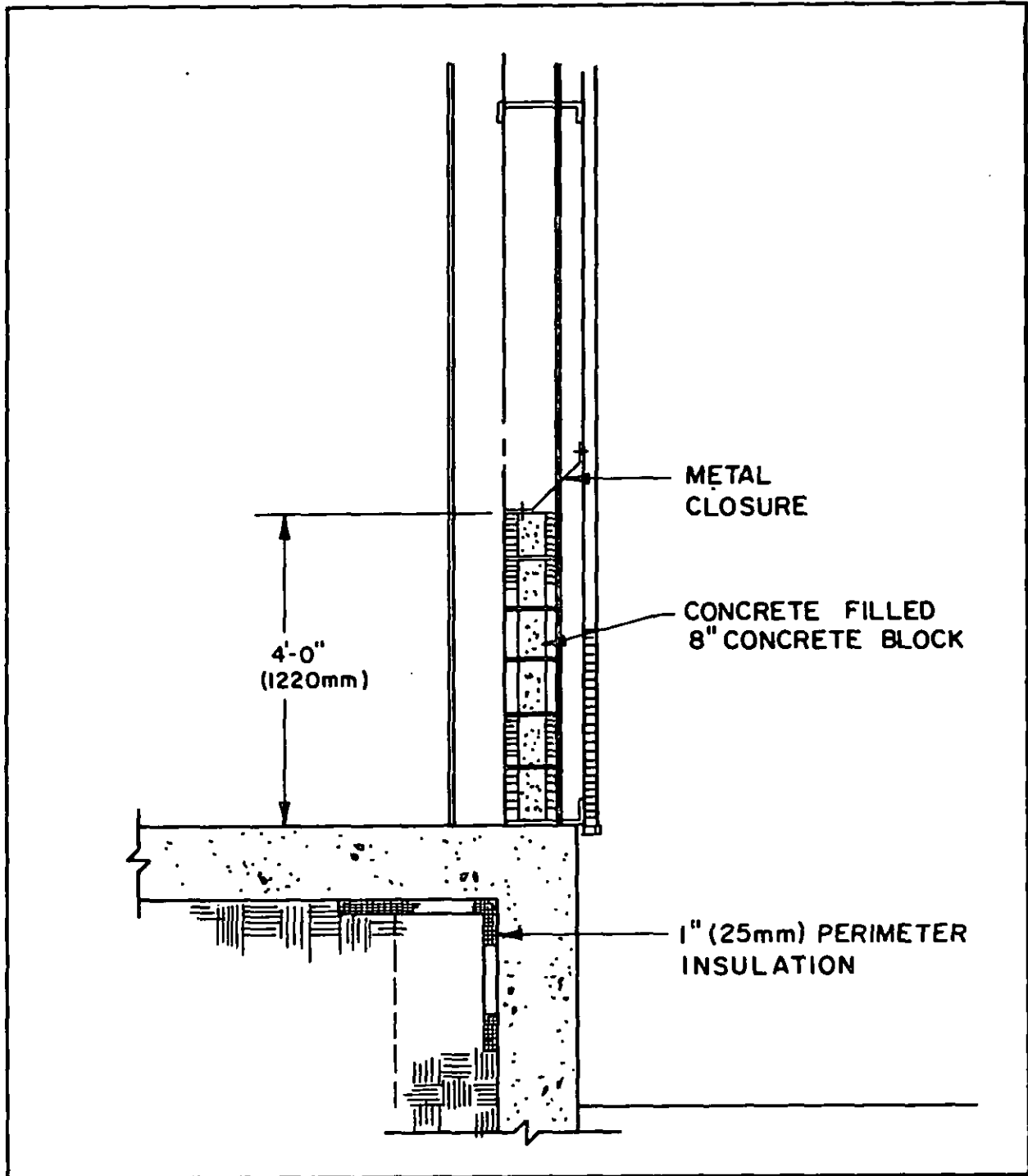
Figure 17 Exterior Wall Detail
