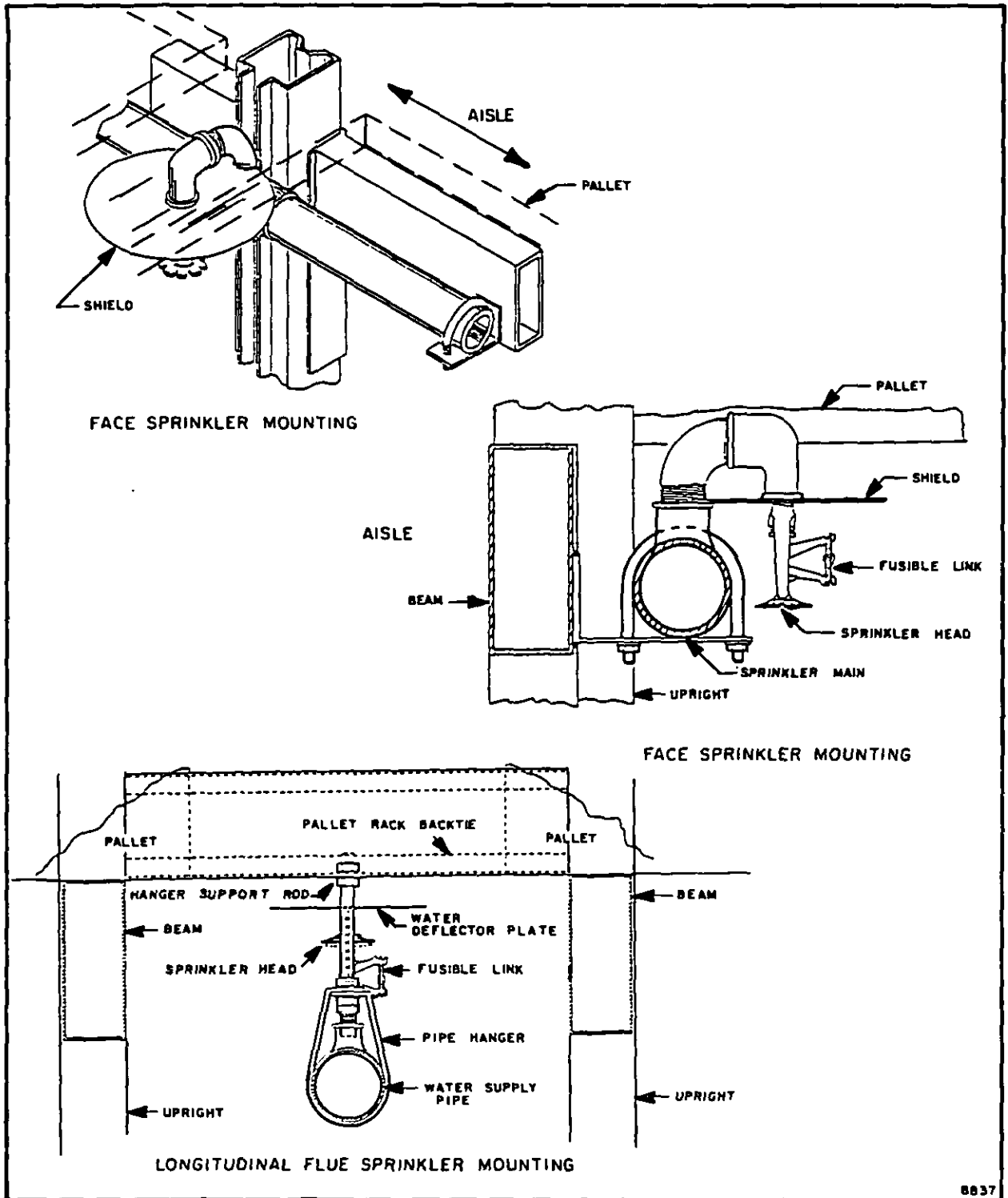
Figure 20 Standard Navy Face and Longitudinal Flue Sprinkler Mounting (to Prevent Pallet and Load Interference)
