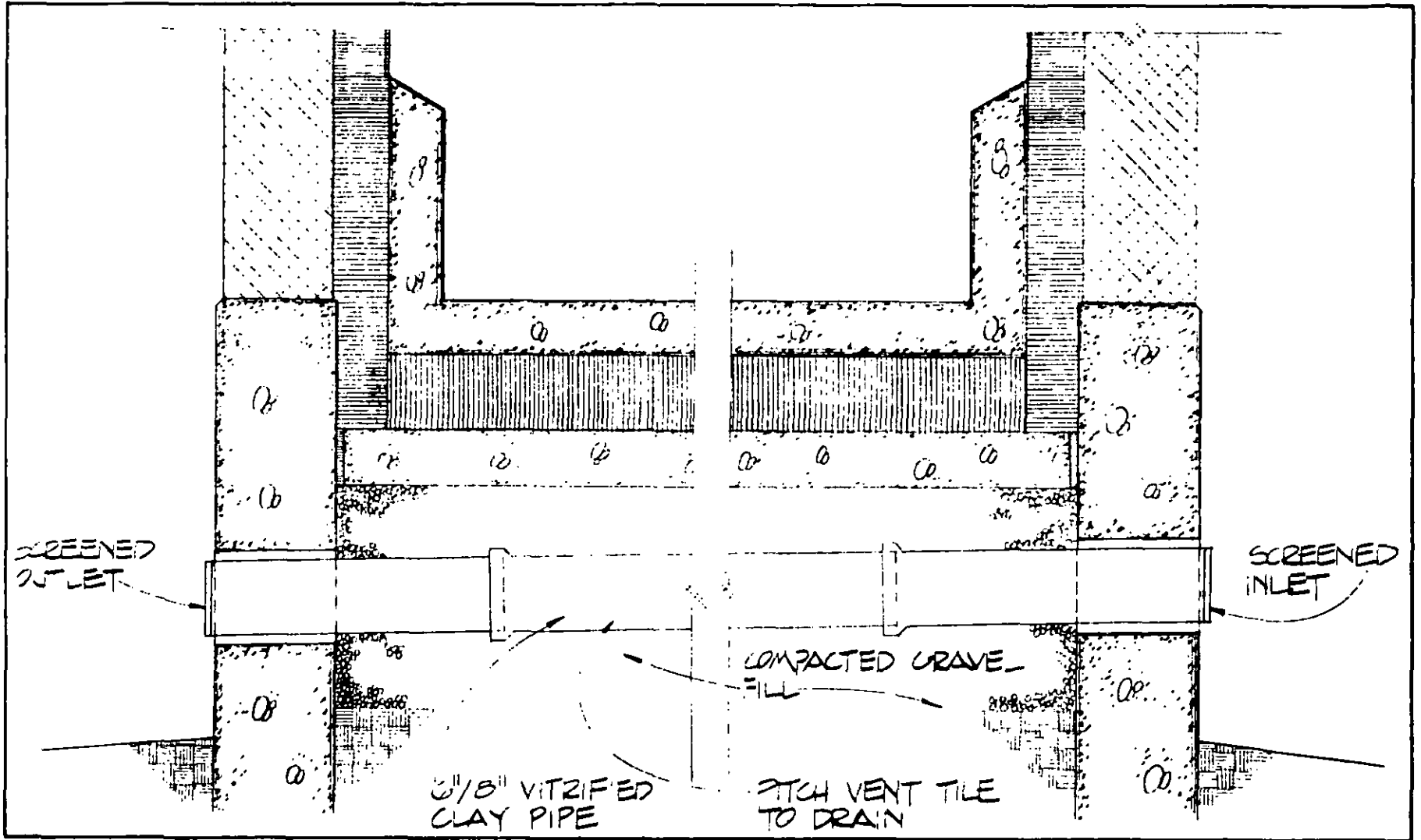
Figure A-13 Typical Underfloor Air Duct Heat System For Slab On Ground Freezers
