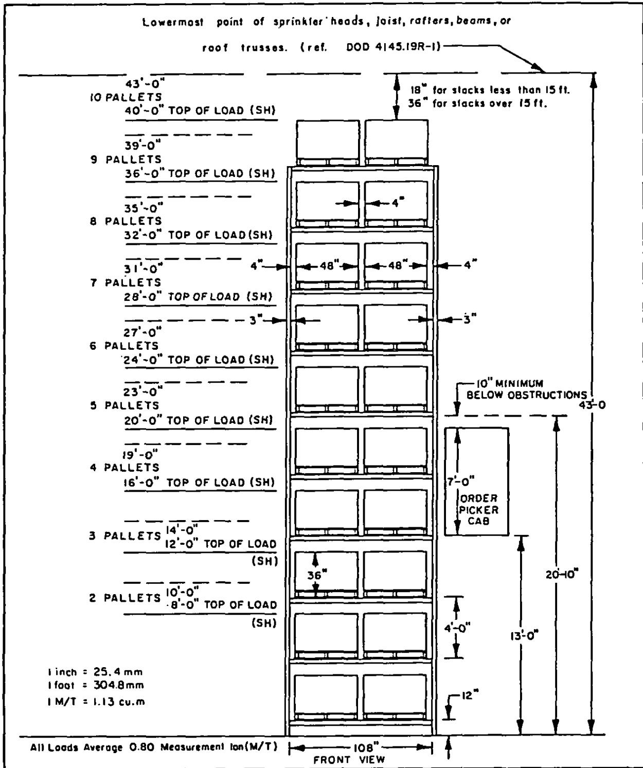
Figure 27 Standard Pallet Rack Elevation
