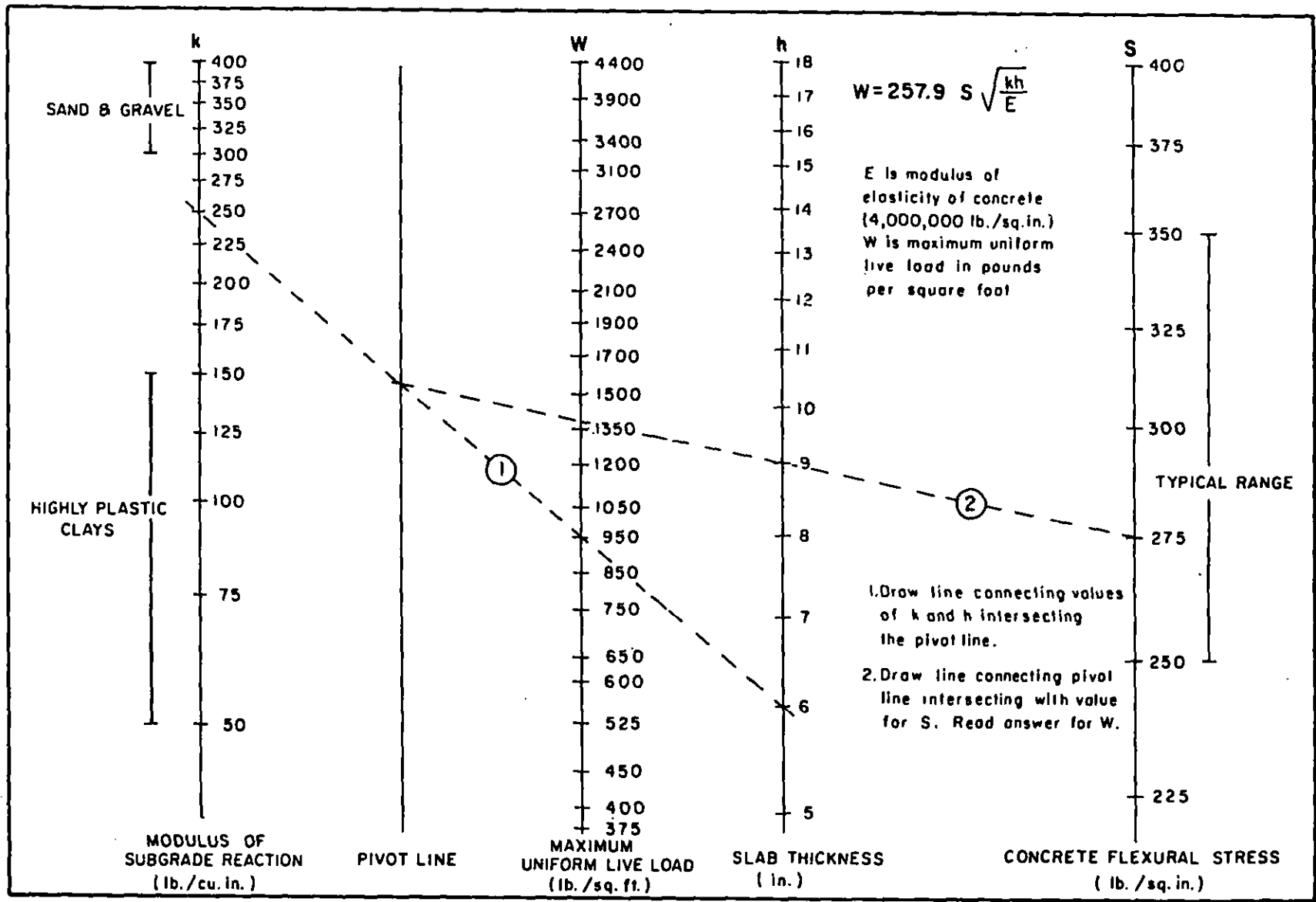
Figure 18 Floor Loading Nomograph
