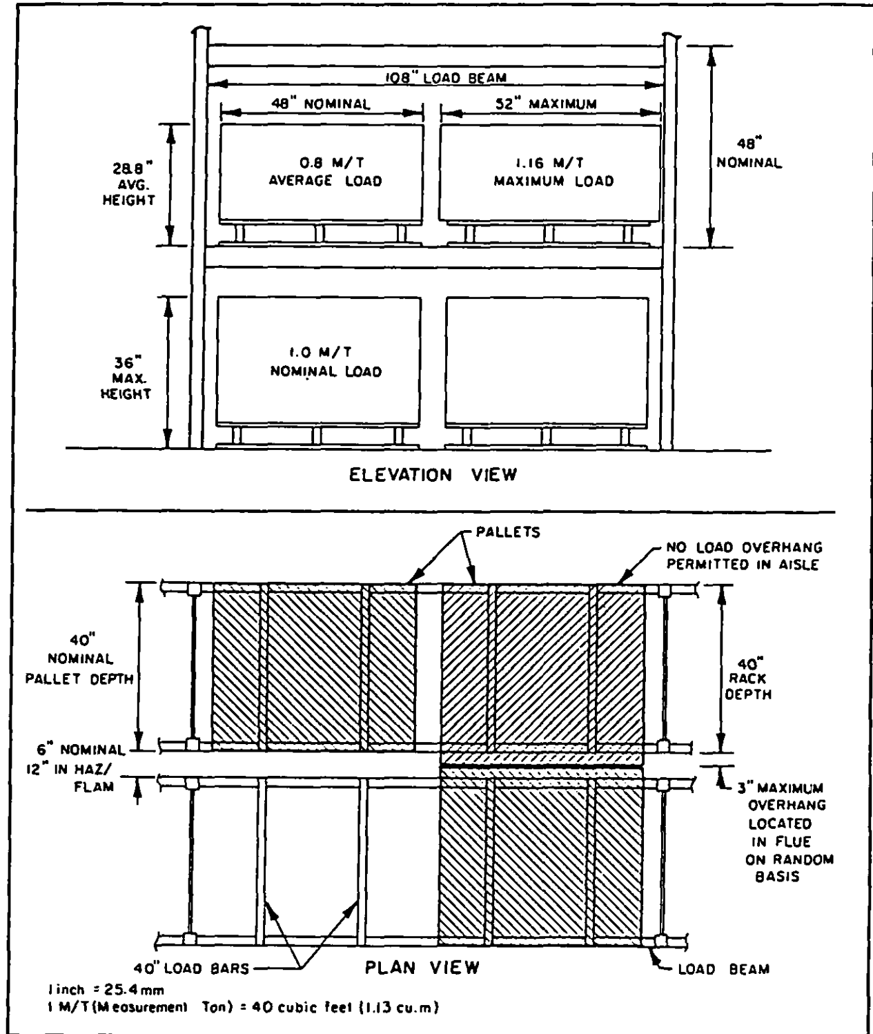
Figure 26 Navy/DOD Pallet Arrangement
