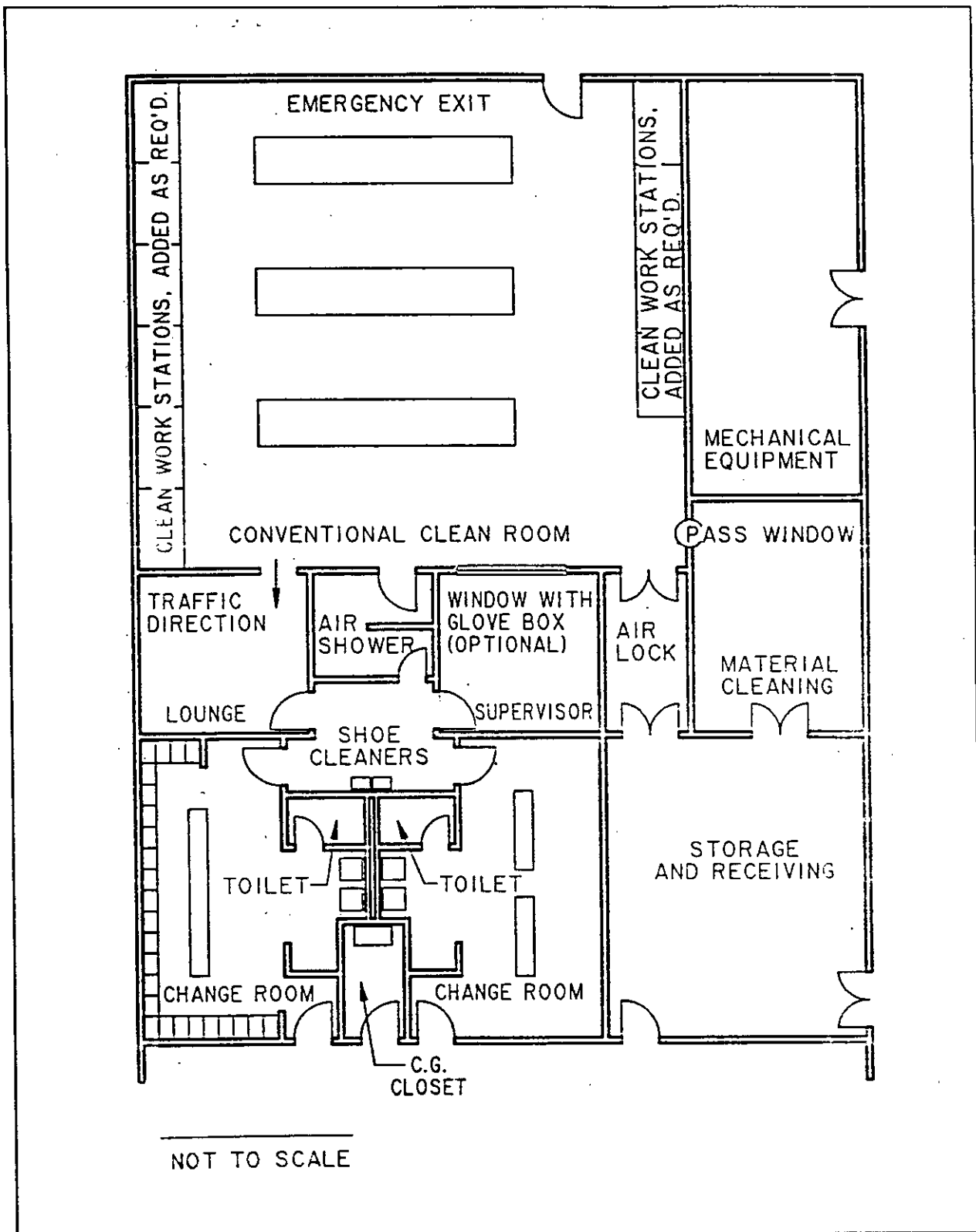
Figure 9 Plan View of a Conventional Clean Room Area With Clean Work Stations
