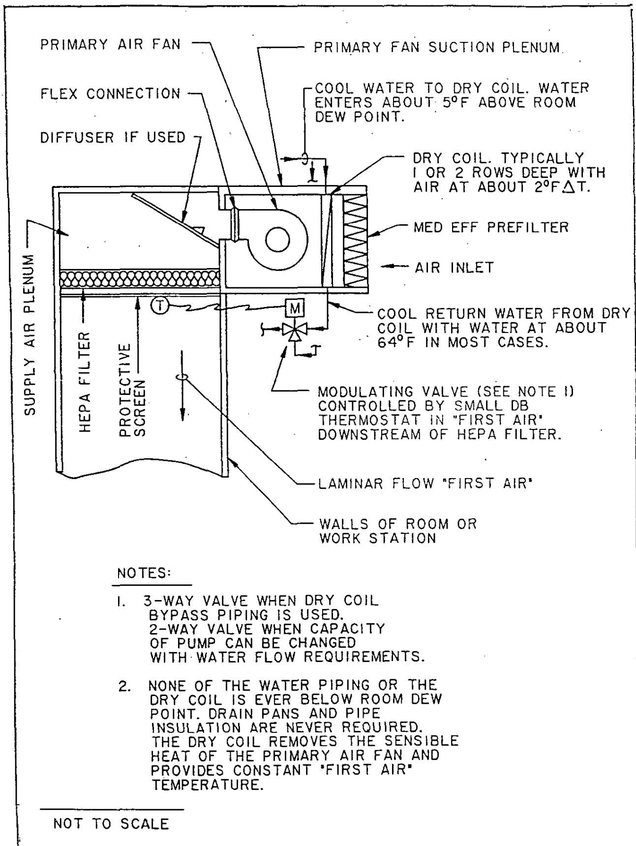
Figure 1 Primary Airstream Using a Dry Coil
