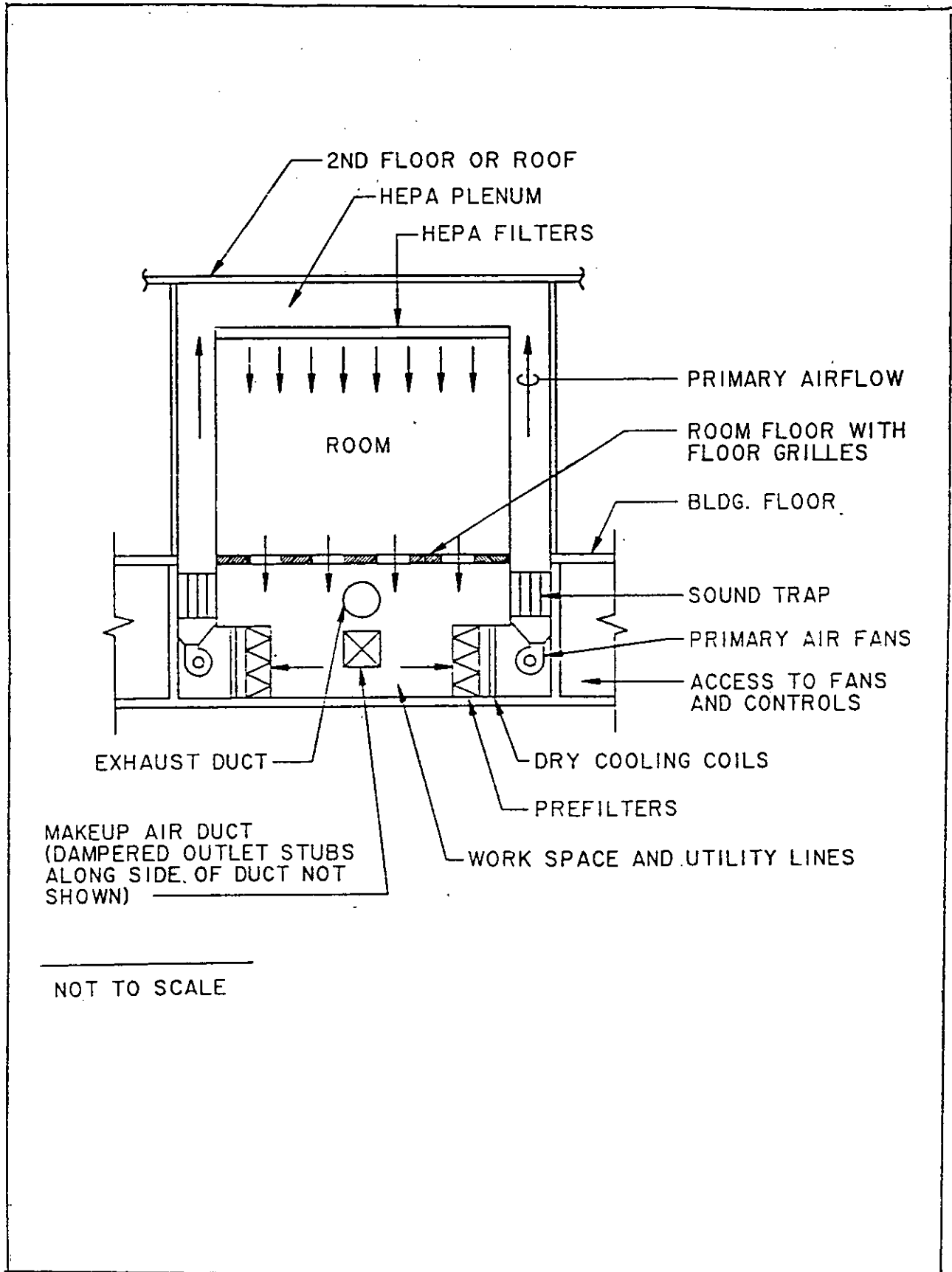
Figure 12 Vertical Flow Room with Basement
