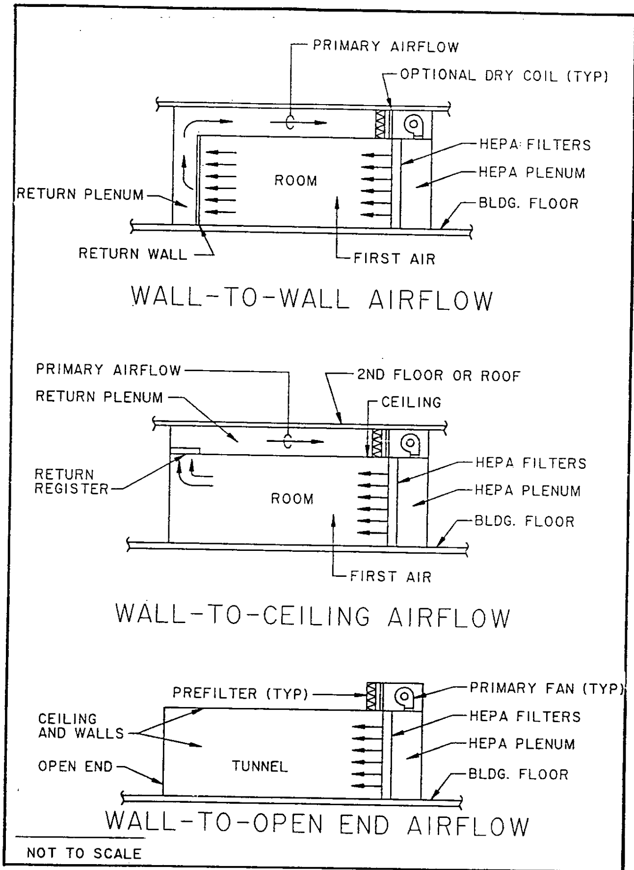
Figure 10 Horizontal Laminar Airflow Paths
