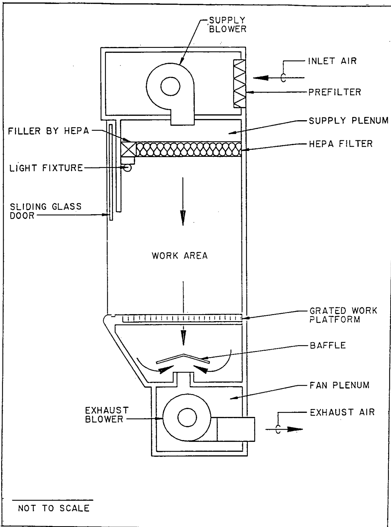
Figure 18 Laminar Flow Exhaust Hood 51
