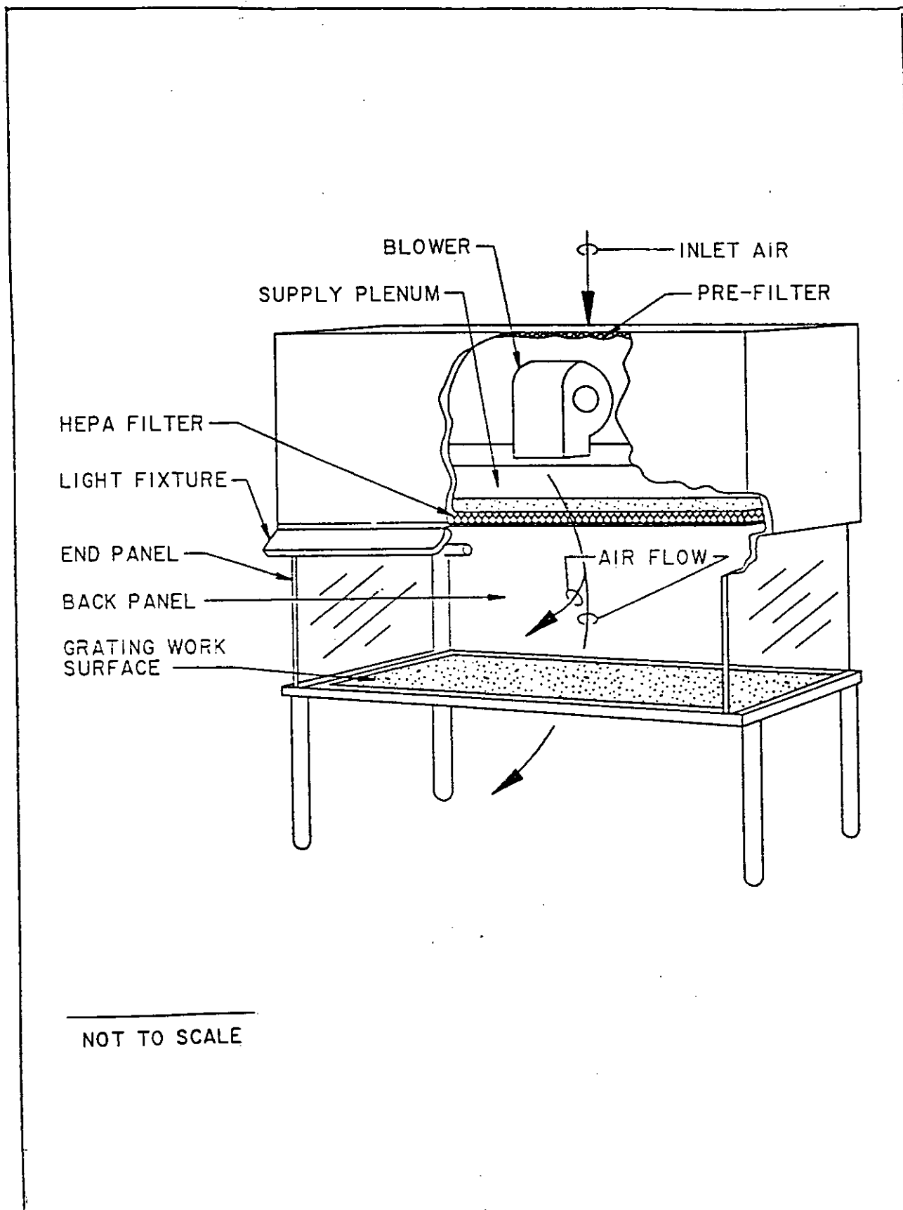
Figure 17 Vertical Laminar Flow Bench 50
