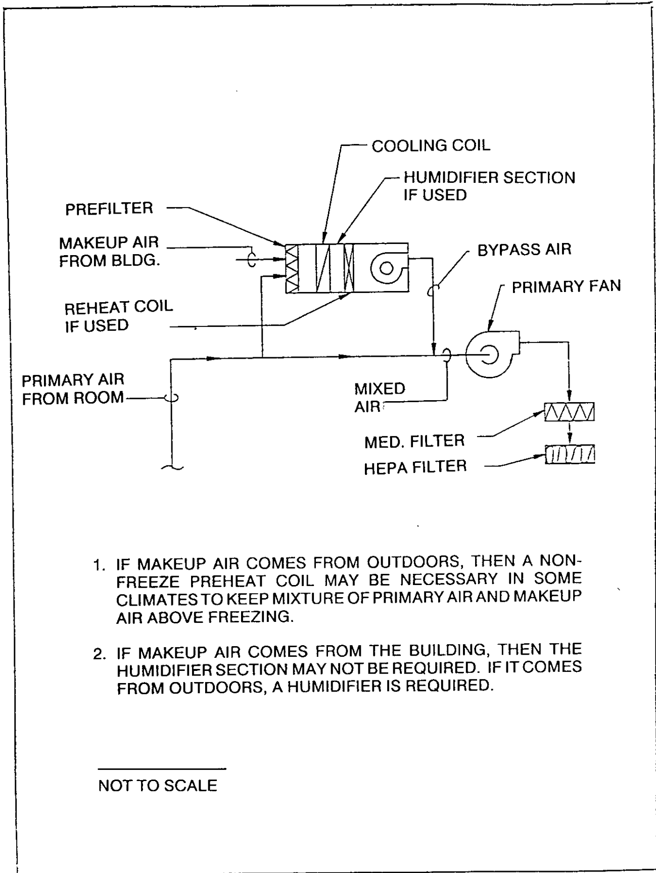
Figure 4 Primary Airstream with Bypass Air
