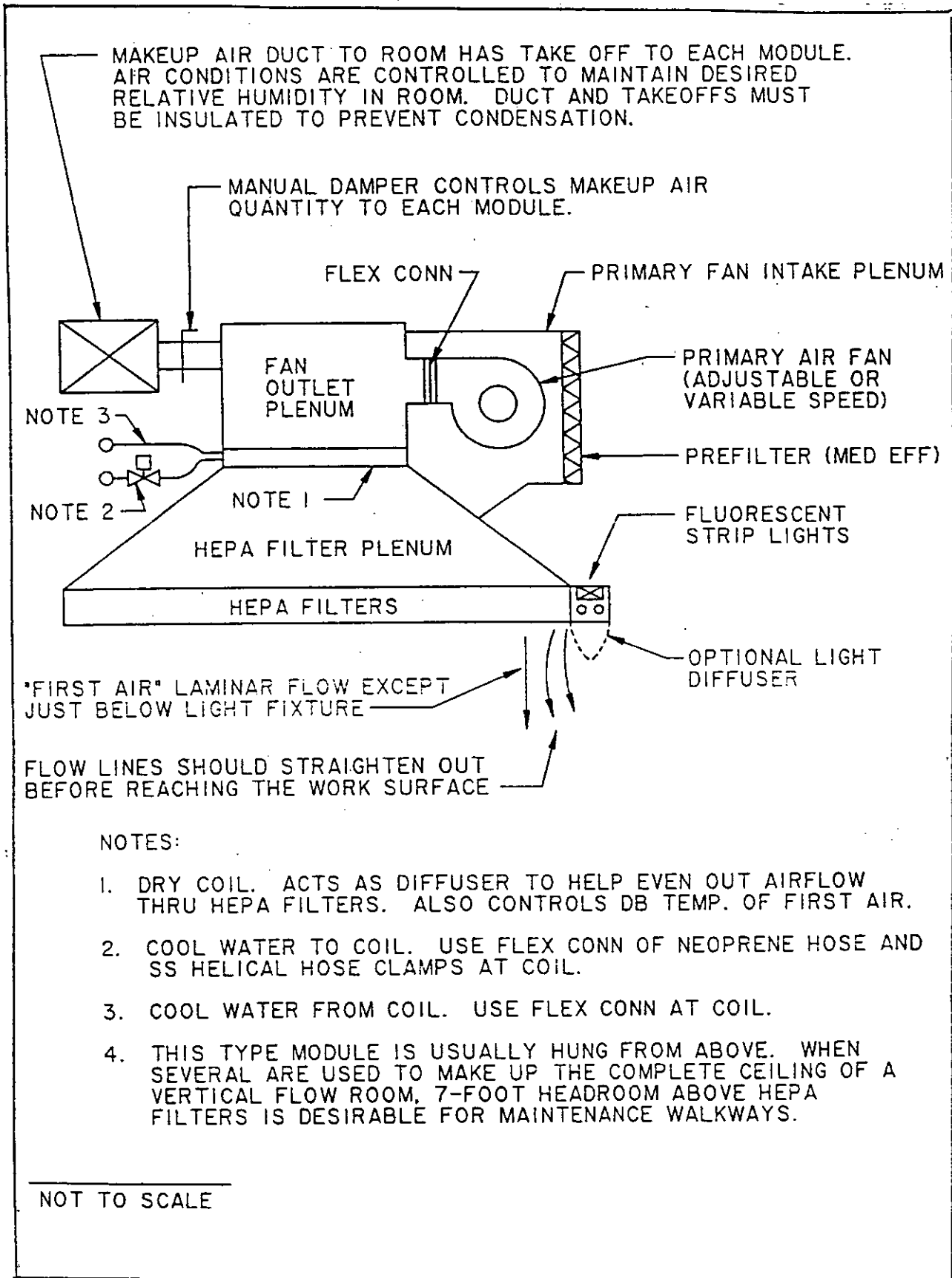
Figure 13 Vertical Flow Ceiling Unit
