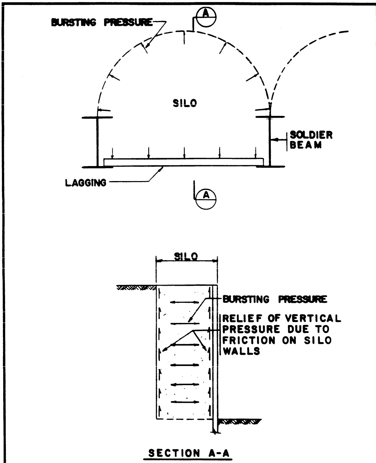
Figure 29 Silo Walls
