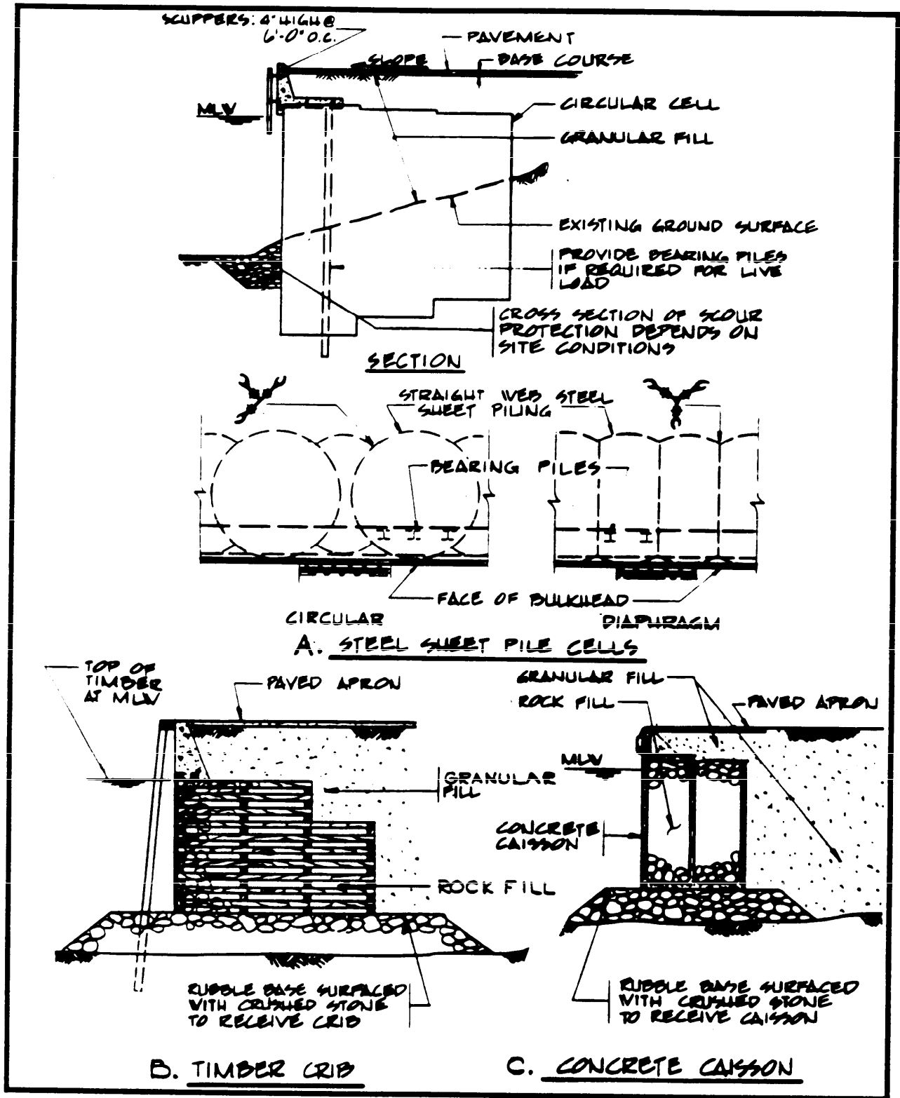
Figure 35 Types of Quaywalls (Examples A thru C)
