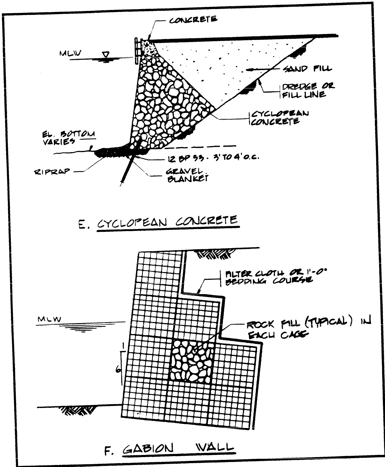
Figure 37 Types of Quaywalls (Examples E and F)
