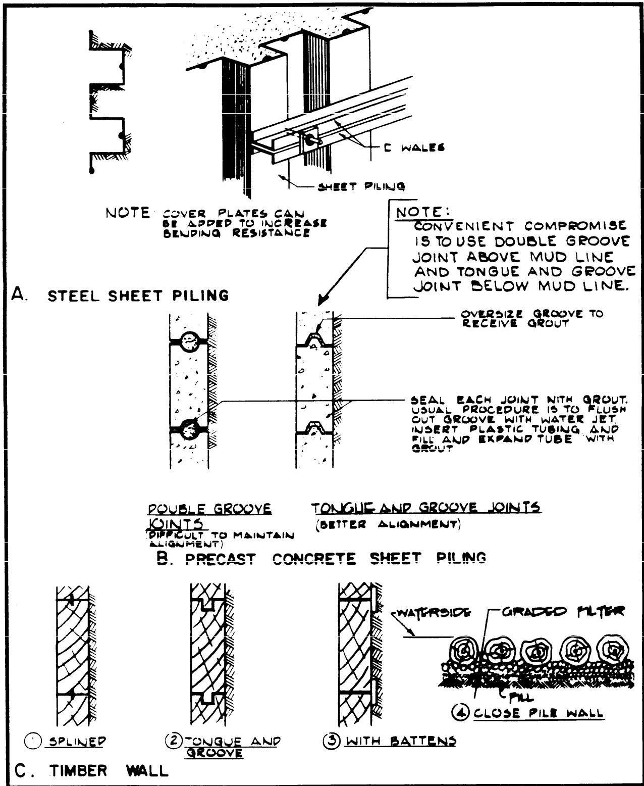
Figure 27 Types of Front Wall (Examples A thru C)
