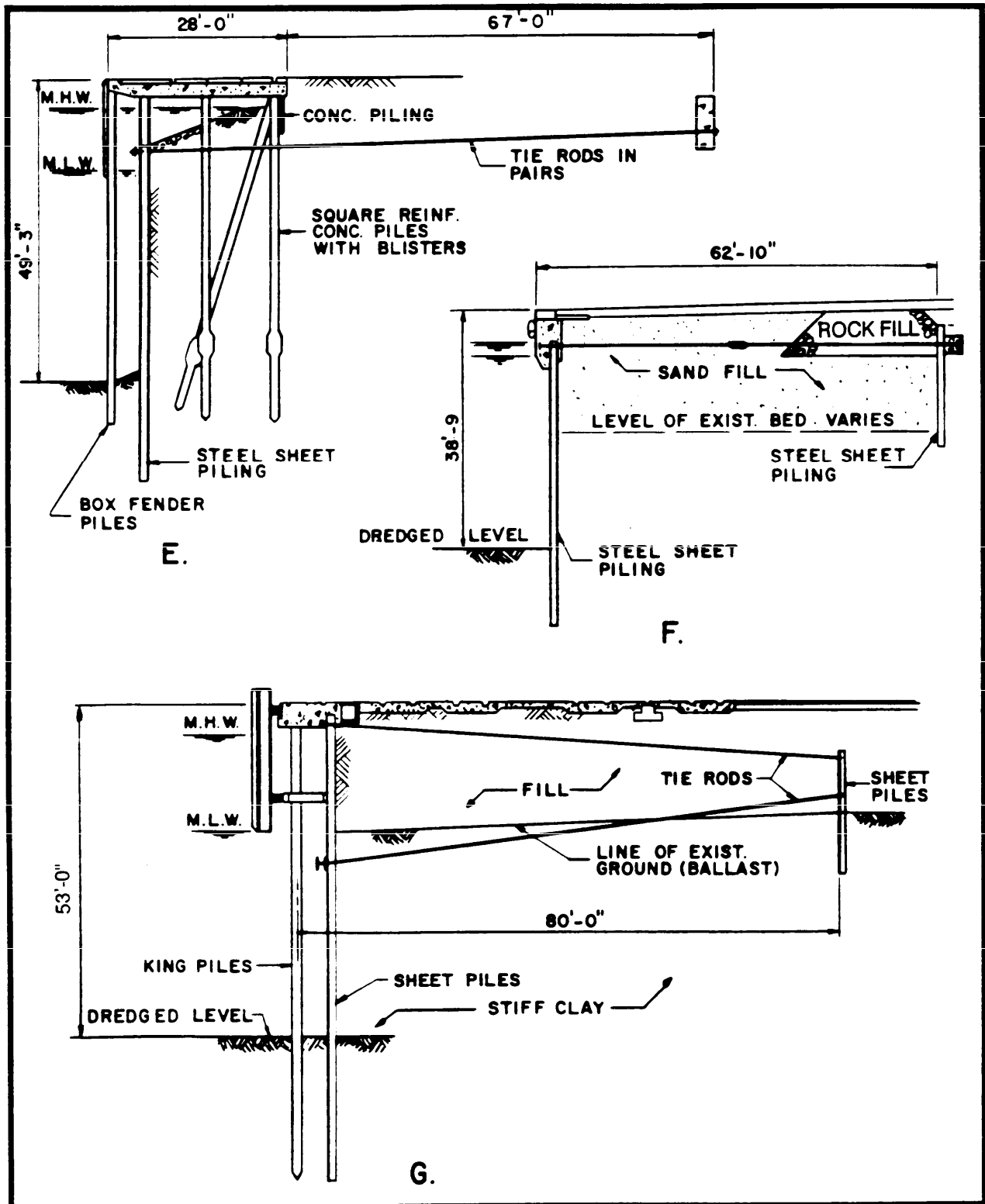
Figure 12 Bulkheads - Actual Constructions (Examples E thru G)
