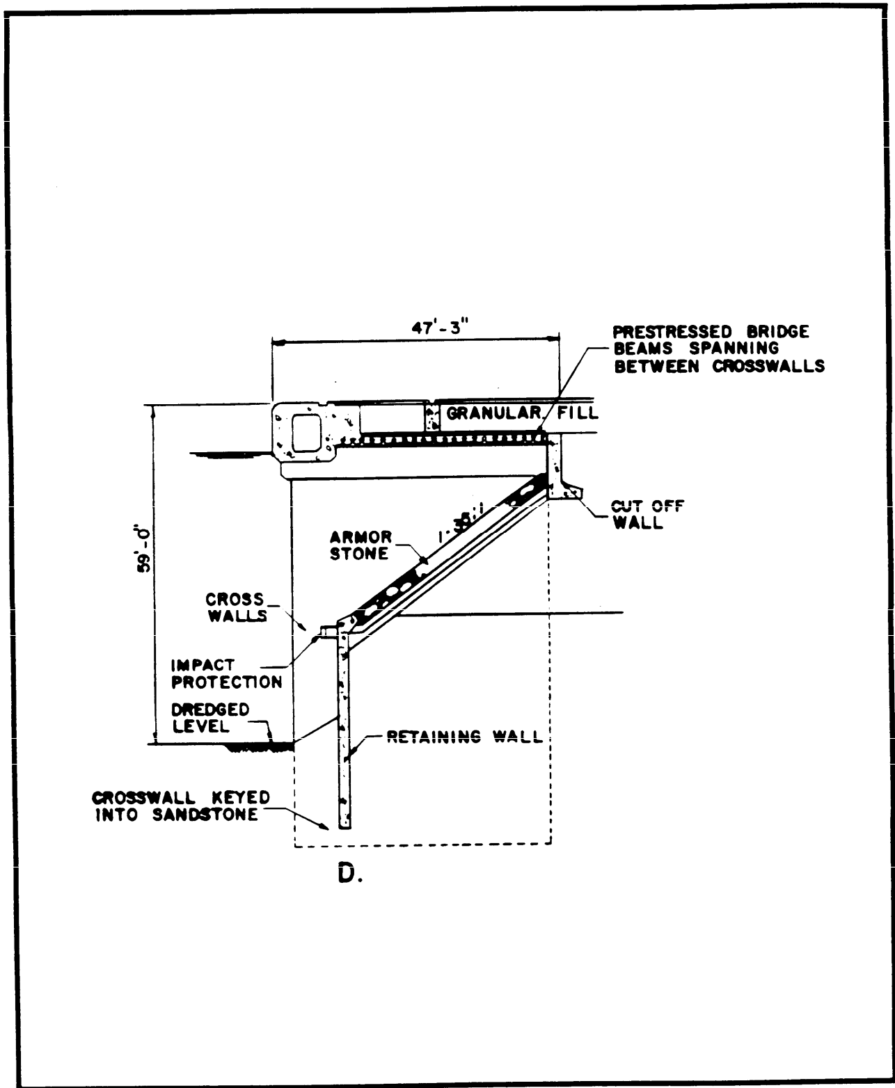
Figure 40 Quaywalls - Actual Constructions (Example D)
