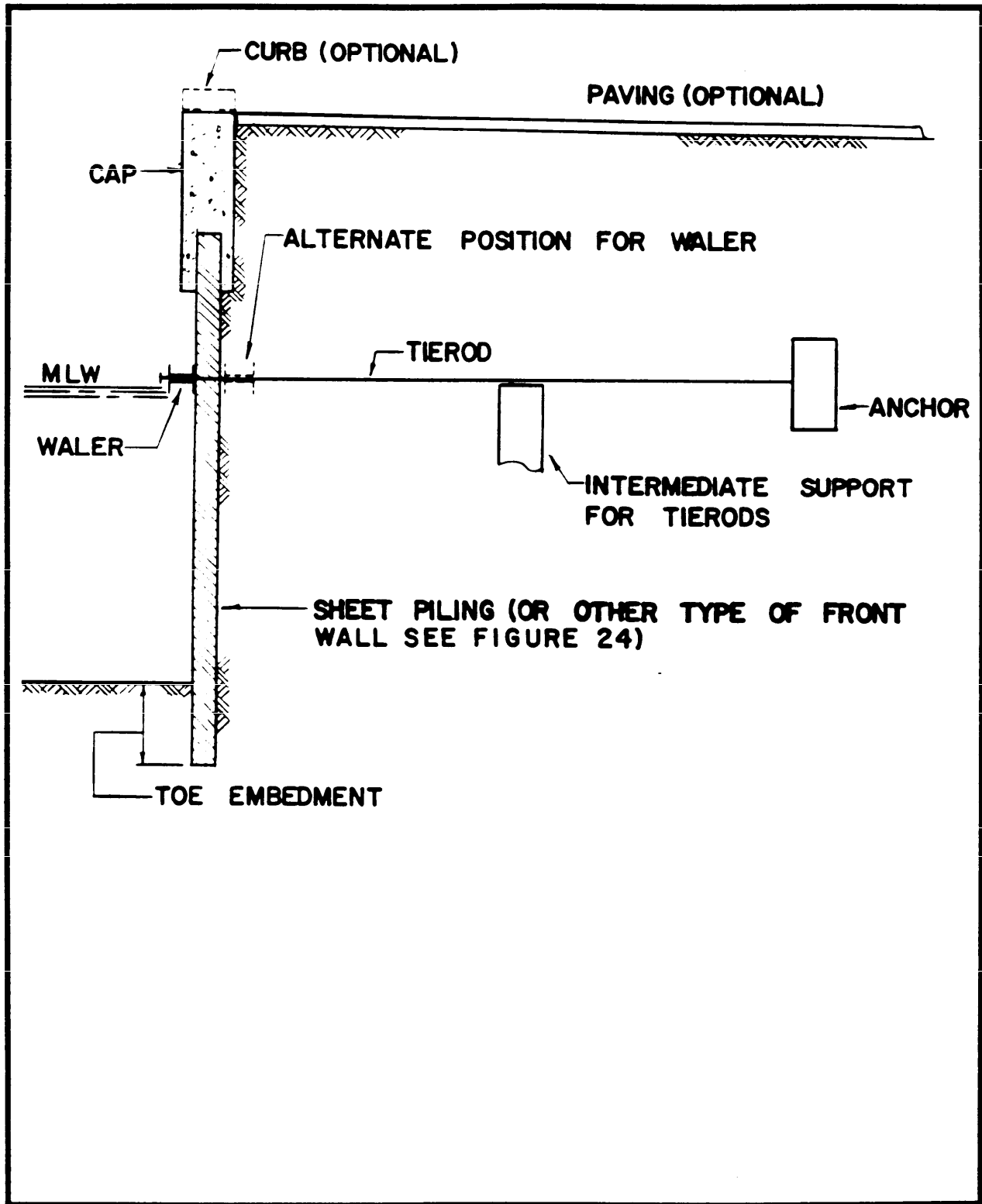
Figure 16 Anchored Wall With Single Level of Anchorage
