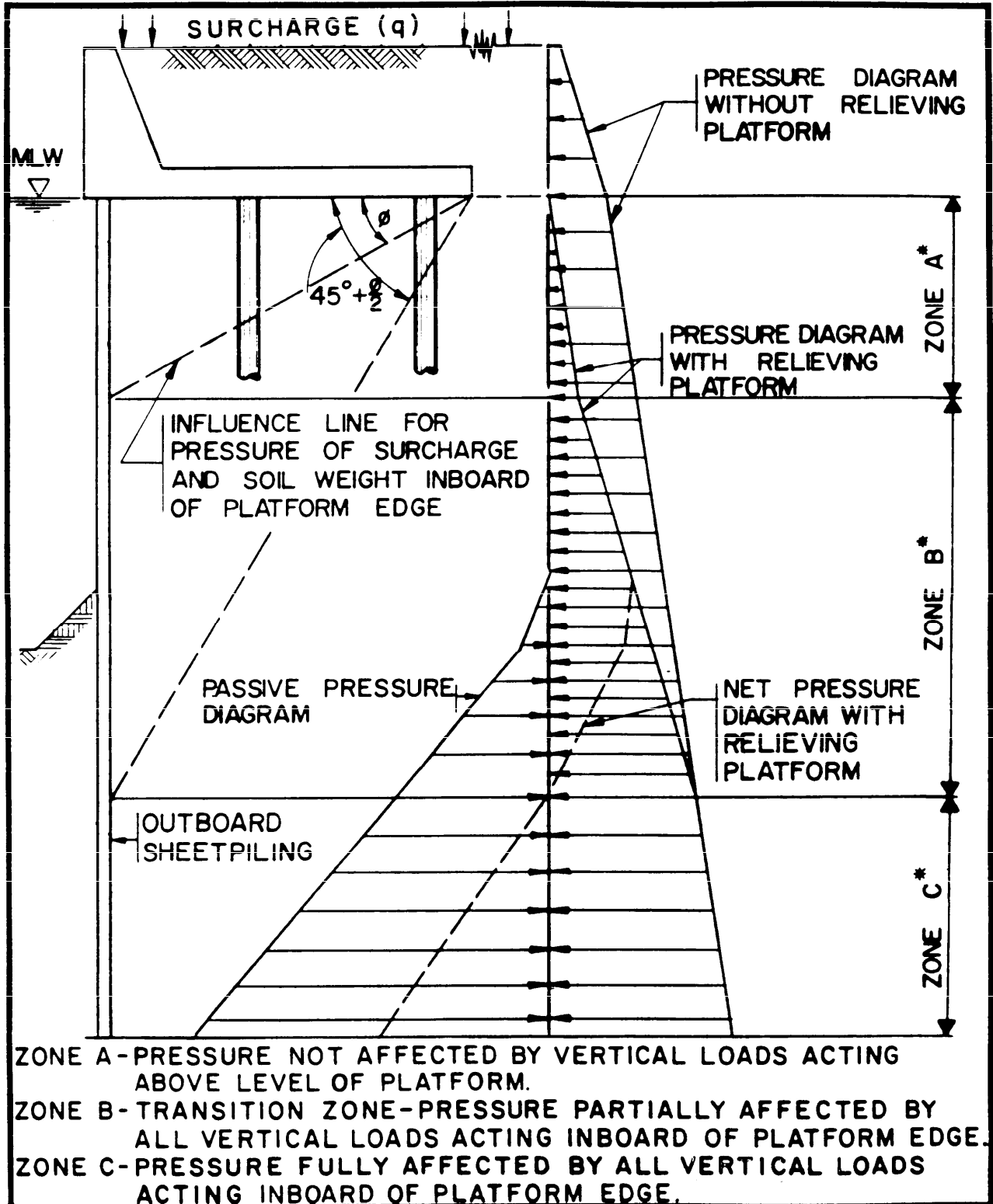
Figure 17 Relieving Platform
