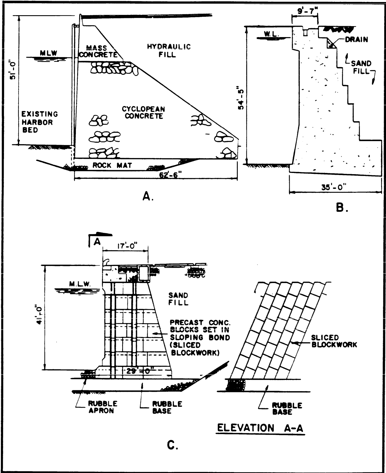
Figure 39 Quaywalls - Actual Constructions (Examples A thru C)
