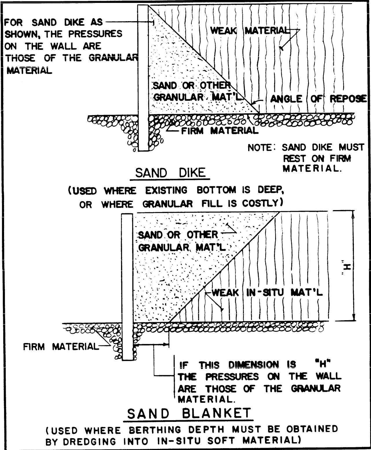
Figure 24 Sand Dike and Sand Blanket
