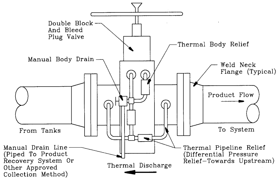
INTEGRAL VALVE THERMAL RELIEF PIPING SYSTEM
