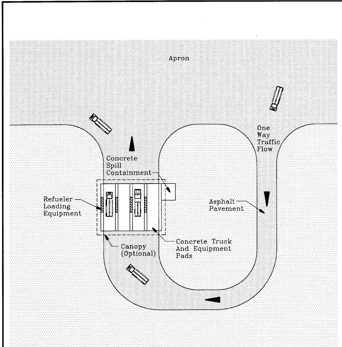
REFUELER TRUCK LOADING LAYOUT PLAN
