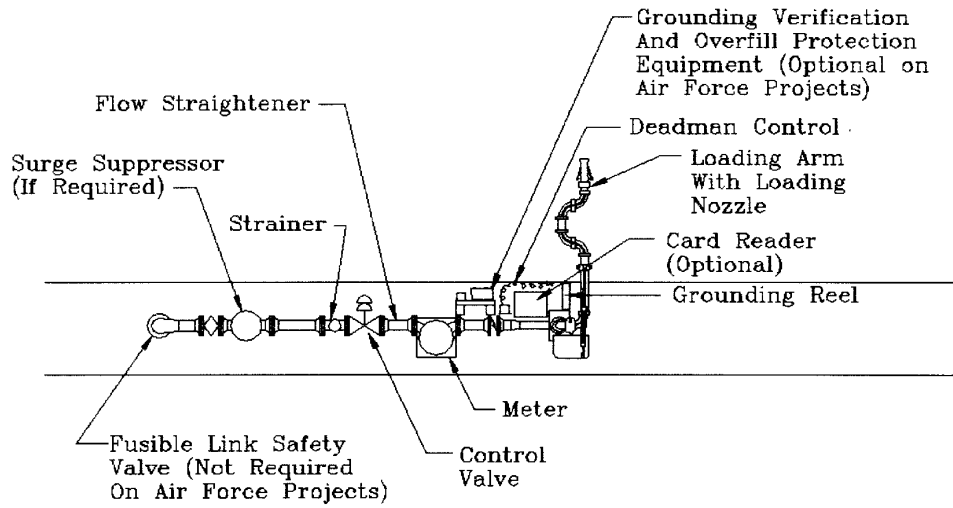
LOADING EQUIPMENT - FROM LATERALS OR NONFERROUS AIRCRAFT DIRECT FUELING SYSTEMS
