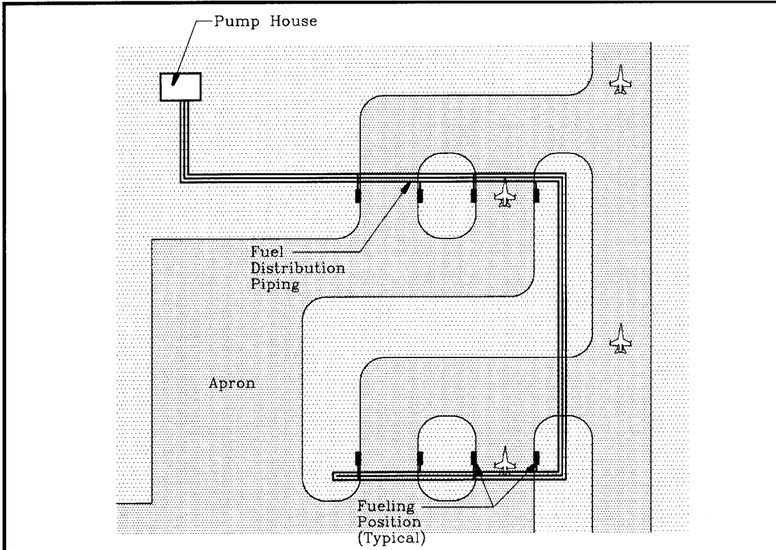
FUELING LANE
