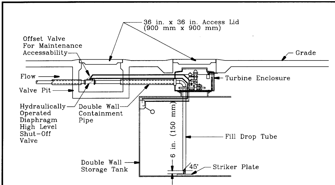
HORIZONTAL UNDERGROUND PUMPED FILL CONNECTION
