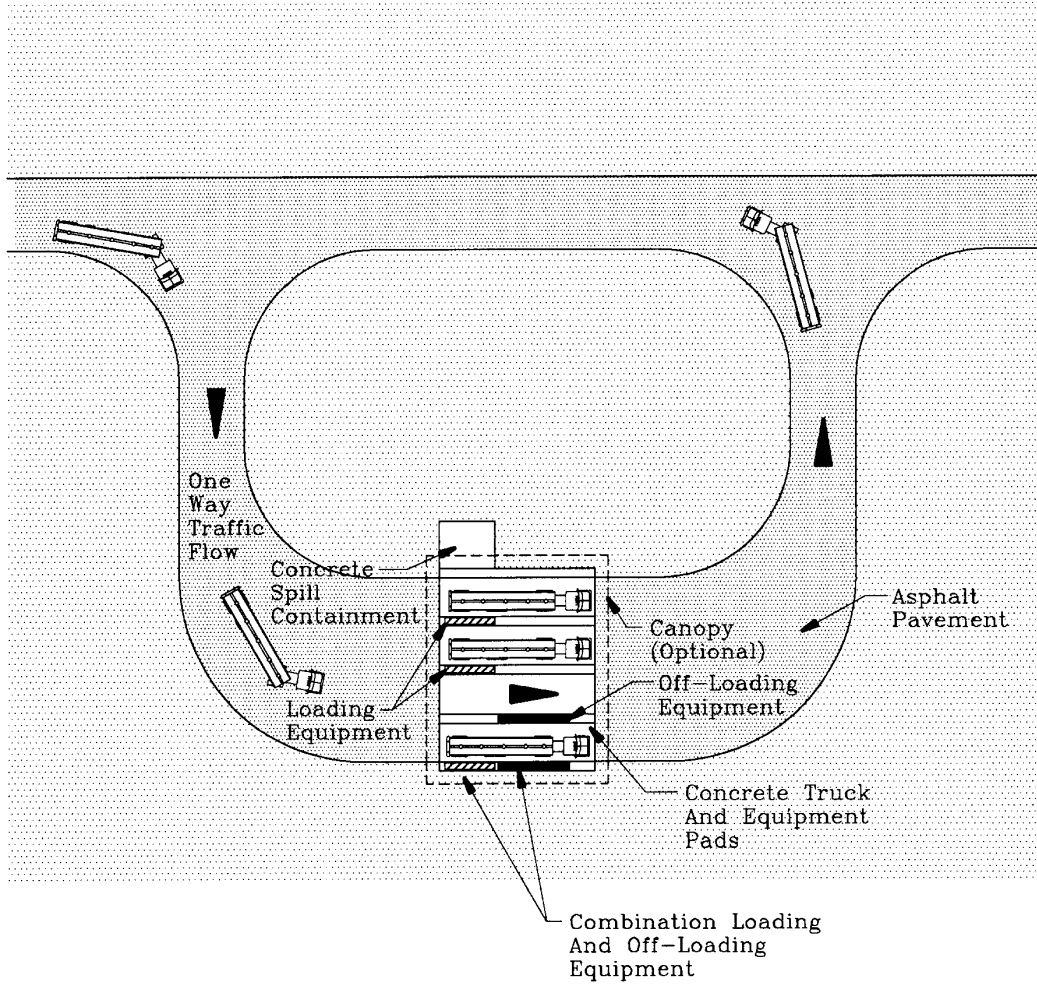
TANK TRUCK LAYOUT PLAN
