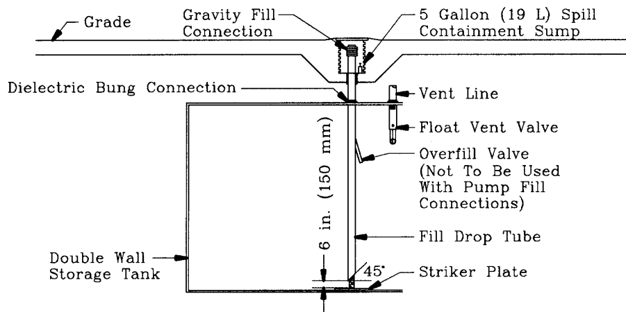
HORIZONTAL UNDERGROUND GRAVITY DROP FILL CONNECTION
