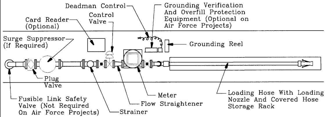
LOADING EQUIPMENT WITH HOSE
