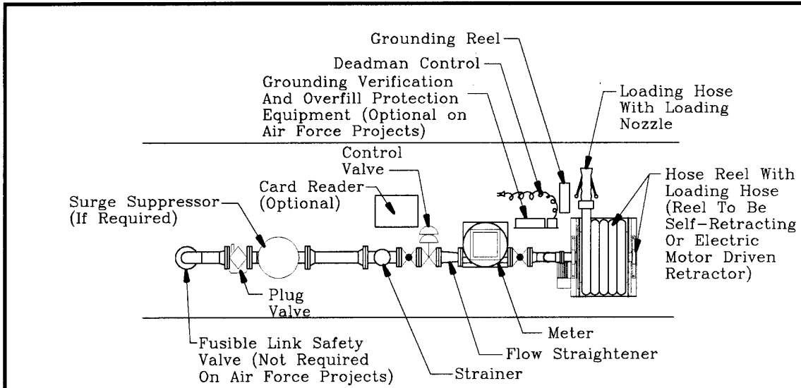
LOADING EQUIPMENT WITH HOSE REEL
