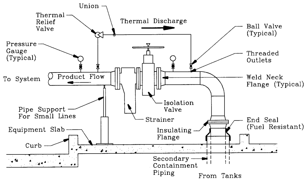
CONVENTIONAL THERMAL RELIEF PIPING SYSTEM
