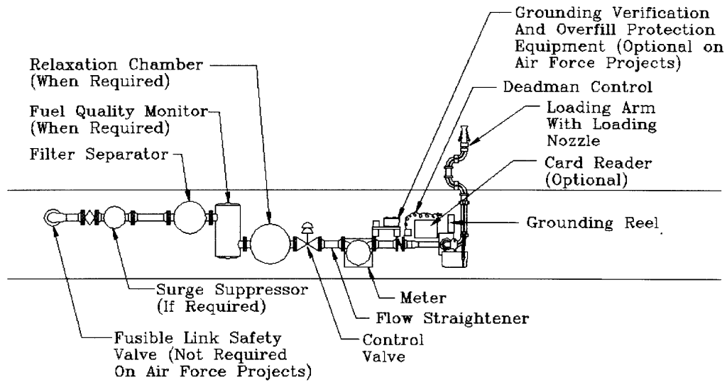
LOADING EQUIPMENT - STAND ALONE
