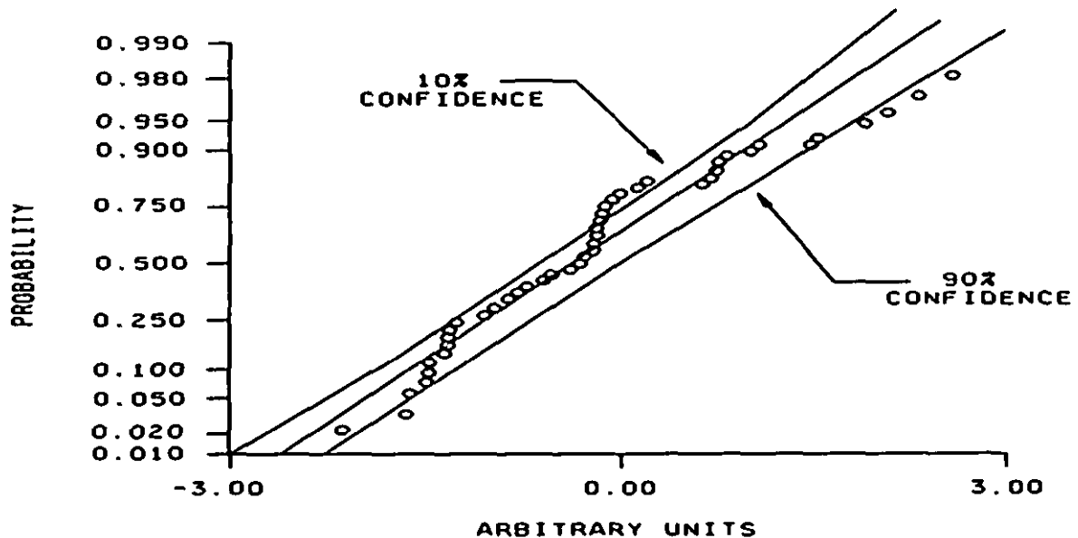
FIGURE 7. Plot of figure 6 with coloring and confidence lines.
