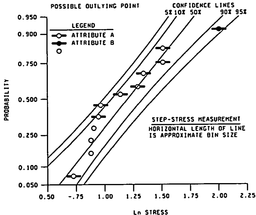
FIGURE 13. Double example of possible outlier and step-stress data - actual data.
