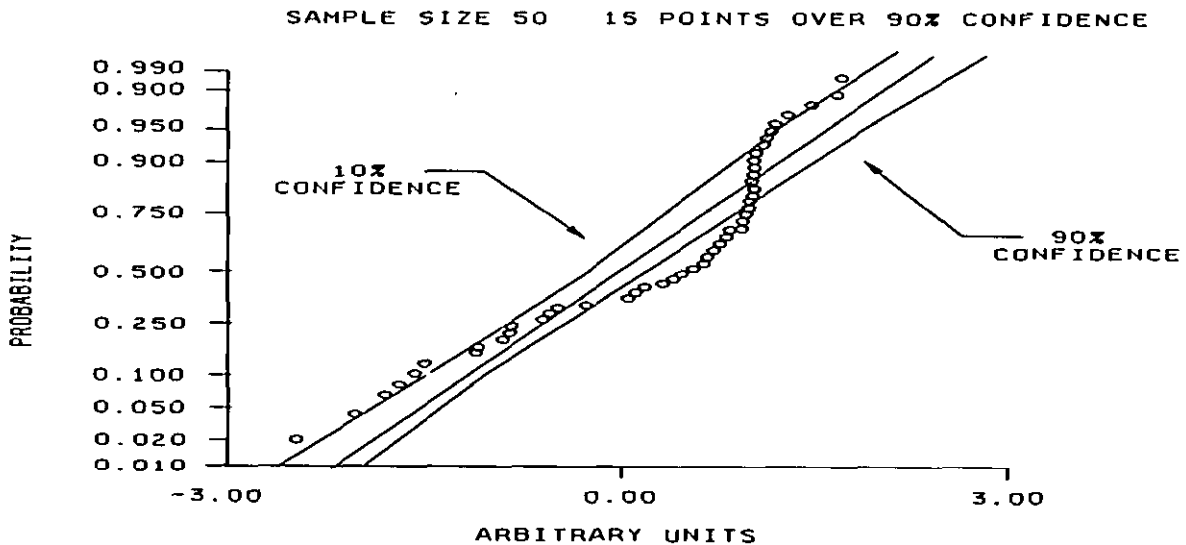
FIGURE 9. Normal probability plot of 50 points with an overly good but still acceptable -simulated data.
