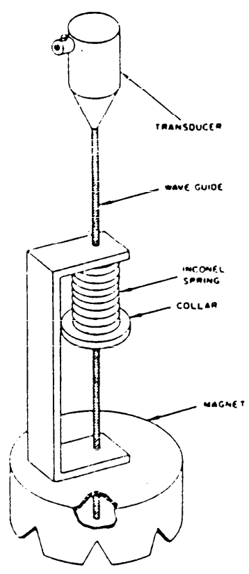
FIGURE 4. A sensor-waveguide assembly.
