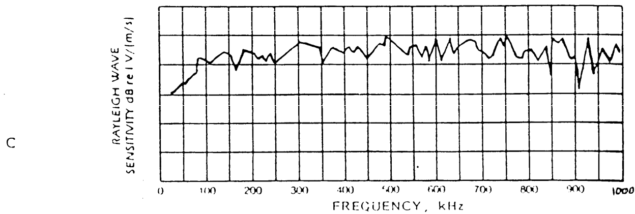
FIGURE 2. Typical surface-wave calibration plots for (A) single-resonance sensor (B) dual-resonance sensor (C) flat-broadband sensor
