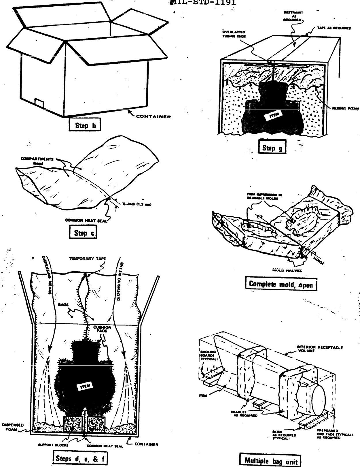
FIGURE 7. Foam-in-bag.
