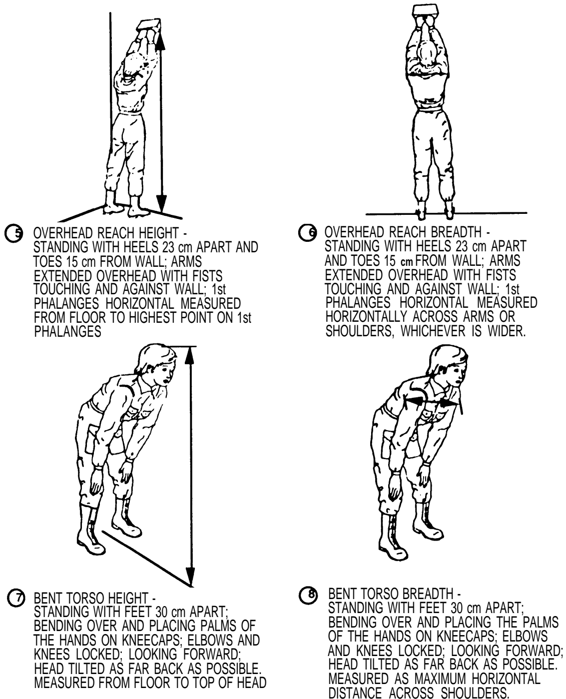
FIGURE 81. Anthropometric data for workspaces - continued
