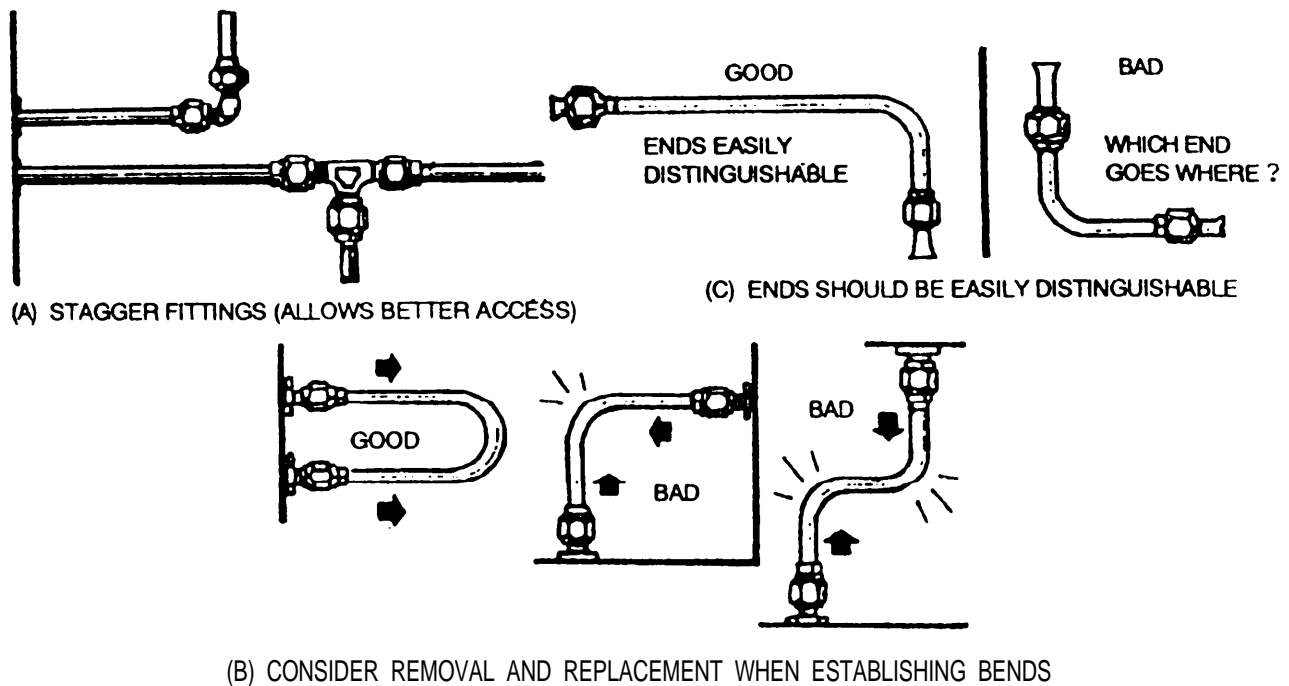
FIGURE 129. Connectors for fluid lines
