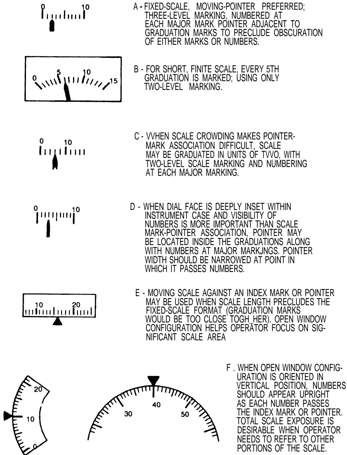
FIGURE 27. Scale graduation, pointer position and scale numbering alternatives
