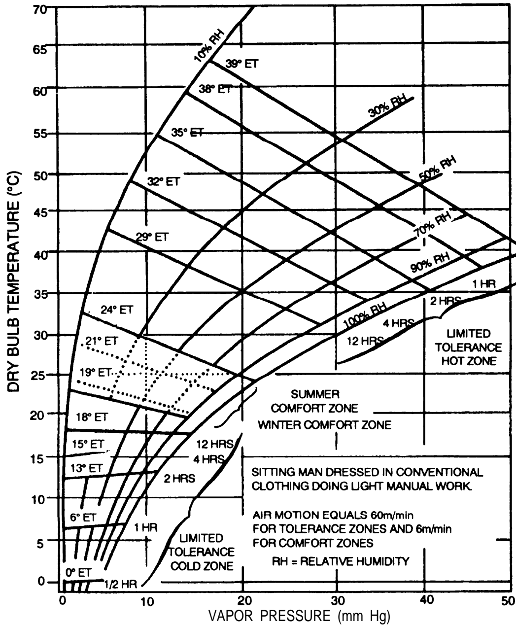
FIGURE 83. Summer and winter comfort zones and thermal tolerance for inhabited compartments
