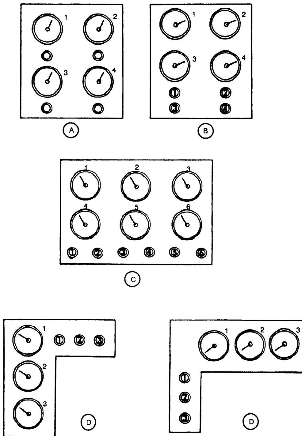
FIGURE 41. Control/display relationship
