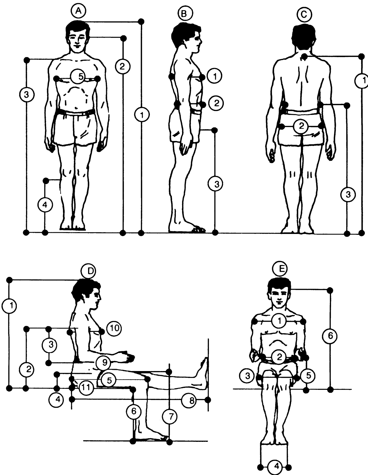
FIGURE 57. Body dimensions
