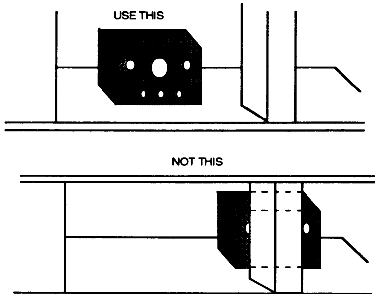
FIGURE 122. Component placement
