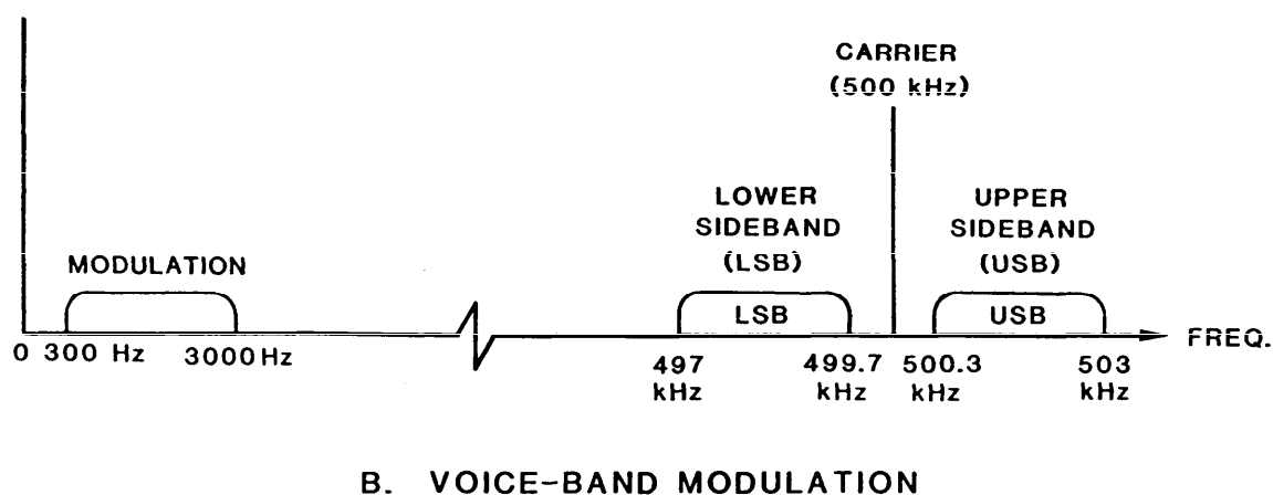
FIGURE 15. AM signal spectrum.
