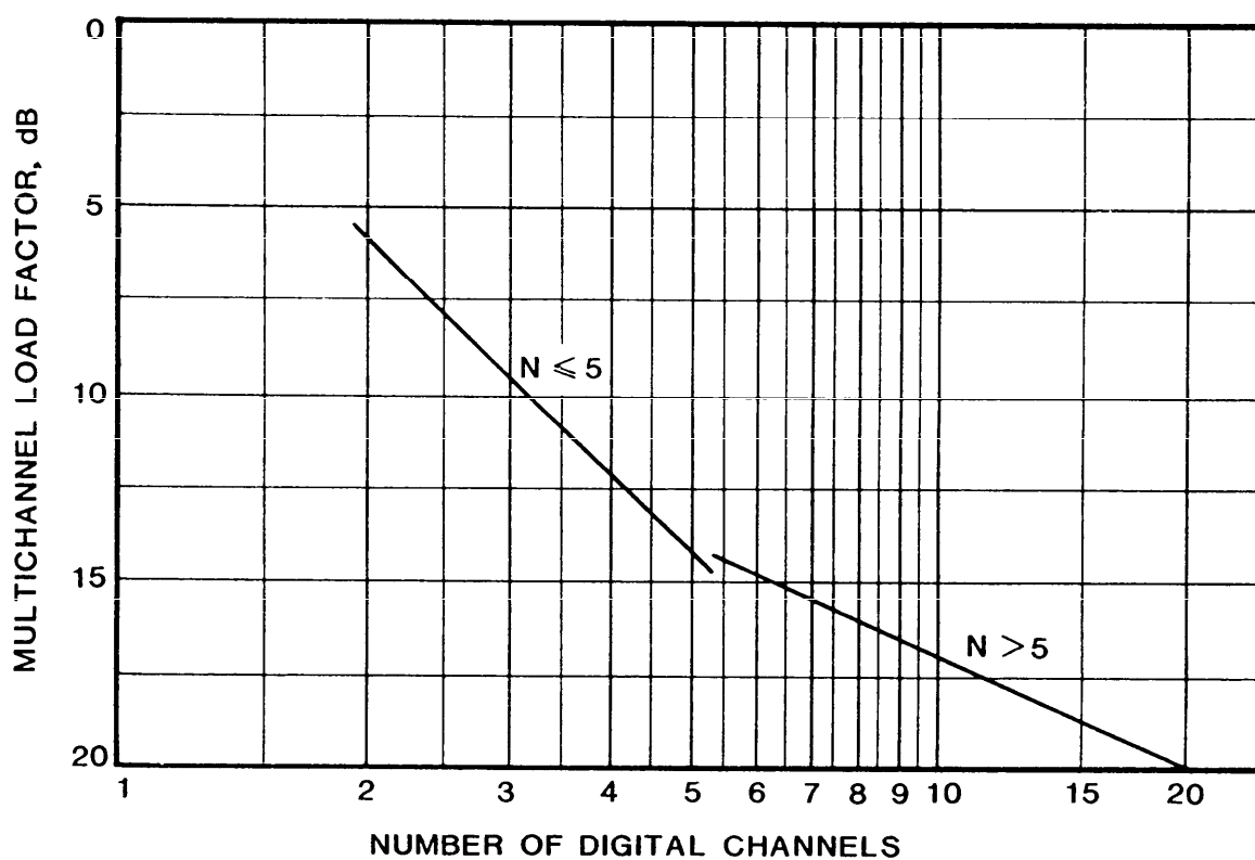
FIGURE 66. Multichannel load factor for digital channels.
