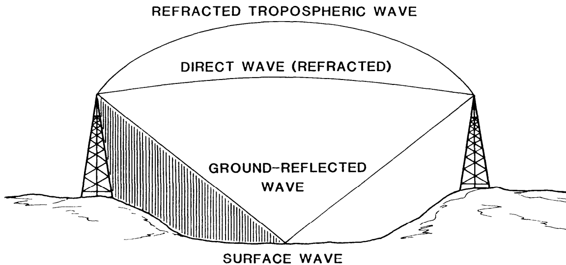
FIGURE 2. Groundwave components.
