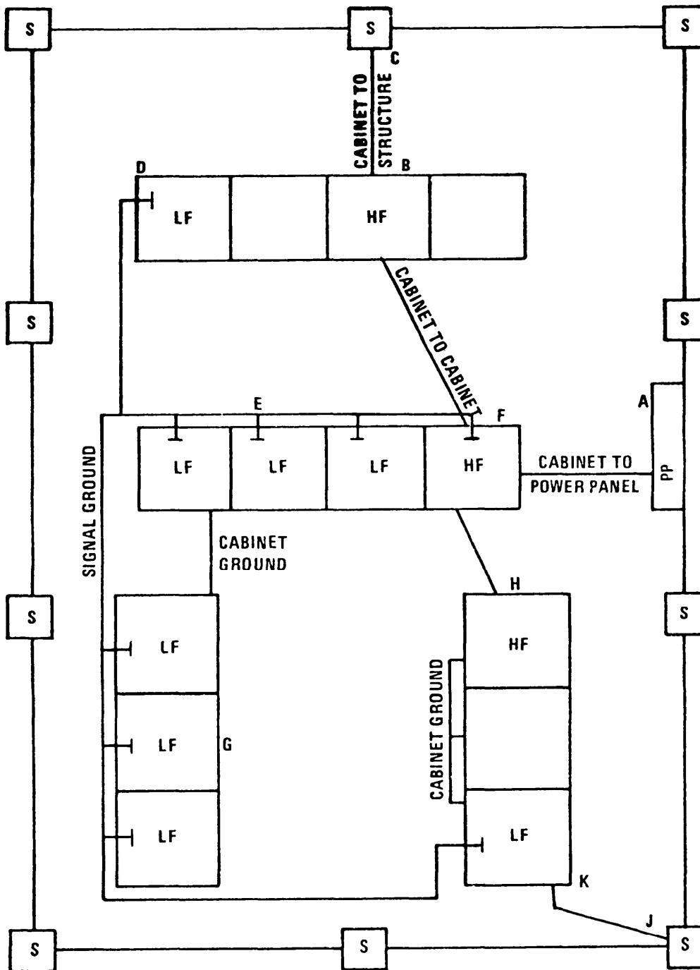
Figure 2-11. Typical Bond Resistance and Stray Current Measurement Locations in an Electronic Facility
