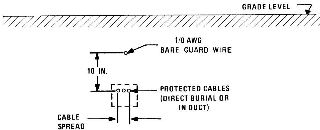
(a) CABLE SPREAD LESS THAN 3 FEET
