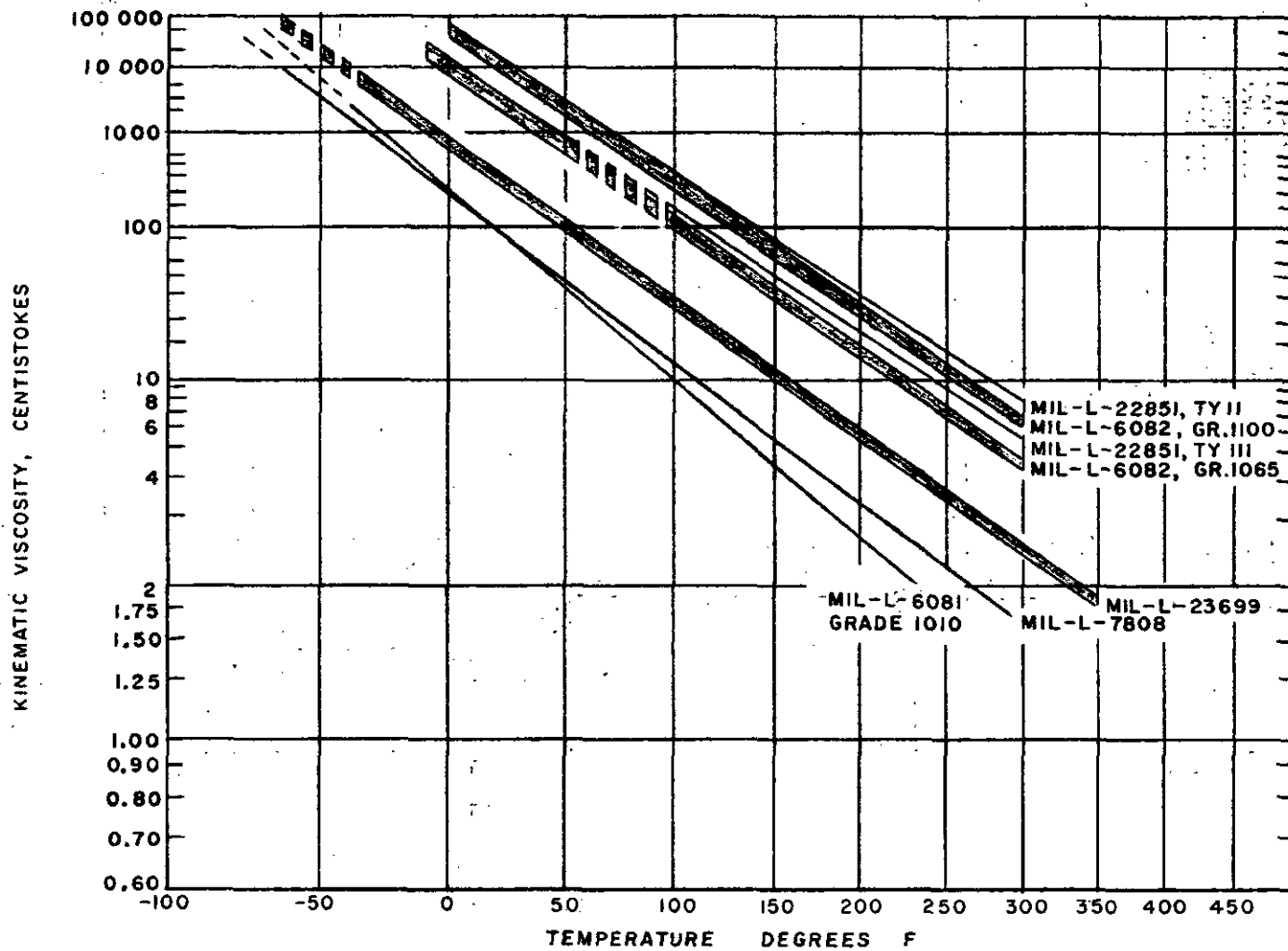
FIGURE 2. Viscosity-temperature characteristics of aircraft engine oils
