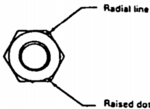
GRADE 5 HEX NUTS (ONE RAISED RADIAL LINE 120° COUNTERCLOCKWISE FROM ONE RAISED DOT ON CHAMFER)
