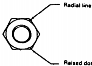
GRADE 5 HEX NUTS (ONE RAISED RADIAL LINE 120° COUNTERCLOCKWISE FROM ONE RAISED DOT ON CHAMFER)
