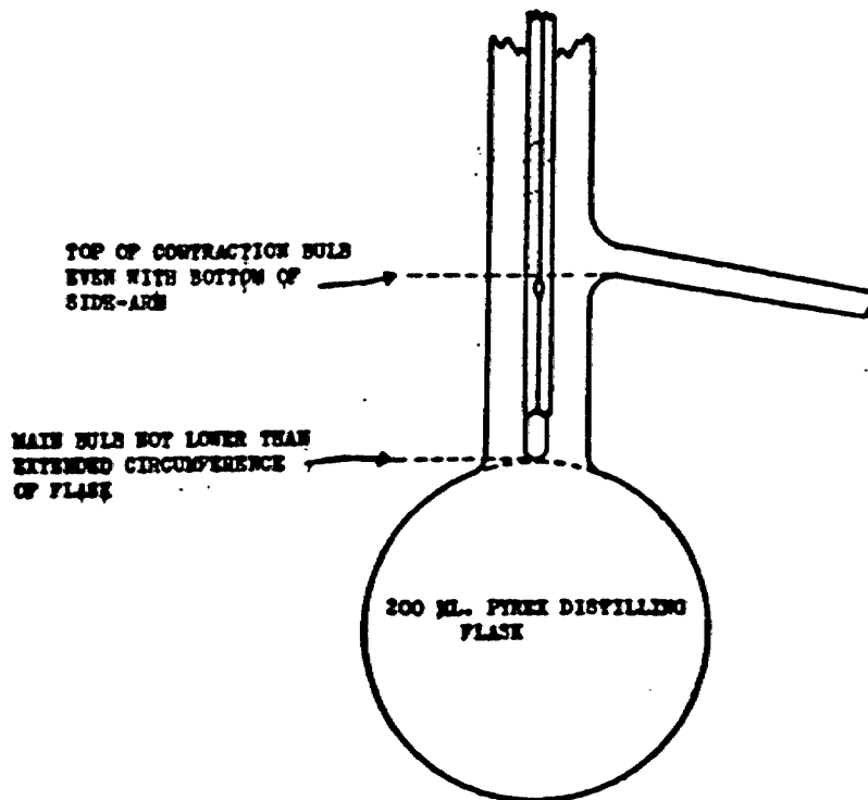
FIGURE 2.—Position of distillation thermometer in flask.
