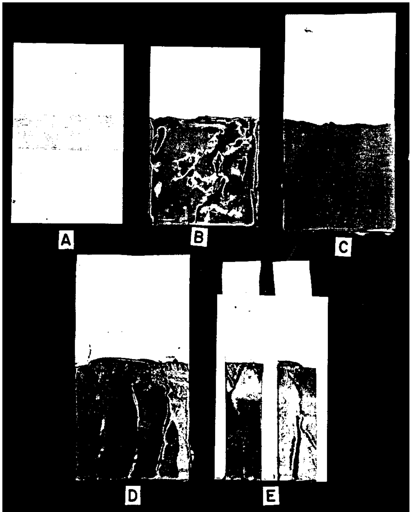
FIGURE 8. Stages in the preparation of the adhesion in peel test specimen.
