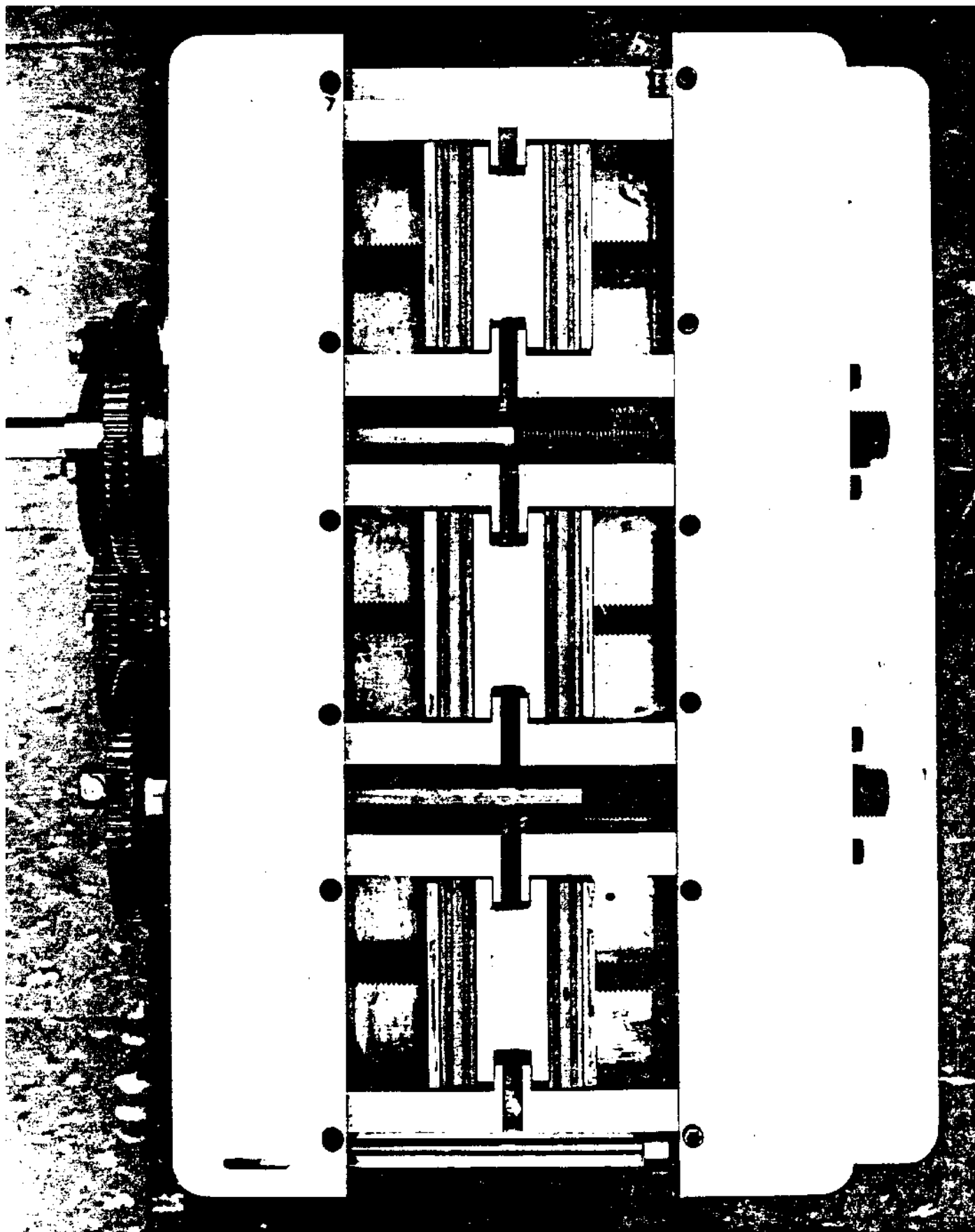
FIGURE 6b. Top view of the machine noted in 6a, showing 3 specimens ready for automatic compression-extension cycling. Also noted are cushioning blocks and pressure plates.
