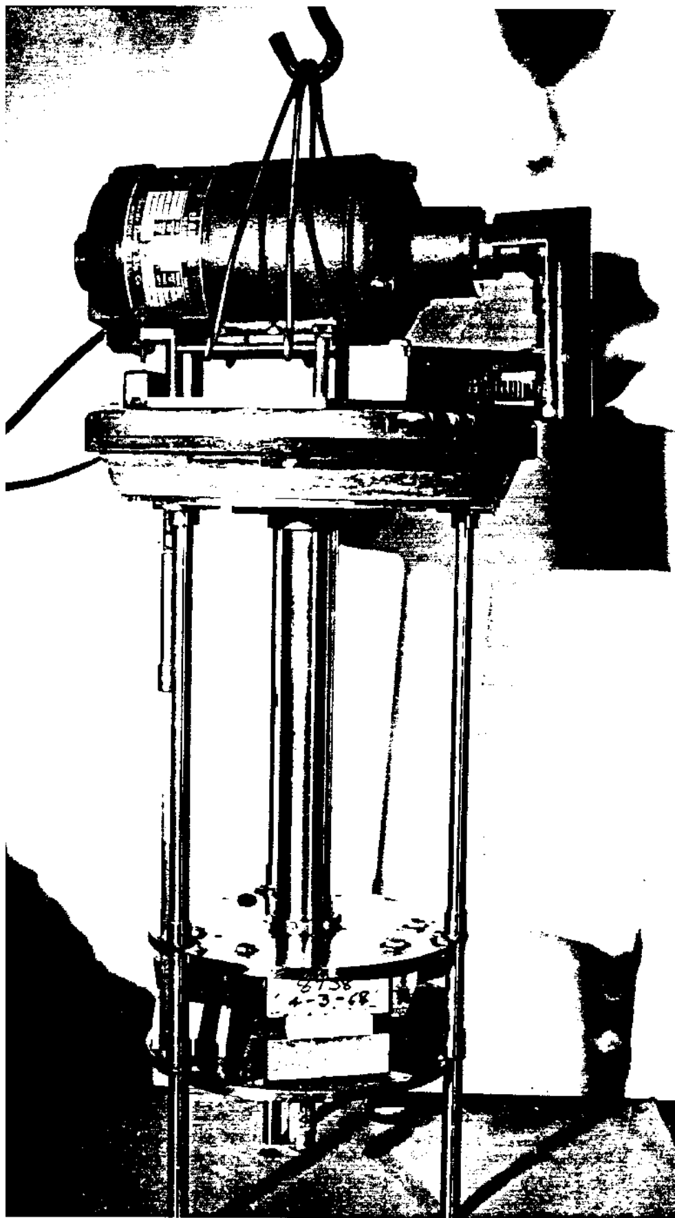
FIGURE 6c. A motor driven machine used for extension of specimens at -15^{\circ}\text{F} . in the Durability test.
