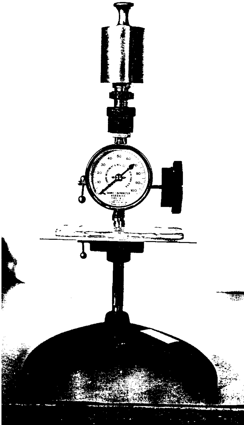
FIGURE 3a. Durometer fitted to operating stand with 822 gram load, for hardness determination.
