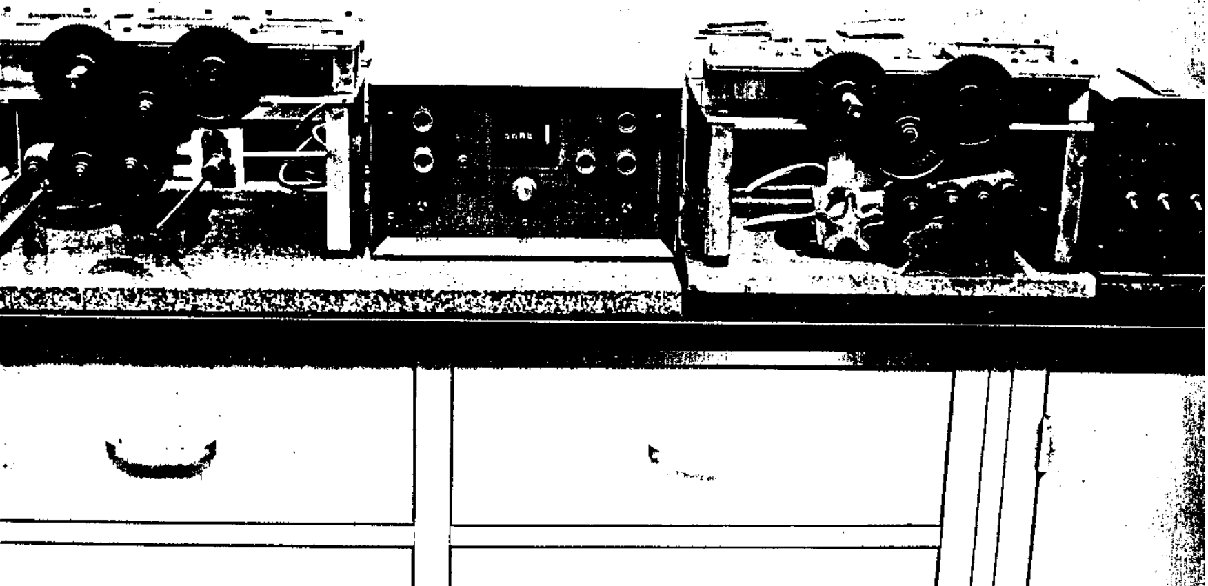
FIGURE 6a. Compression-extension machines with automatic control units, used in the Durability test.
