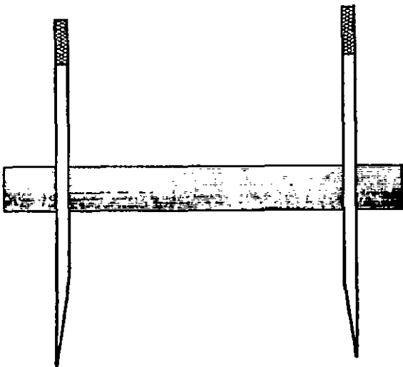
FIGURE 6. TYPE III, class A scriber points.
