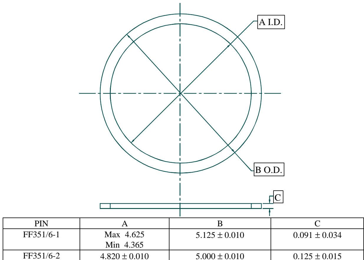
Figure 1. Oil filter cover gaskets.
