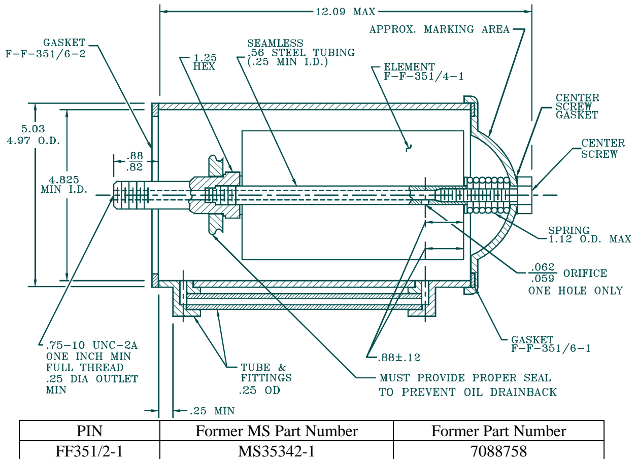
Figure 1. Filter assembly with element.
