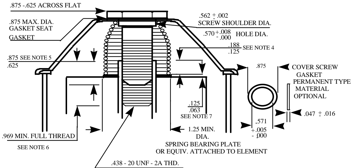
Figure 2. Filter assembly dimensions.
