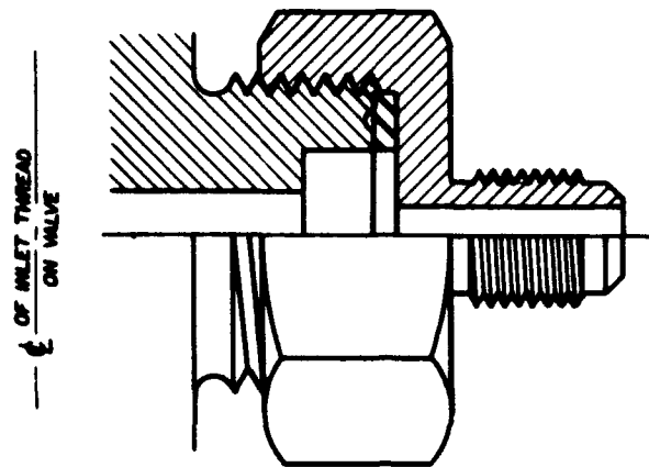
CONNECTION NO. 620
