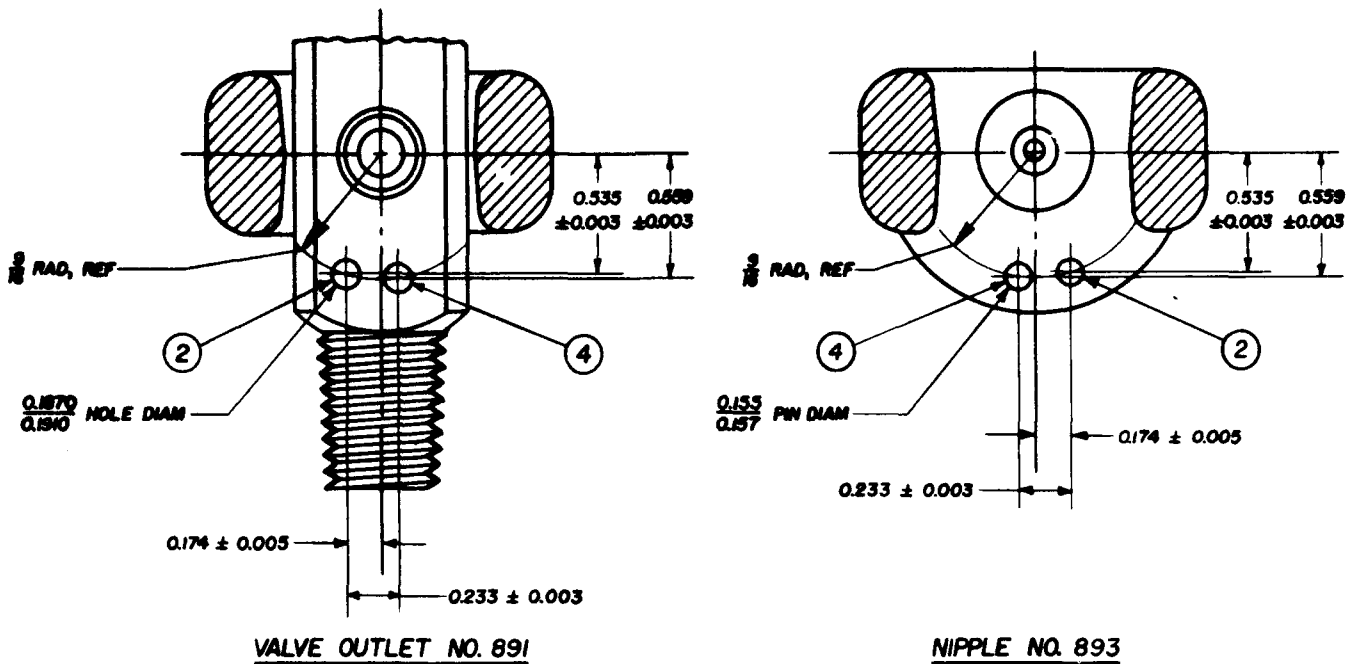
FIGURE IX.29.—No. 890 standard valve outlet connection, yoke type, for oxygen-helium mixtures (helium not over 80 per cent), medical.
