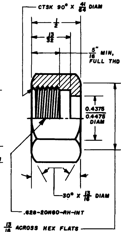
HEX NUT NO. 204
