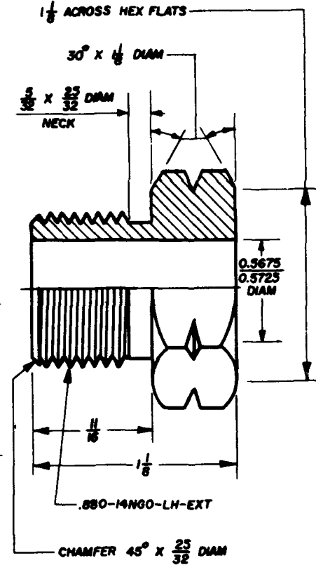
HEX NUT NO. 514
