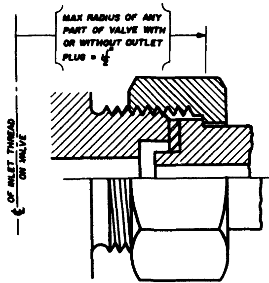
CONNECTION NO. 660
