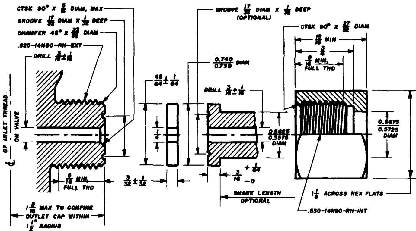
CONNECTION NO. 320
