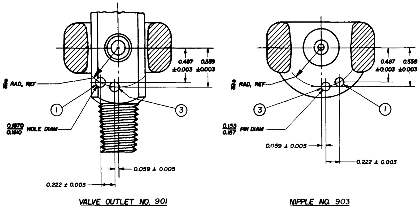
FIGURE IX.30.—No. 900 standard valve outlet connection, yoke type, for ethylene, medical.
