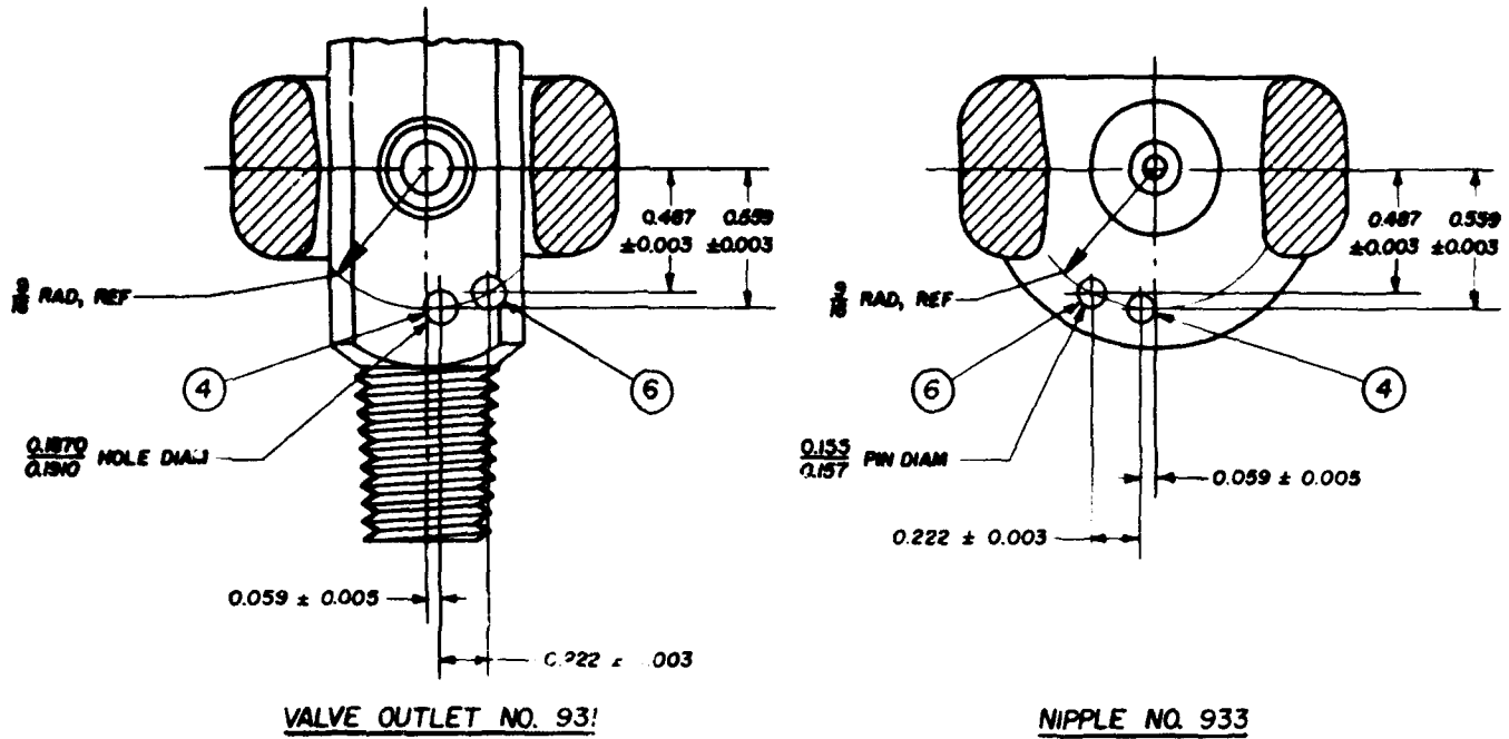
FIGURE IX.33.—No. 930 standard valve outlet connection, yoke type, for helium, medical; and helium-oxygen mixture ( O_2 less than 20 percent), medical.
