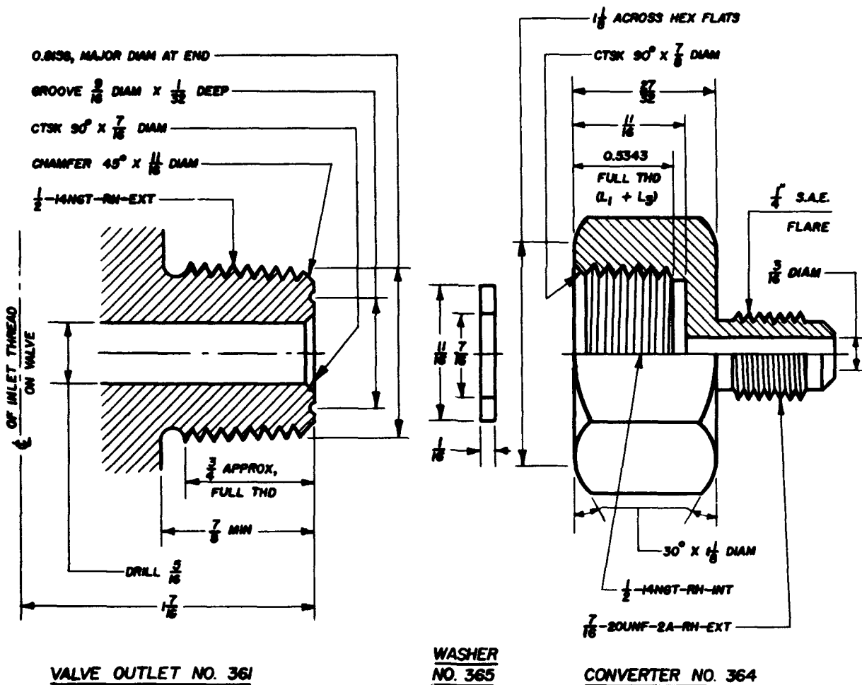
CONNECTION NO. 360
