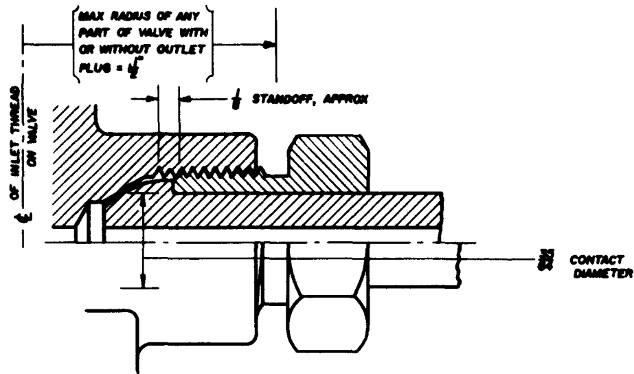
CONNECTION NO. 580
