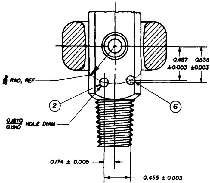
VALVE OUTLET NO. 881
