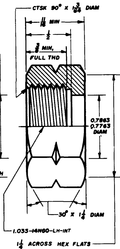
HEX NUT NO. 674
