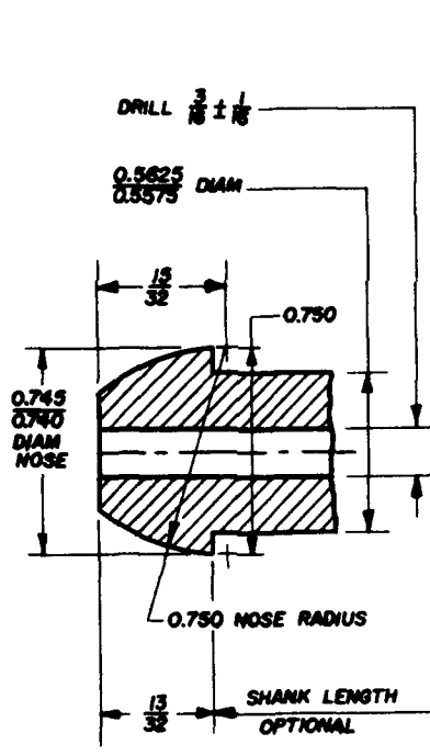
CONNECTION NO. 510
