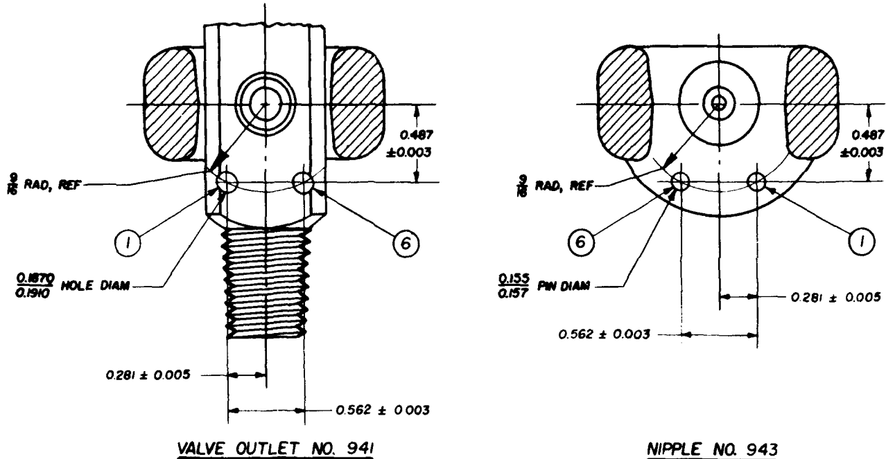
FIGURE IX.34.—No. 940 standard valve outlet connection, yoke type, for carbon dioxide, medical; and carbon dioxide-oxygen mixture ( CO_2 over 7 percent), medical.
