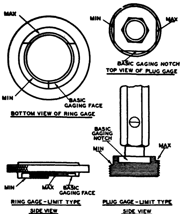
FIGURE VII.6.—Alternative form of taper pipe thread limit plug and thread ring gages.
