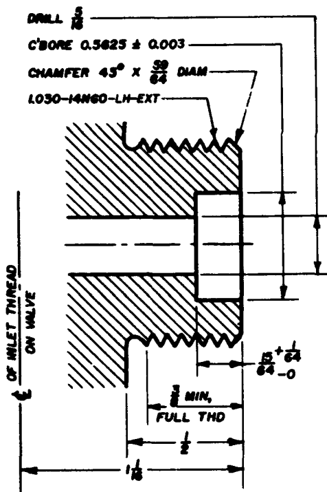
VALVE OUTLET NO. 671
