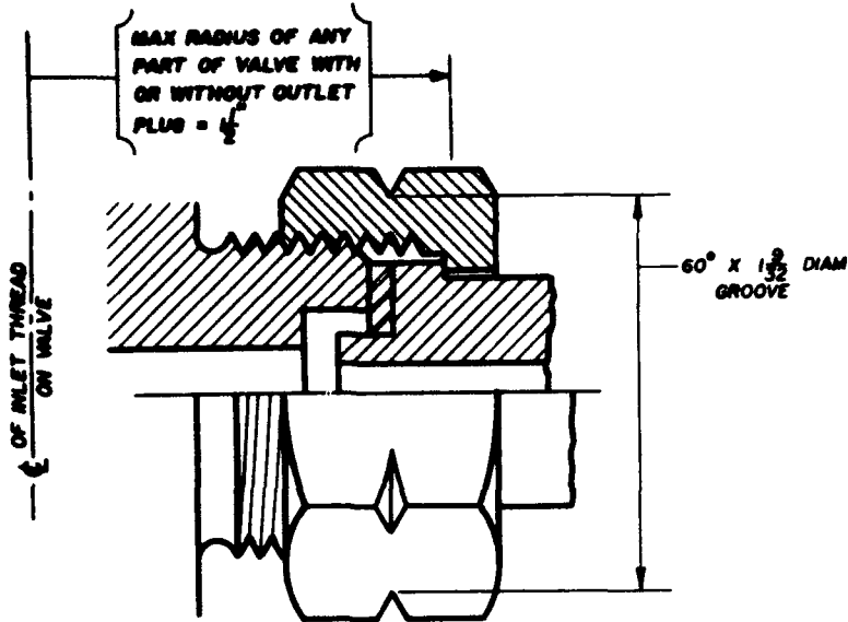
CONNECTION NO. 670
