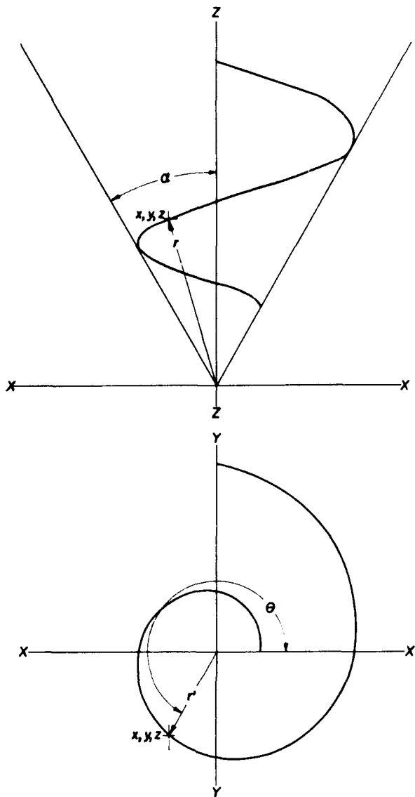
FIGURE 8.2.—The conical helix.
