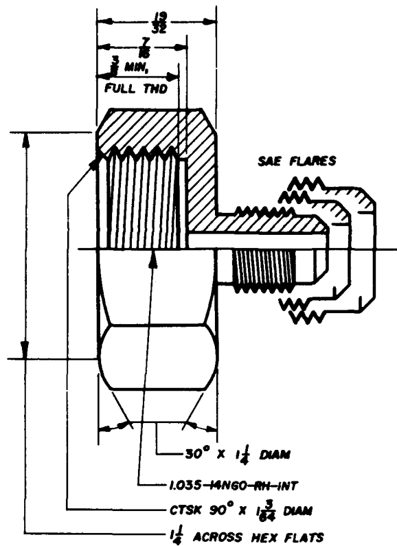
CONVERTER NO. 624
