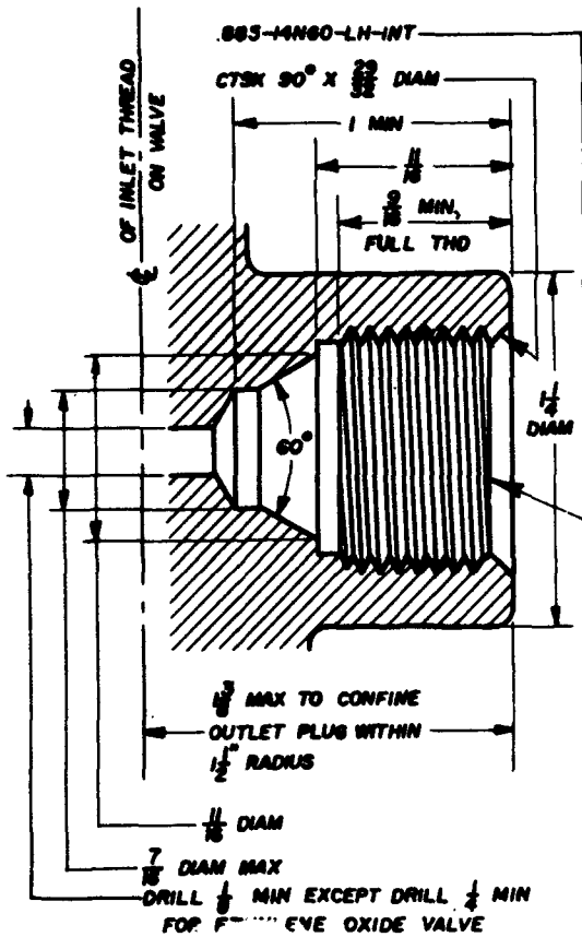
VALVE NO. 511
