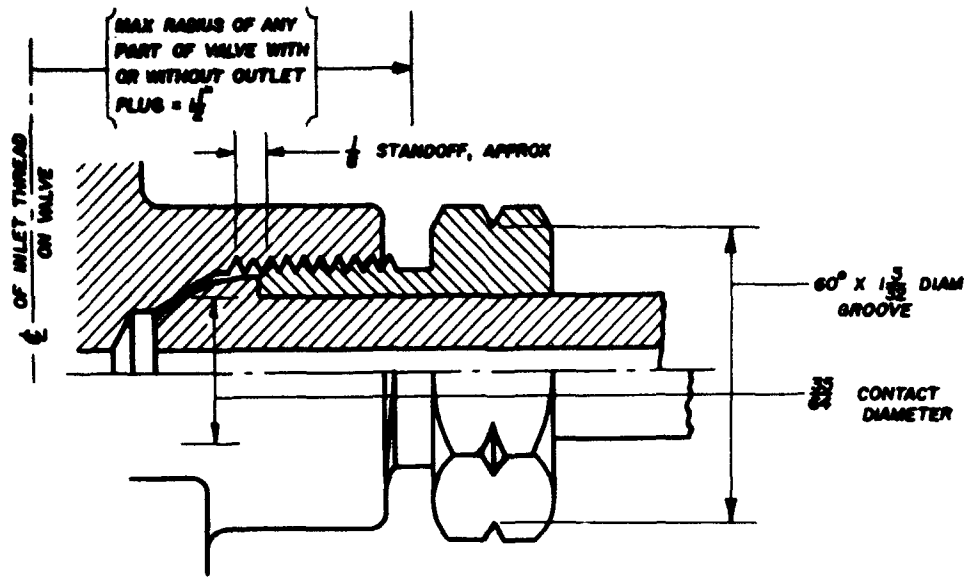
CONNECTION NO. 510
