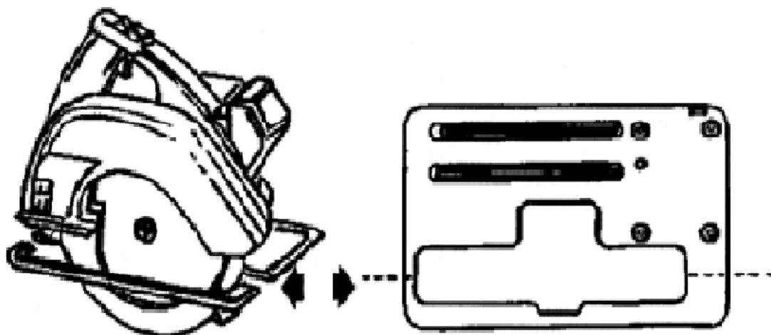
Figure 3. Builder's circular saw. Cut the foot assembly of the 10 1/4" circular saw as shown. File or grind the cut edges of the foot assembly to remove sharp edges. This size saw is necessary on Mosler or Diebold-Mosler Class 5 security files. A 7 1/4" builders circular saw is adequate for other files and does not require the modification shown above.
