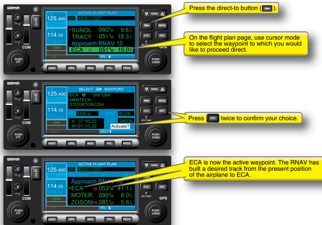
Figure 3-23. Direct-to operation.
