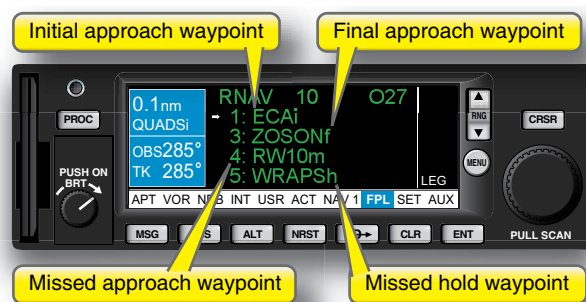
Figure 3-50. Approach waypoints.
