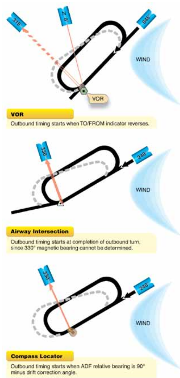
Figure 10-7. Holding—Outbound Timing.
