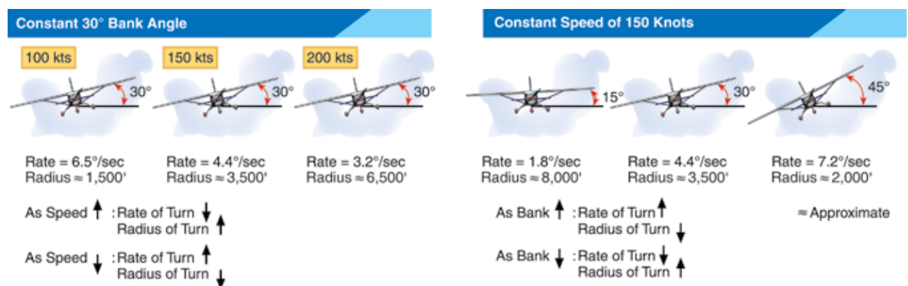
Figure 2-14. Turns.
