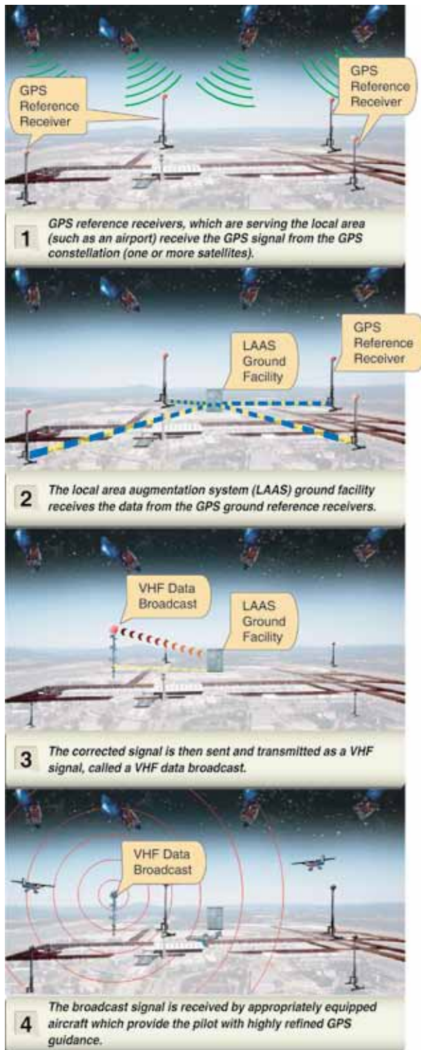
Figure 7-32. LAAS Representation.
