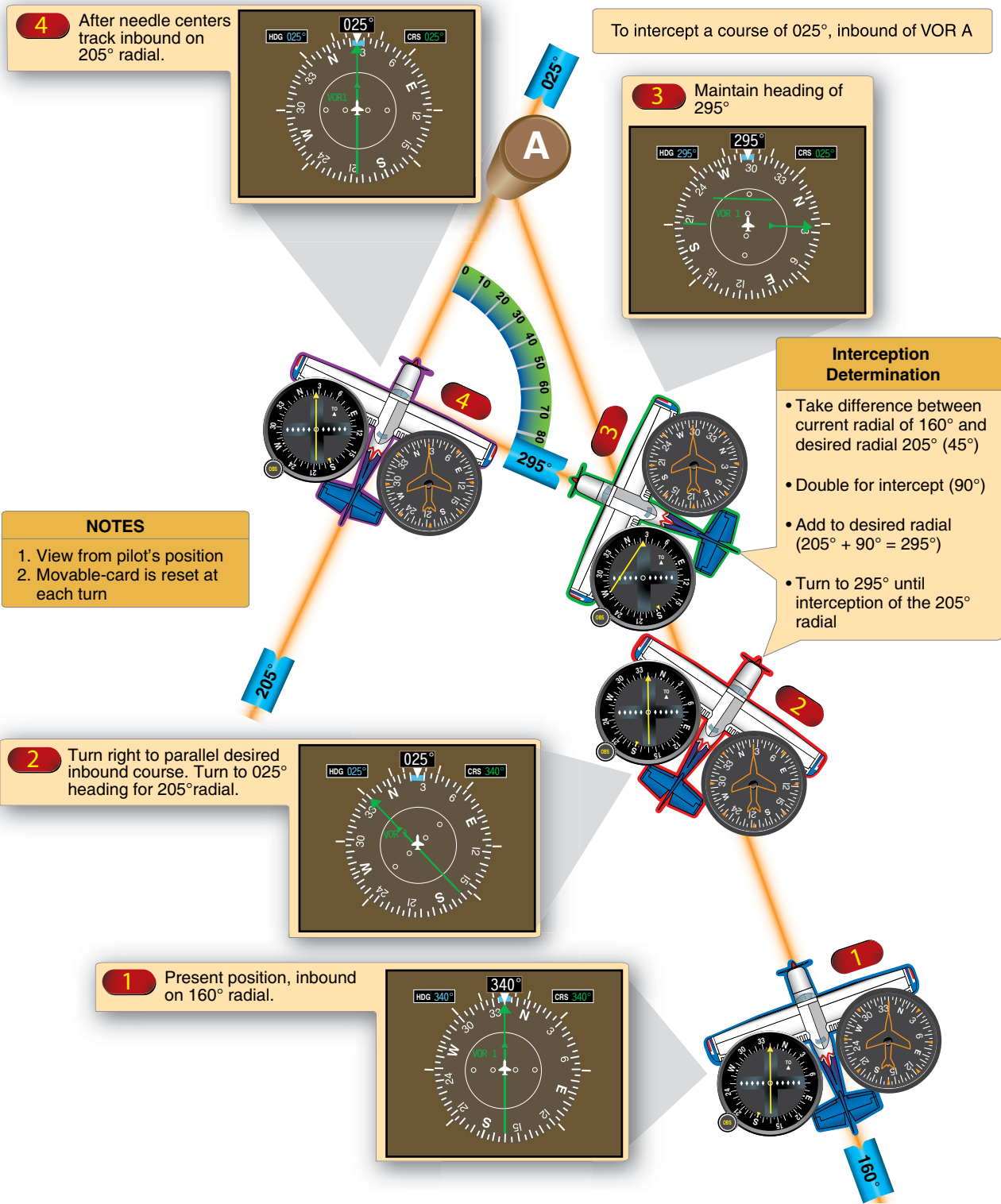
Figure 7-16. Course Interception (VOR).
