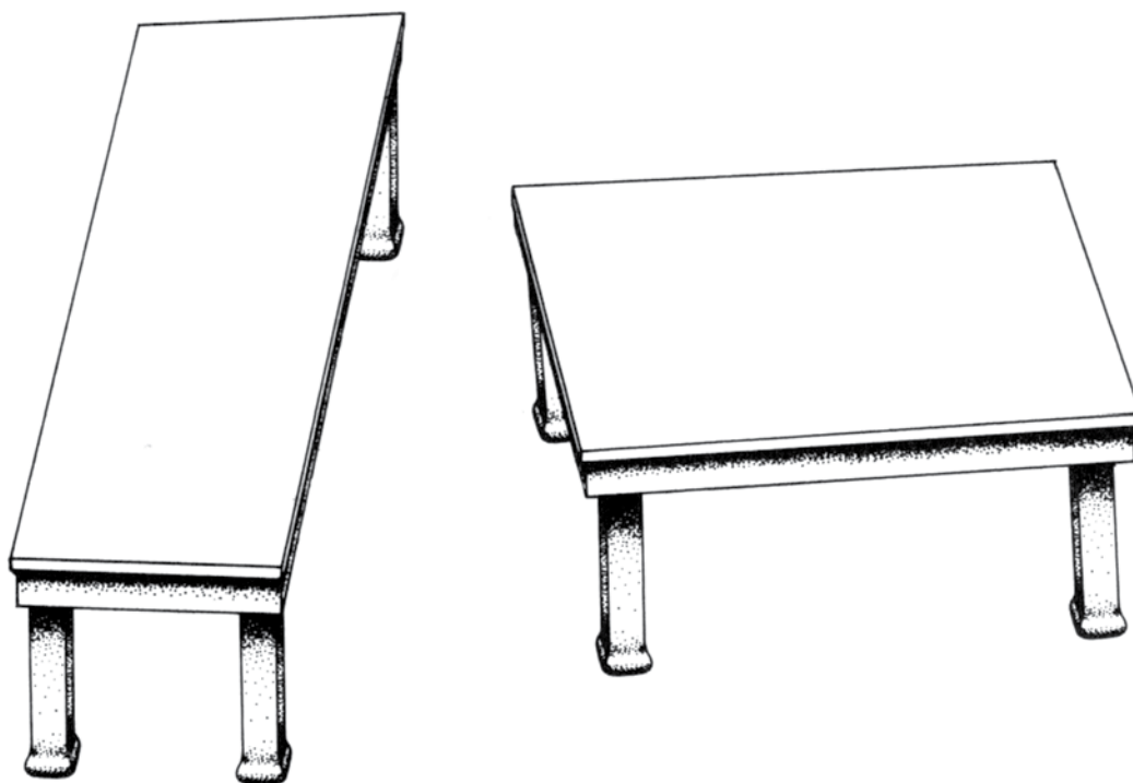
Figure 1-2. Shepard's Tables.
