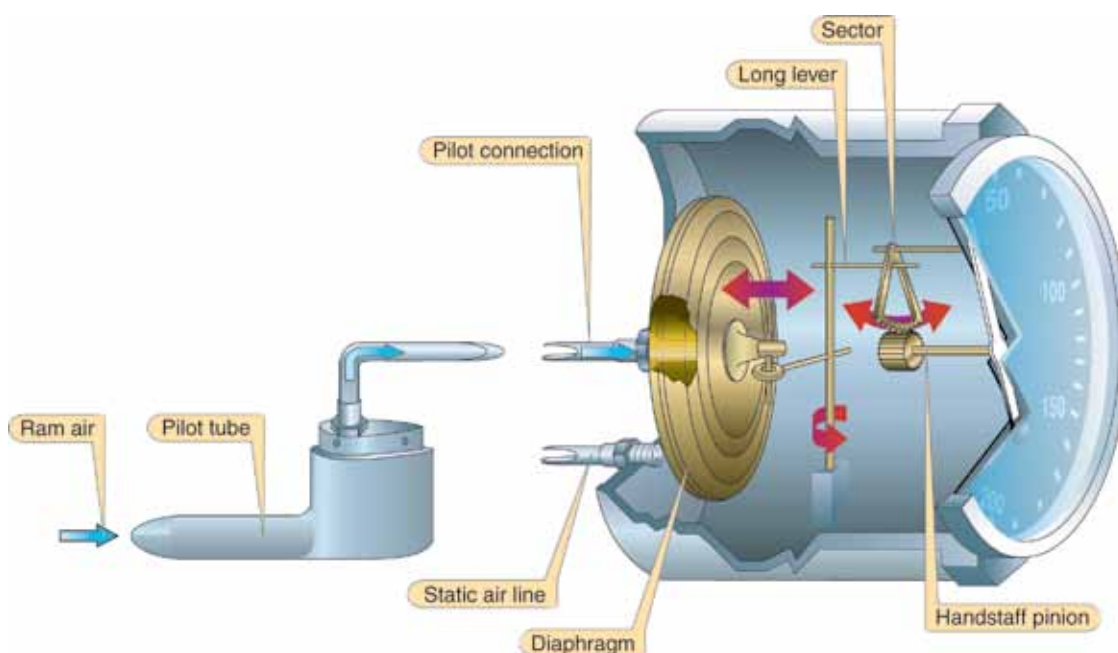
Figure 3-11. Mechanism of an Airspeed Indicator.
