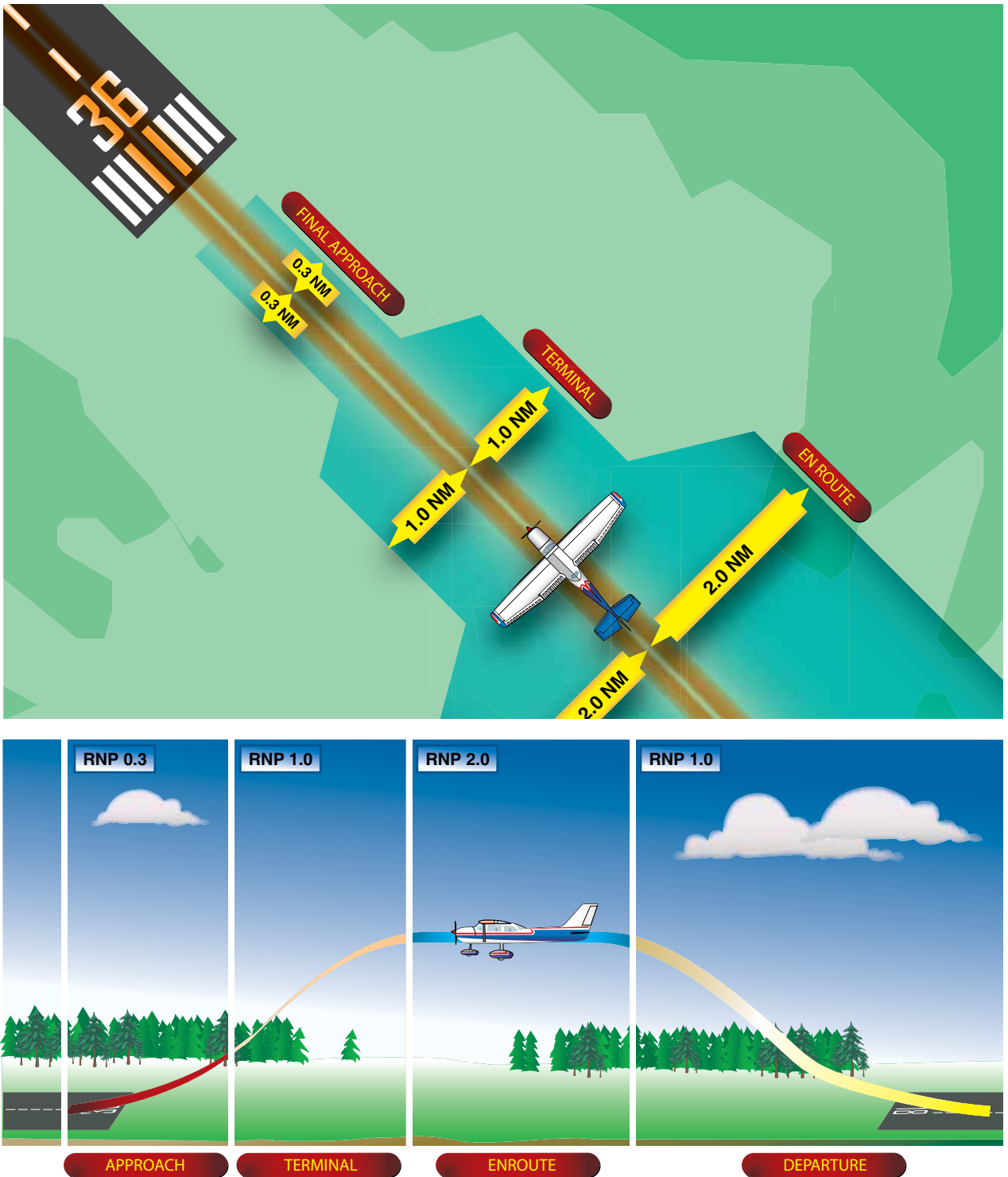
Figure 7-42. Required Navigation Performance.
